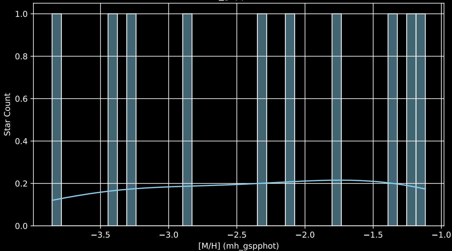
Gaia Stream: [C-23 [M/H] (mh_gspphot) (n= 10)
