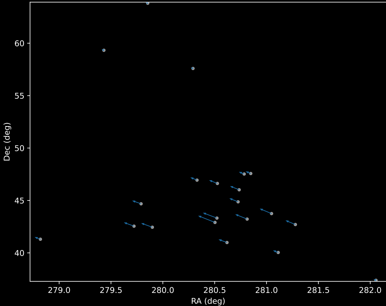
Gaia DR3 Cluster 20 Proper Motion Vectors (n=21)
