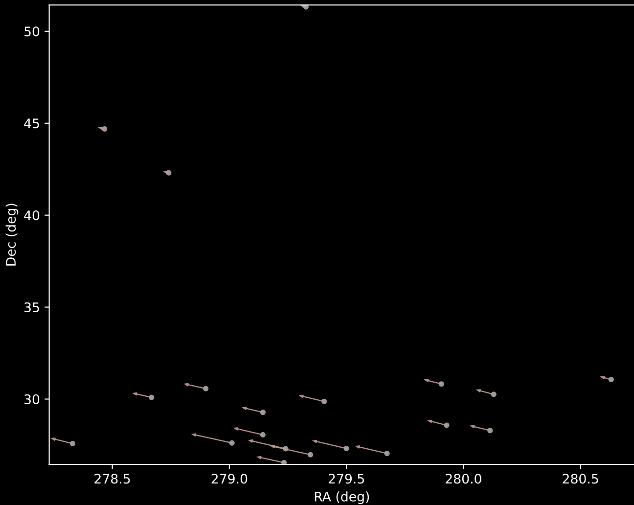
Gaia DR3 Cluster 11 Proper Motion Vectors (n=20)
