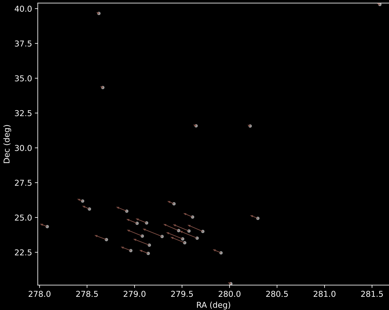
Gaia DR3 Cluster 10 Proper Motion Vectors (n=28)
