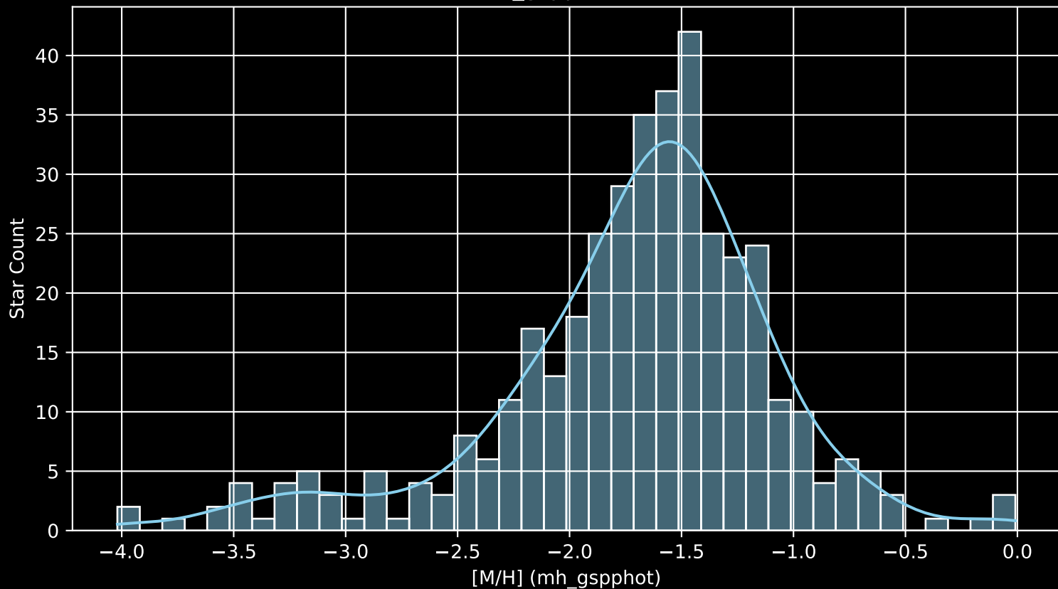
Gaia Stream: [Hrid [M/H] (mh_gspphot) (n= 393)
