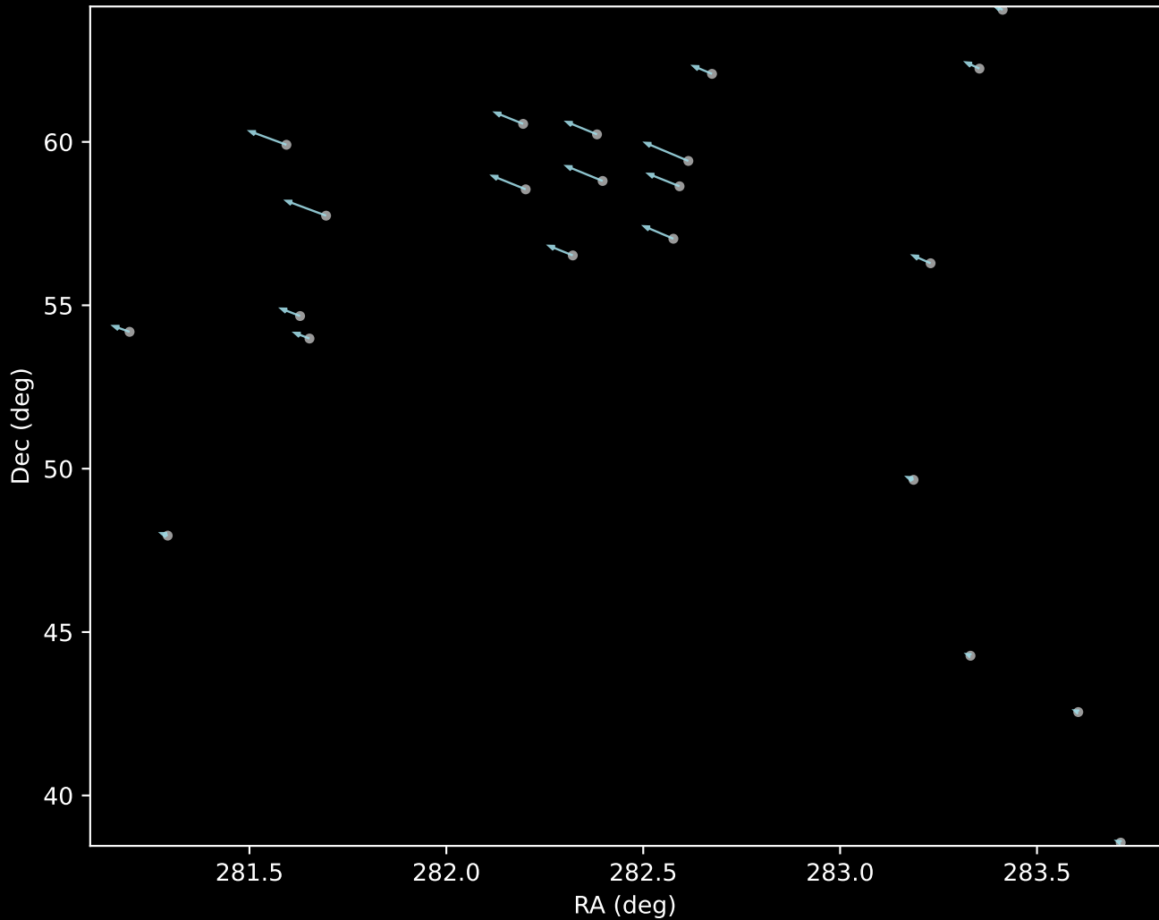
Gaia DR3 Cluster 19 Proper Motion Vectors (n=22)
