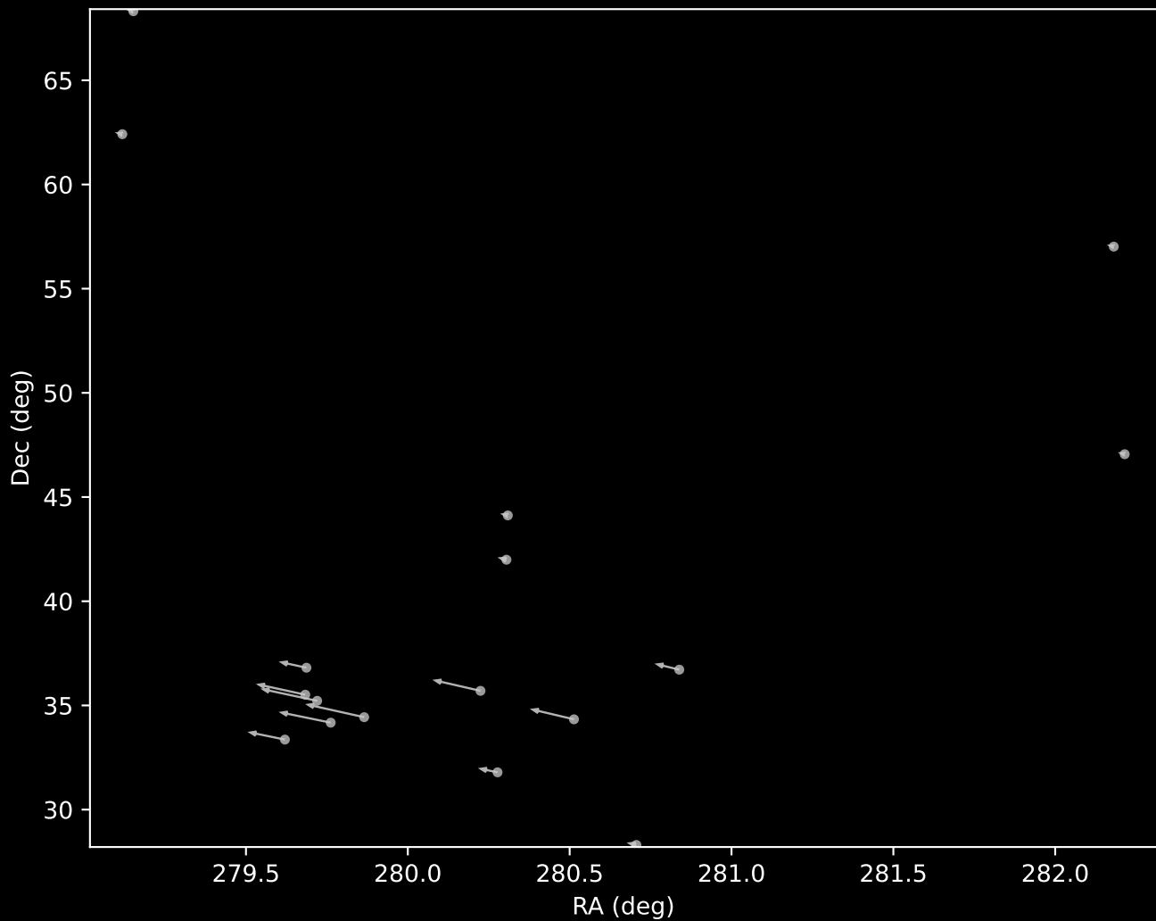
Gaia DR3 Cluster 15 Proper Motion Vectors (n=17)
