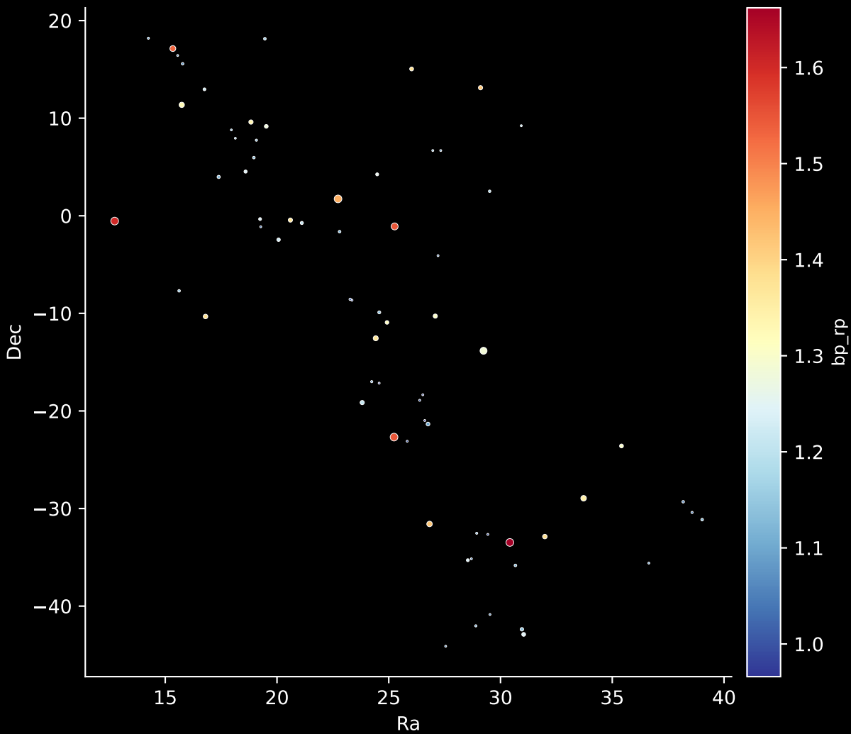
Gaia Stream: [Kwando] Stars: 69
