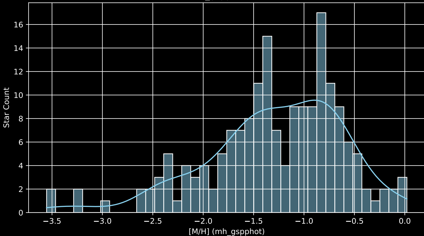
Gaia Stream: [LMS-1 [M/H] (mh_gspphot) (n= 180)
