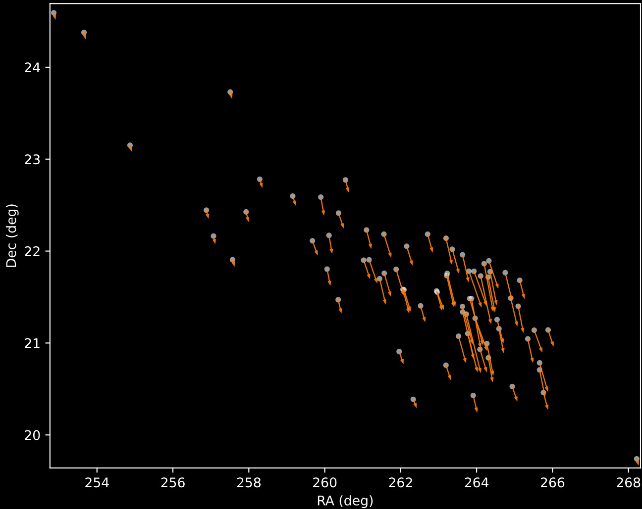
Gaia DR3 Cluster 2 Proper Motion Vectors (n=72)
