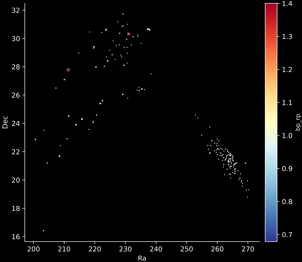
Gaia Stream: [LMS-1] Stars: 180
