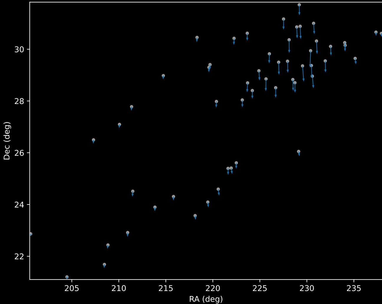
Gaia DR3 Cluster 0 Proper Motion Vectors (n=54)
