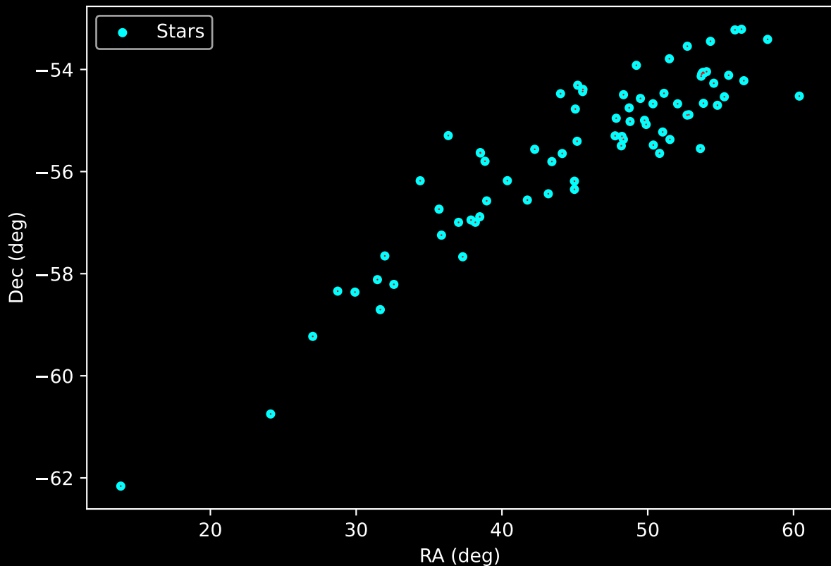
Gaia Stream: [NGC1261] Proper Motion Vectors for Gaia Star Field (n= 77)
