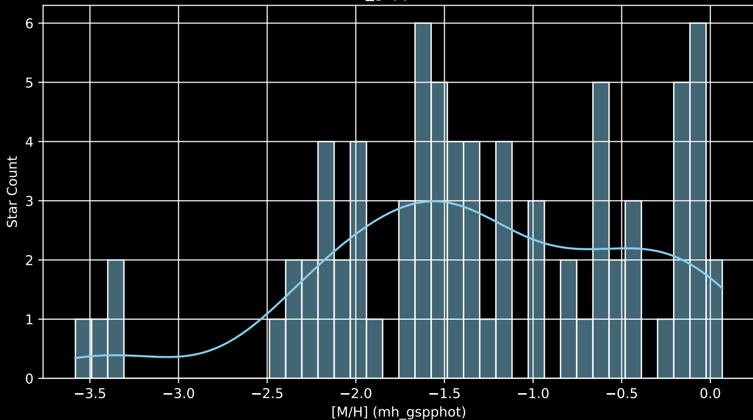
Gaia Stream: [NGC1261 [M/H] (mh_gspphot) (n= 77)
