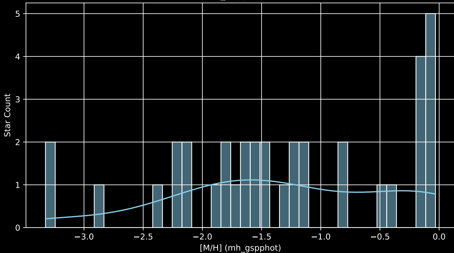
Gaia Stream: [NGC1261b [M/H] (mh_gspphot) (n= 36)
