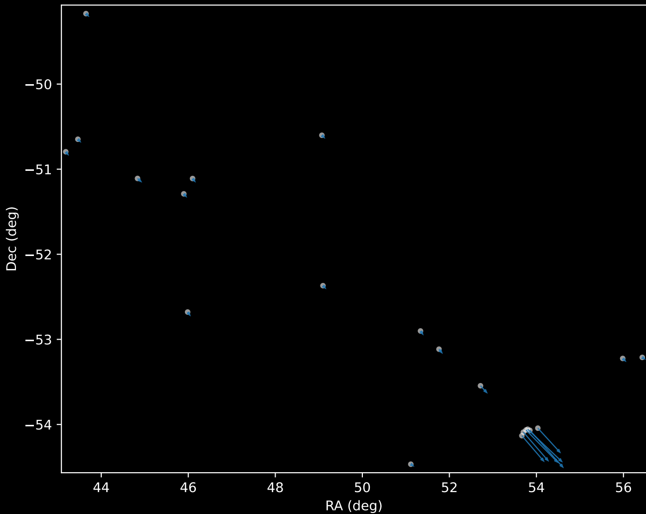
Gaia DR3 Cluster 0 Proper Motion Vectors (n=21)
