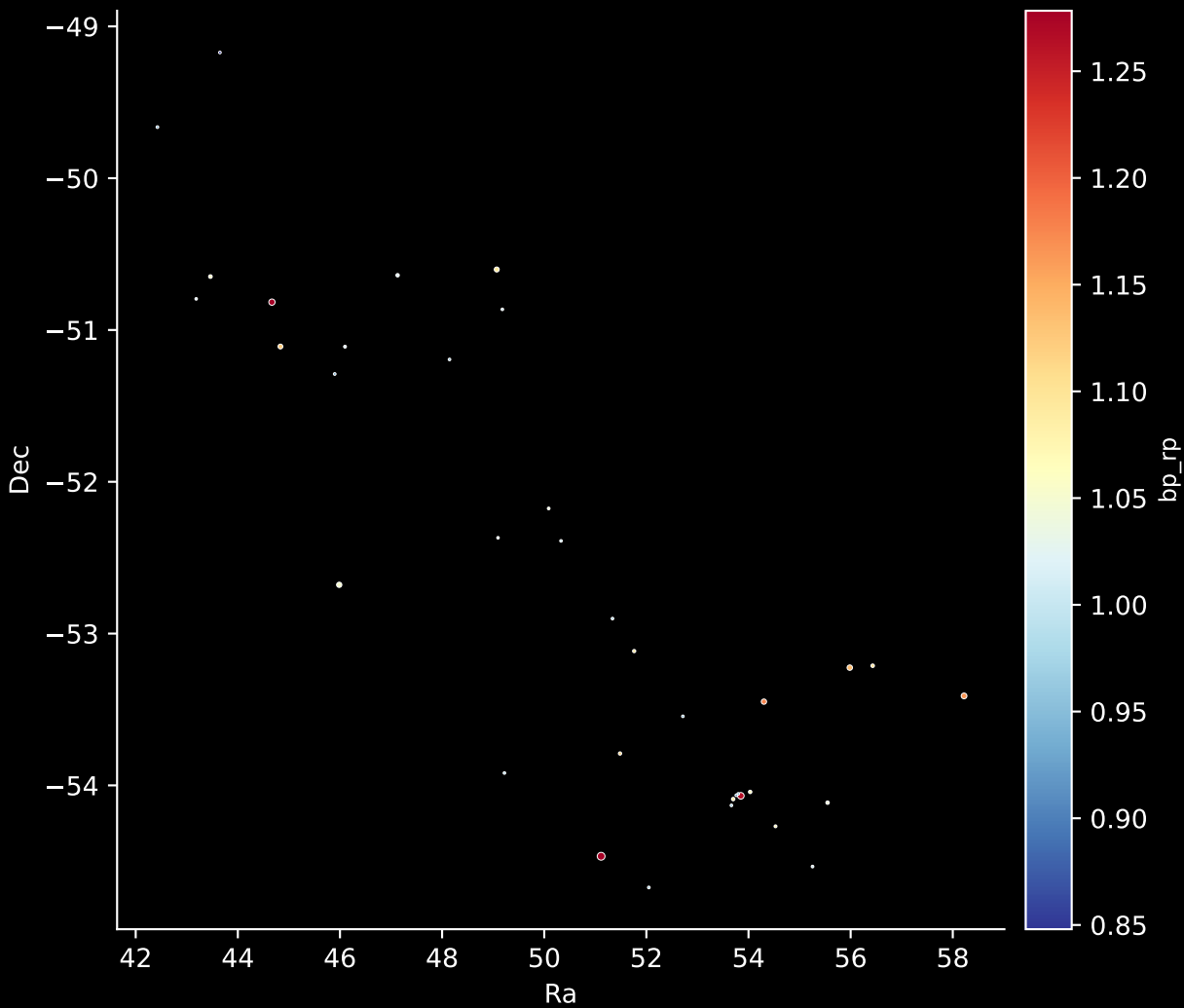
Gaia Stream: [NGC1261b] Stars: 36
