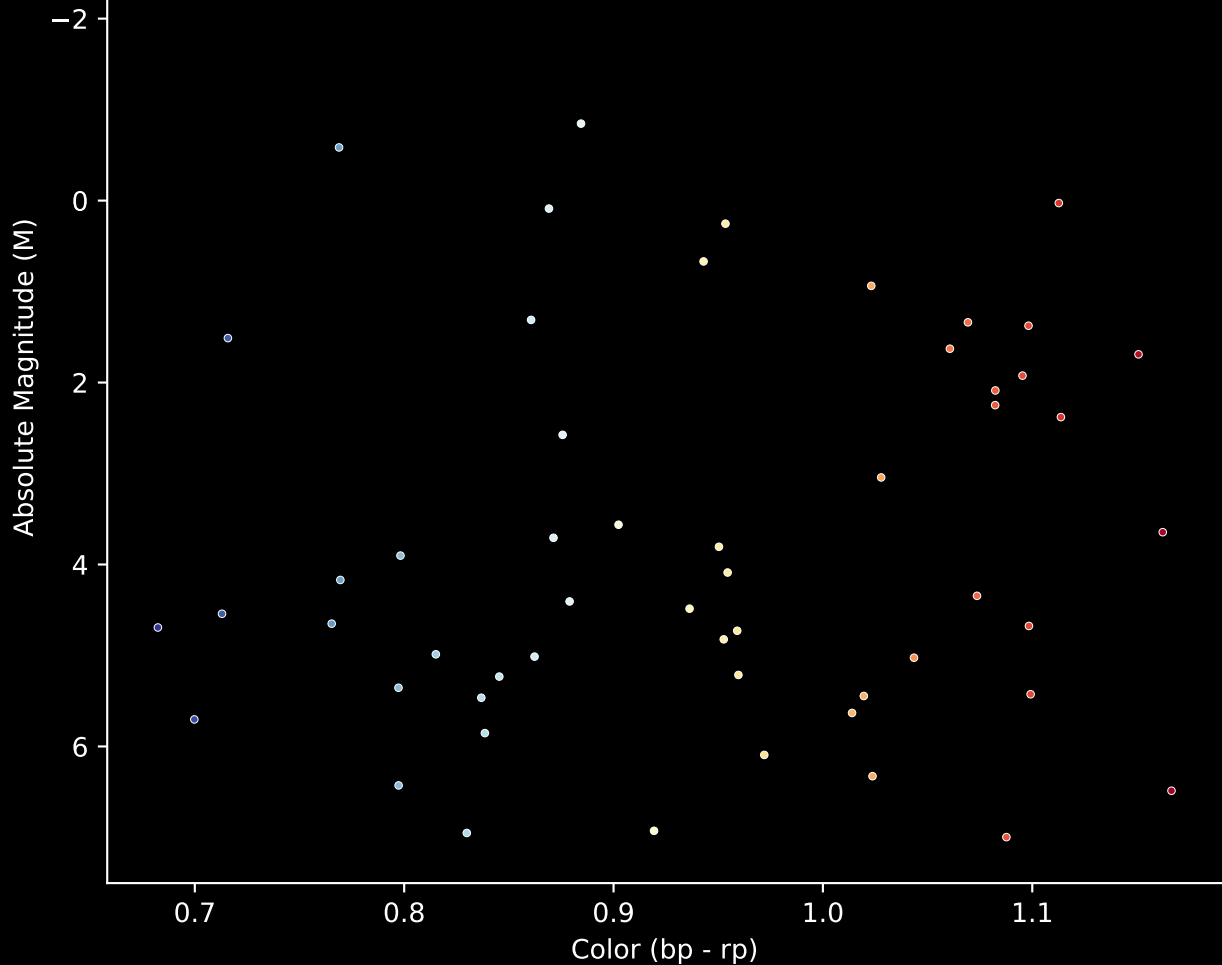
Gaia Stream: [NGC2298] Stream (n= 56) Hertzprung-Russel Diagram
