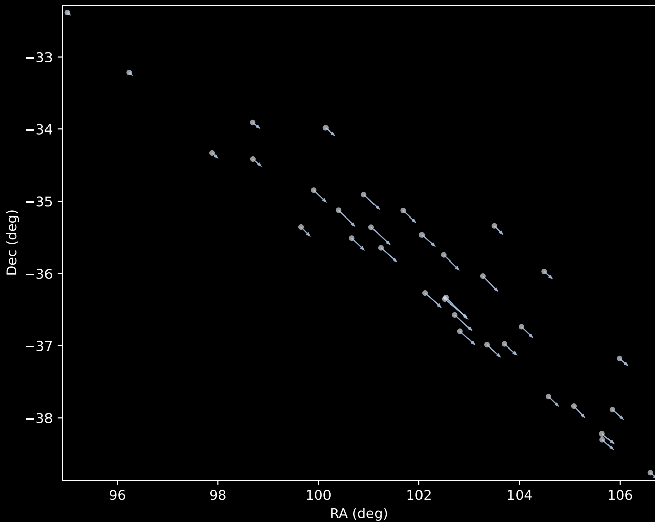
Gaia DR3 Cluster 1 Proper Motion Vectors (n=34)
