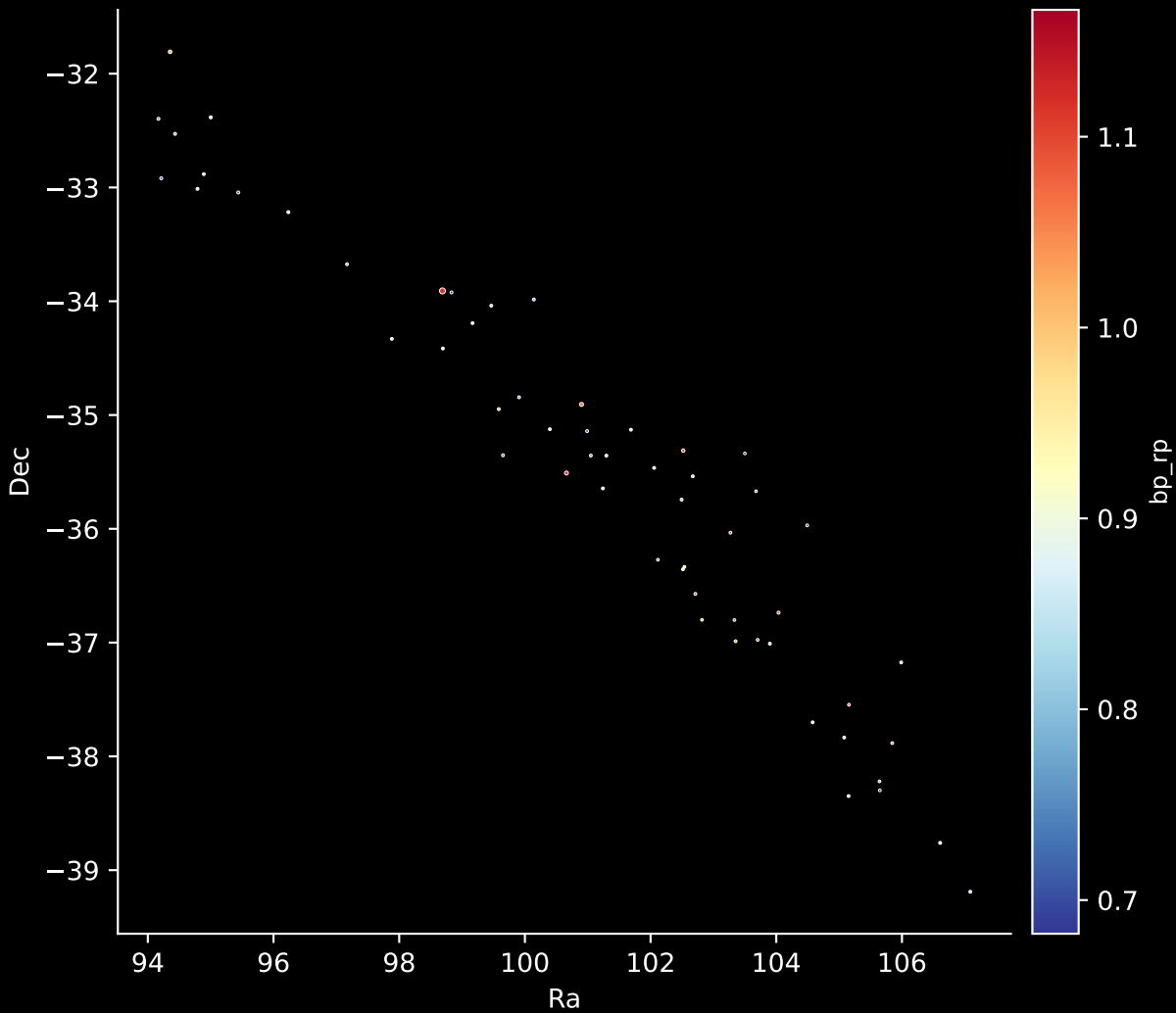
Gaia Stream: [NGC2298] Stars: 56
