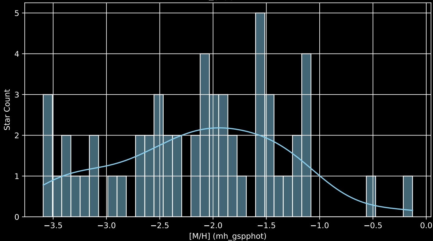
Gaia Stream: [NGC2298 [M/H] (mh_gspphot) (n= 56)
