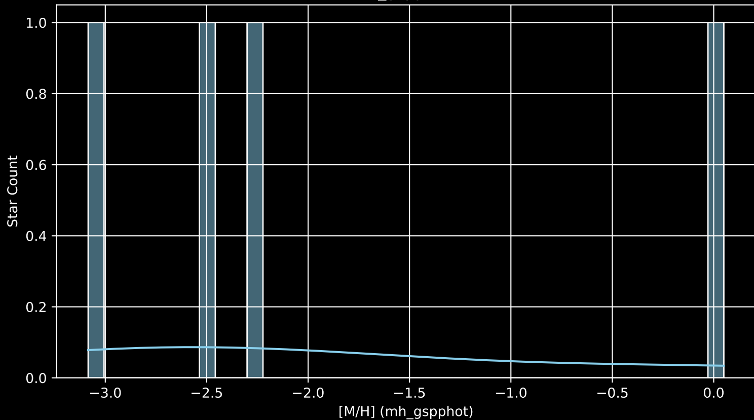
Gaia Stream: [New-1 [M/H] (mh_gspphot) (n= 4)
