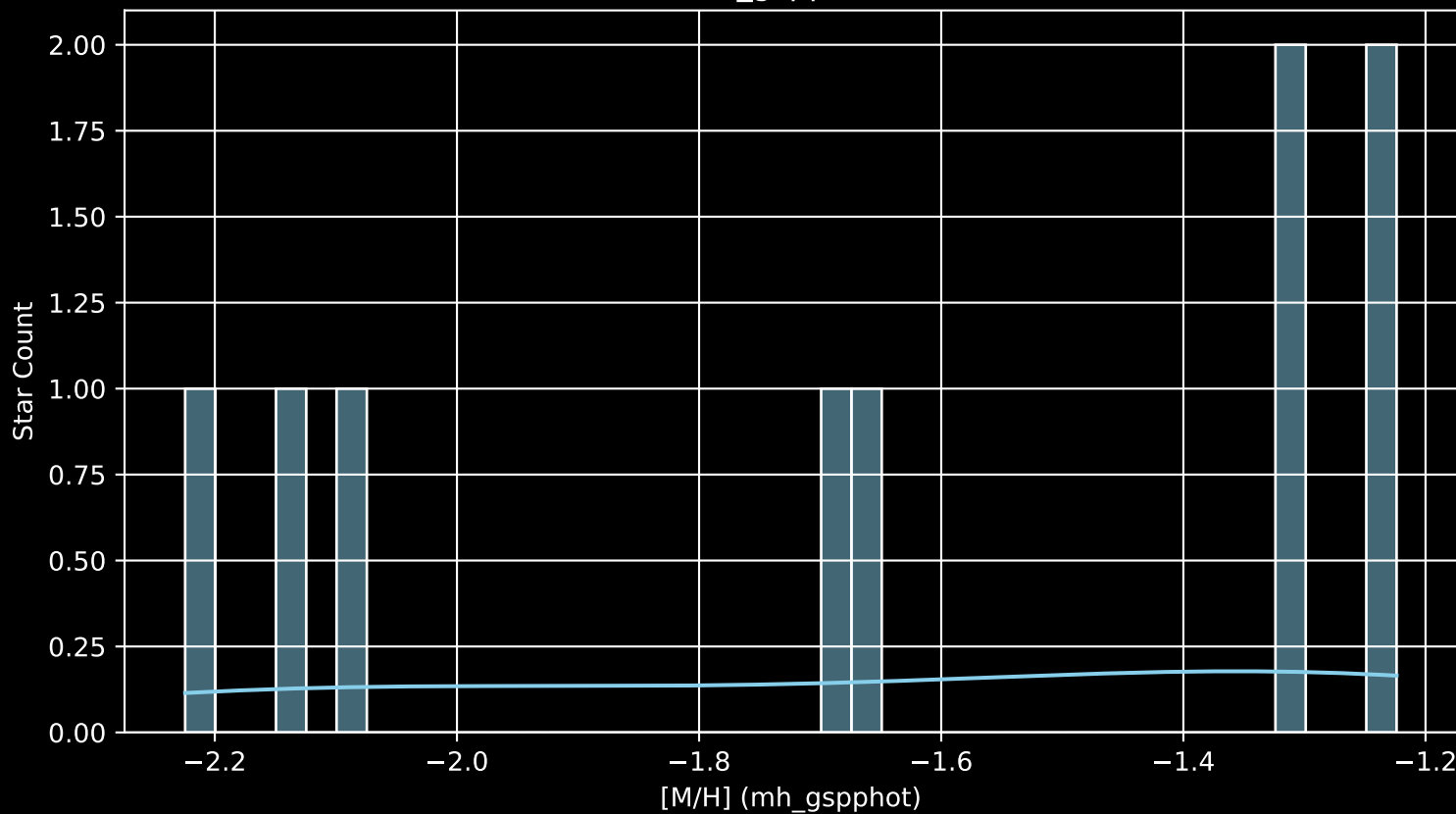
Gaia Stream: [New-11 [M/H] (mh_gspphot) (n= 9)
