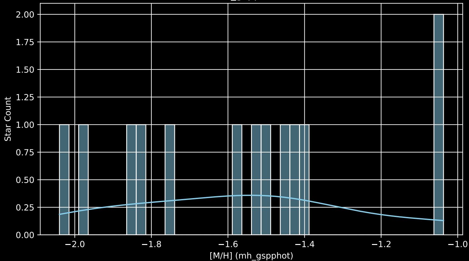
Gaia Stream: [New-14 [M/H] (mh_gspphot) (n= 13)
