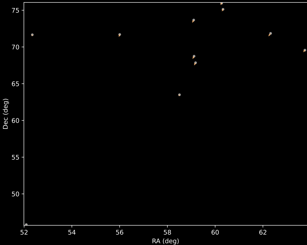
Gaia DR3 Cluster 3 Proper Motion Vectors (n=11)
