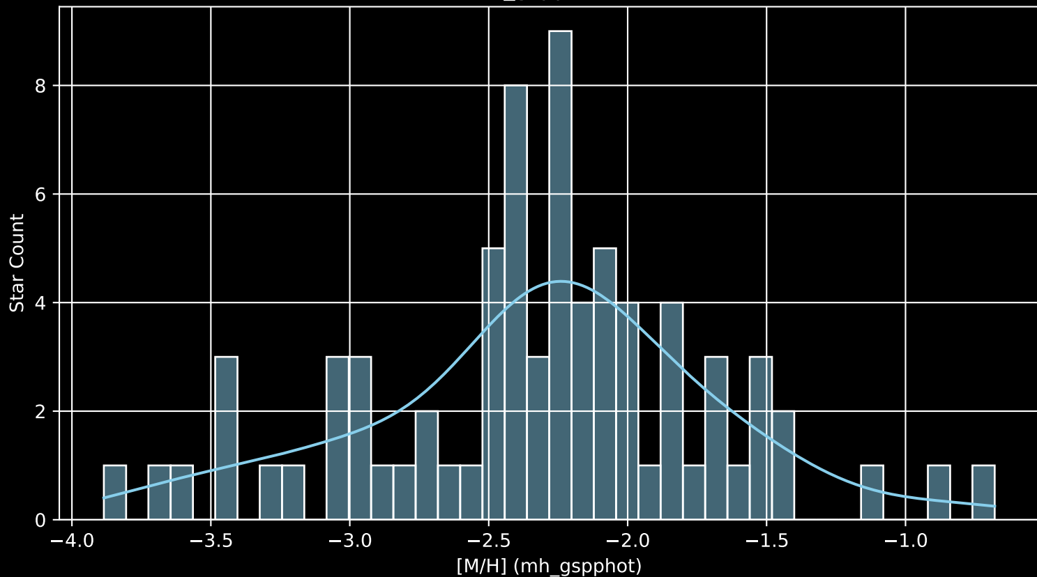
Gaia Stream: [New-6 [M/H] (mh_gspphot) (n= 76)
