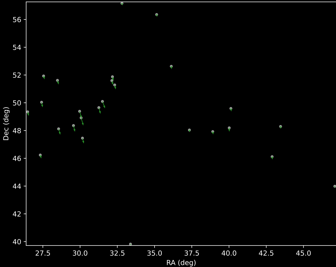
Gaia DR3 Cluster 4 Proper Motion Vectors (n=26)
