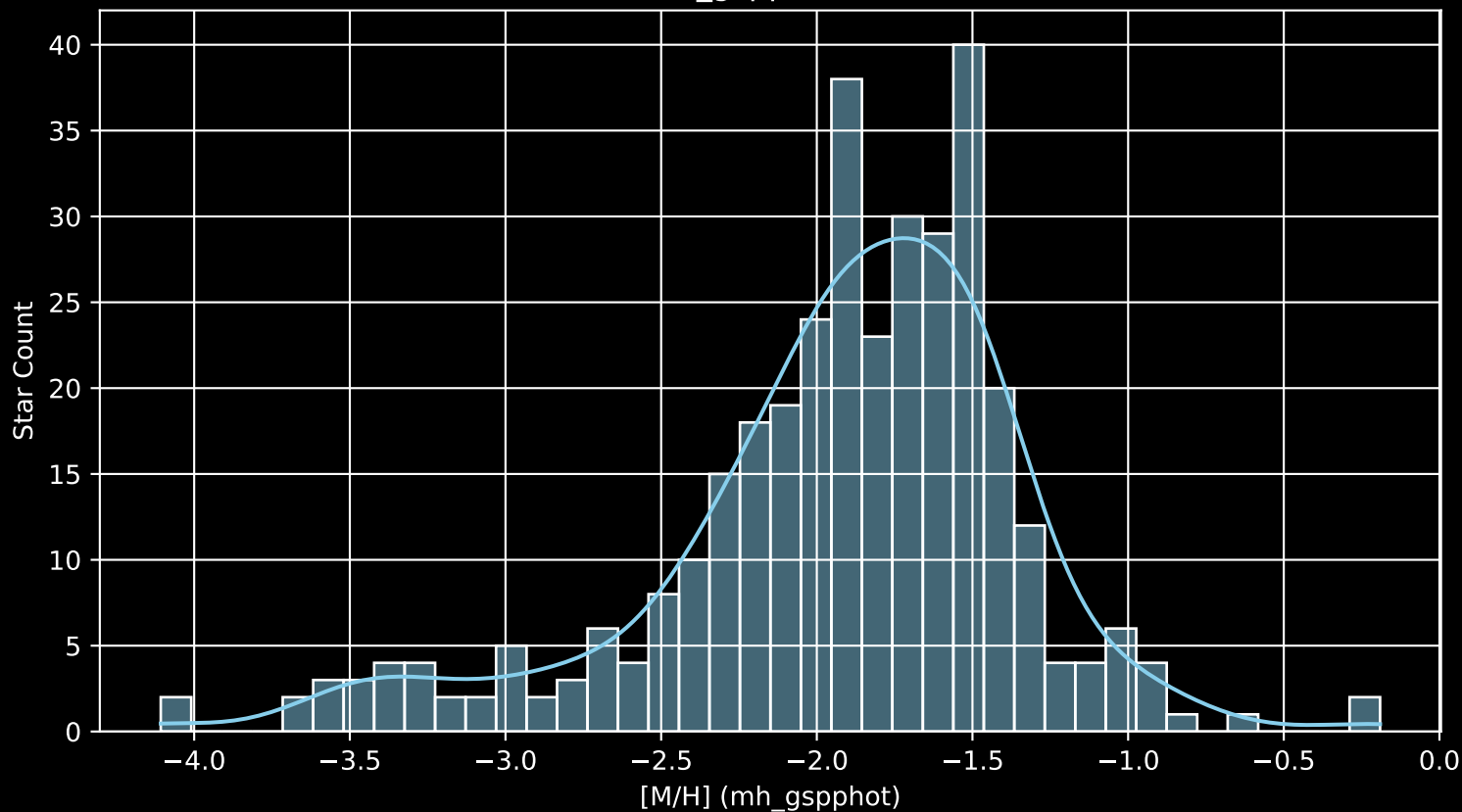
Gaia Stream: [Phlegethon [M/H] (mh_gspphot) (n= 350)
