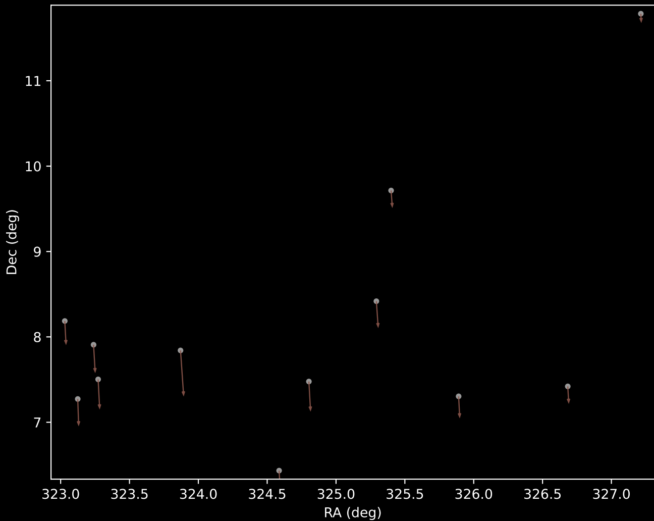
Gaia DR3 Cluster 10 Proper Motion Vectors (n=12)
