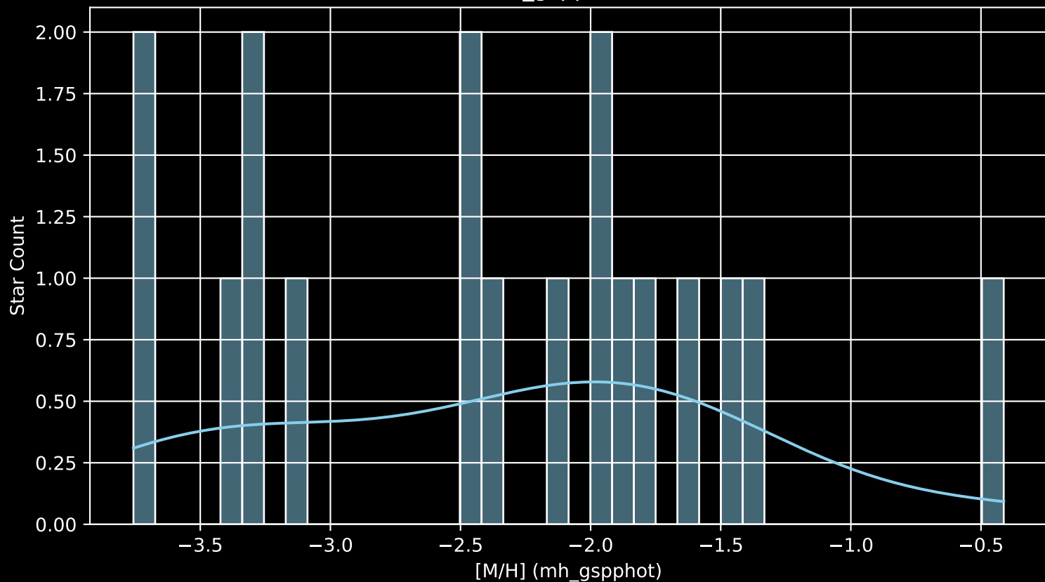
Gaia Stream: [Phoenix [M/H] (mh_gspphot) (n= 18)
