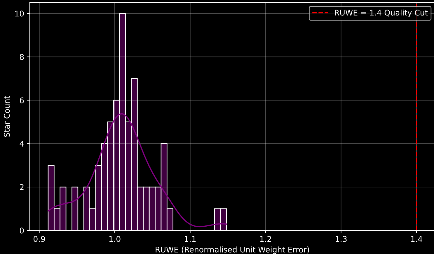
Gaia Stream: [C-10] RUWE Distribution (n= 66)
