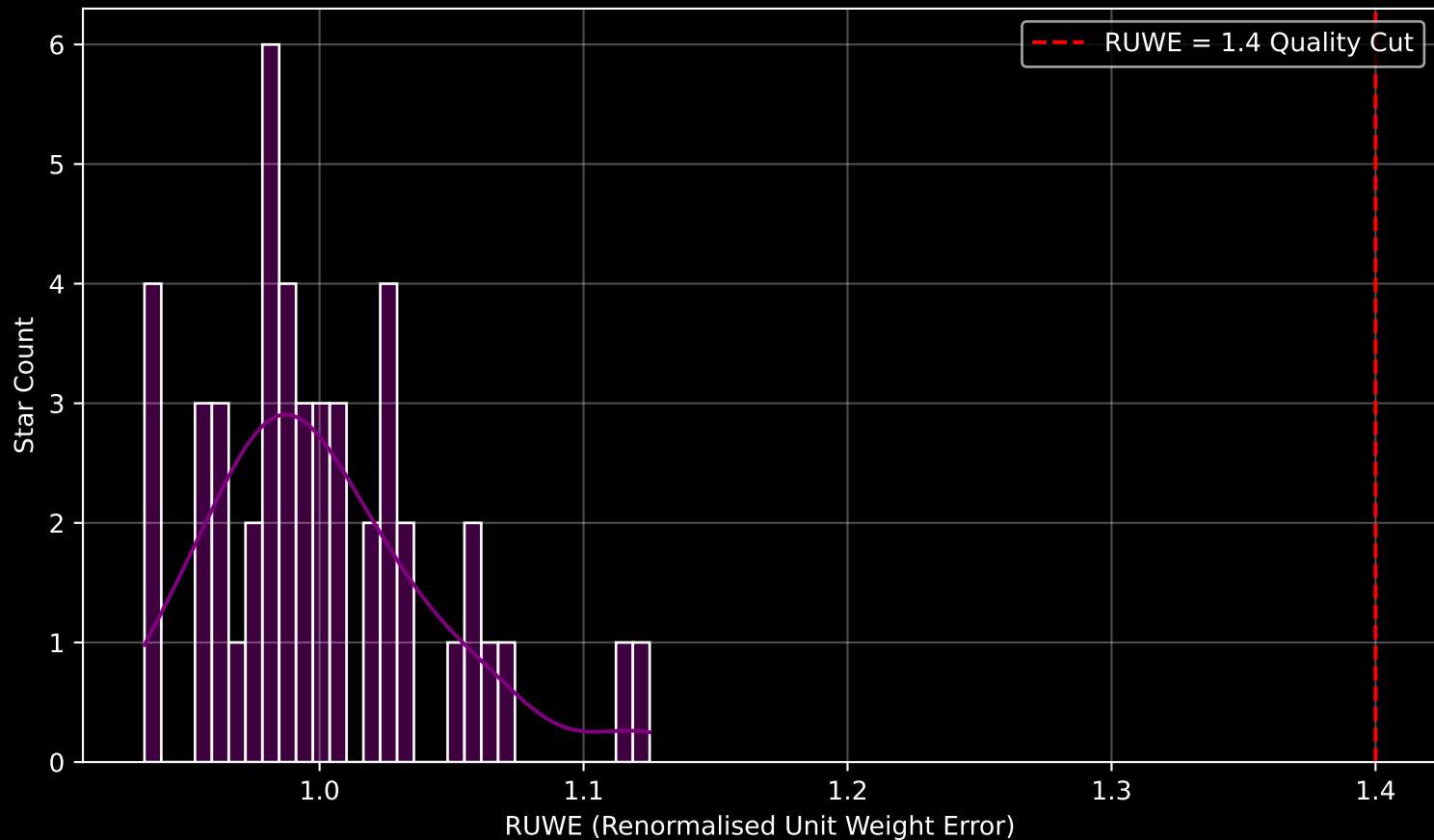
Gaia Stream: [C-11] RUWE Distribution (n= 47)
