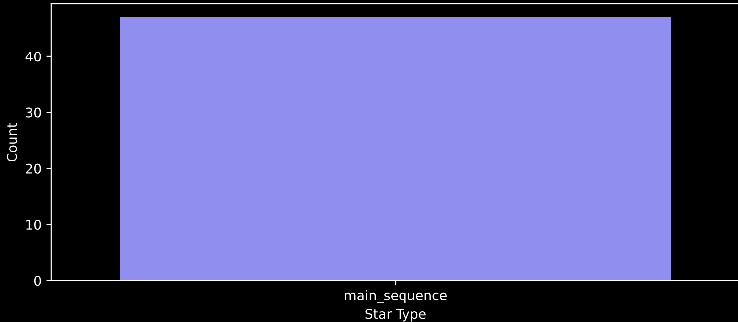
Gaia Stream: [C-11] Count plot of Star Type
