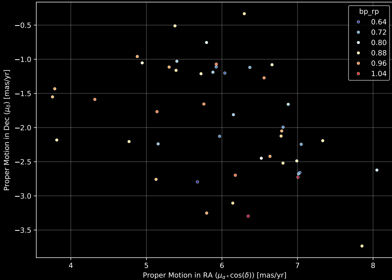
Gaia Stream: [C-11] Proper Motion Diagram (n= 47)
