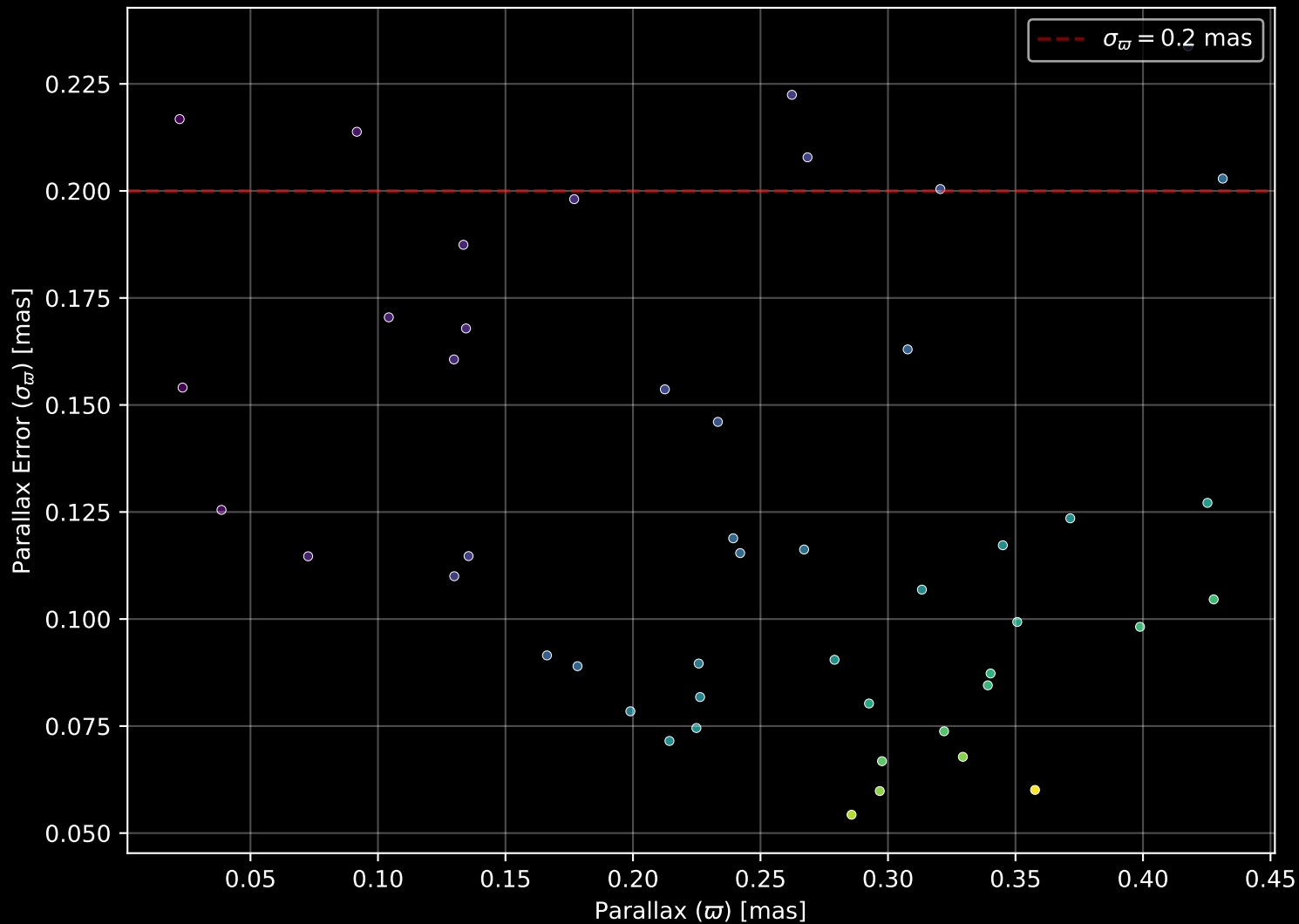
Gaia Stream: [C-11] Parallax Quality (n= 47)
