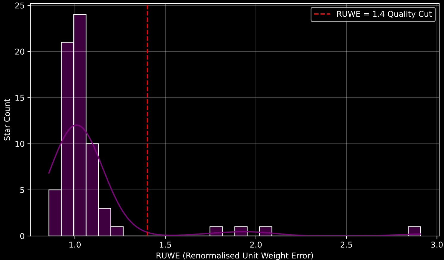
Gaia Stream: [C-13] RUWE Distribution (n= 68)
