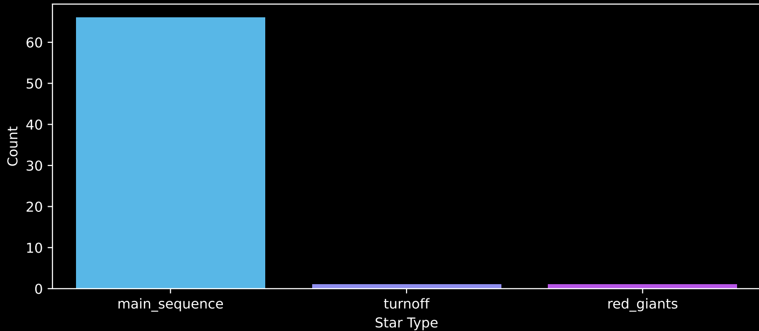
Gaia Stream: [C-13] Count plot of Star Type
