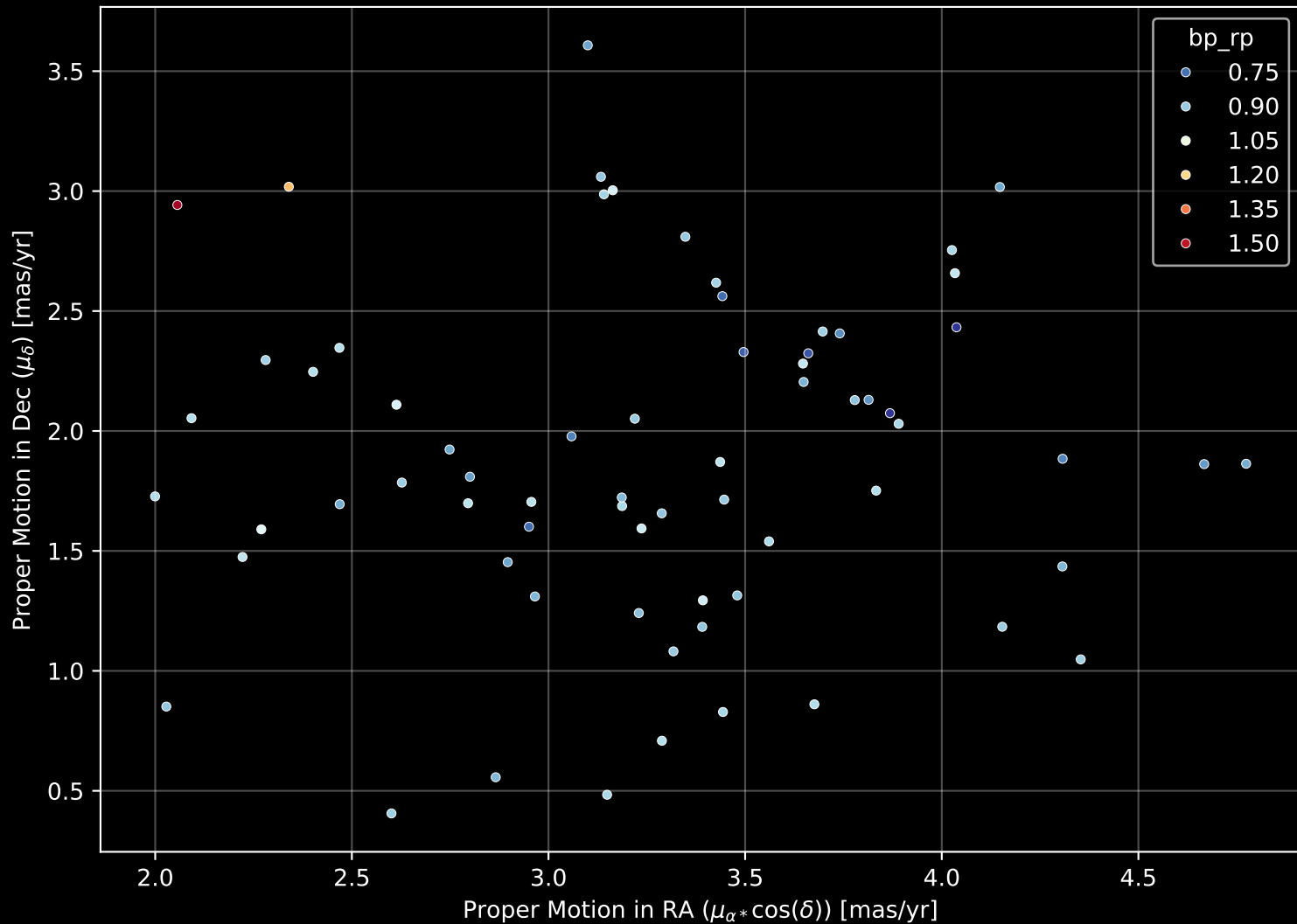
Gaia Stream: [C-13] Proper Motion Diagram (n= 68)
