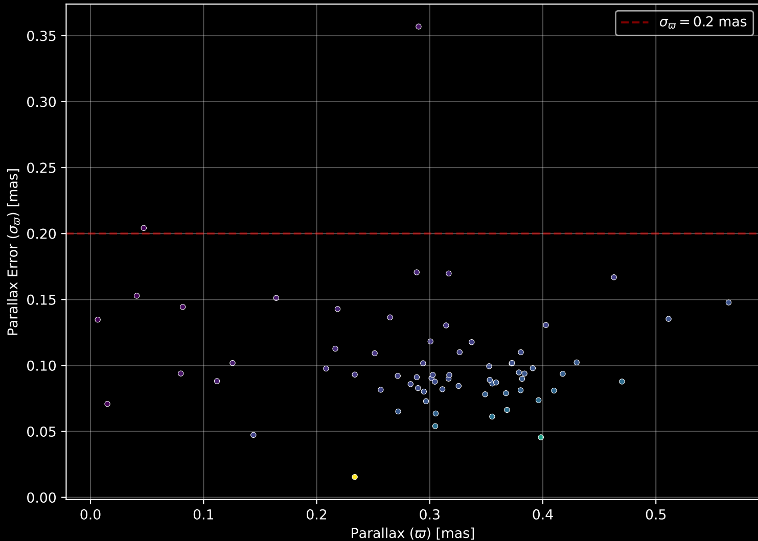
Gaia Stream: [C-13] Parallax Quality (n= 68)
