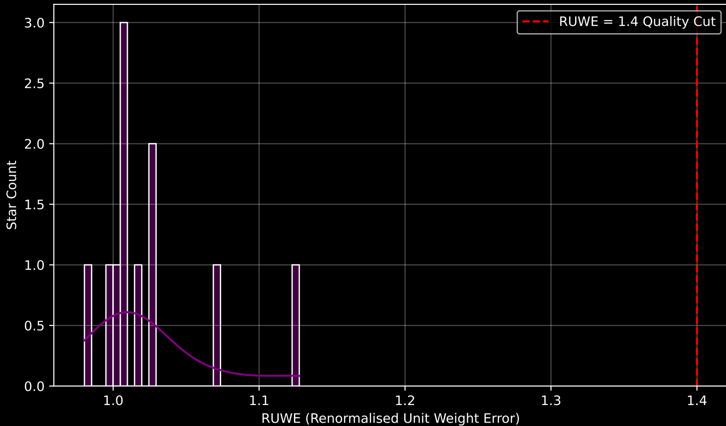
Gaia Stream: [C-19] RUWE Distribution (n= 11)
