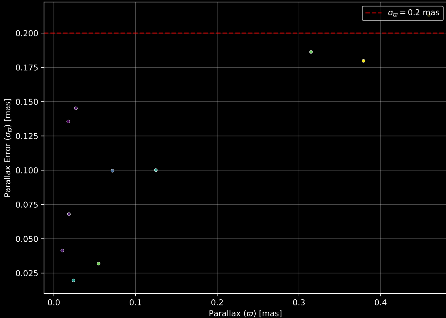
Gaia Stream: [C-19] Parallax Quality (n= 11)
