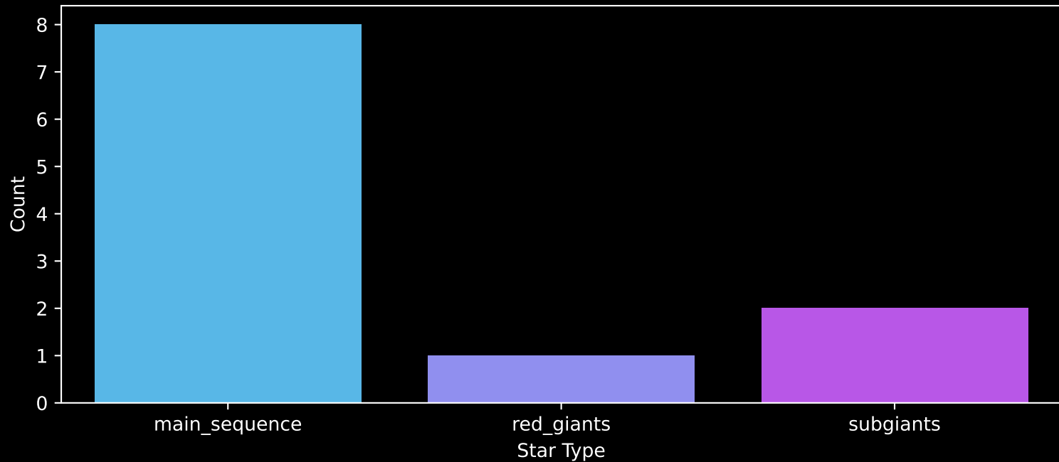
Gaia Stream: [C-19] Count plot of Star Type
