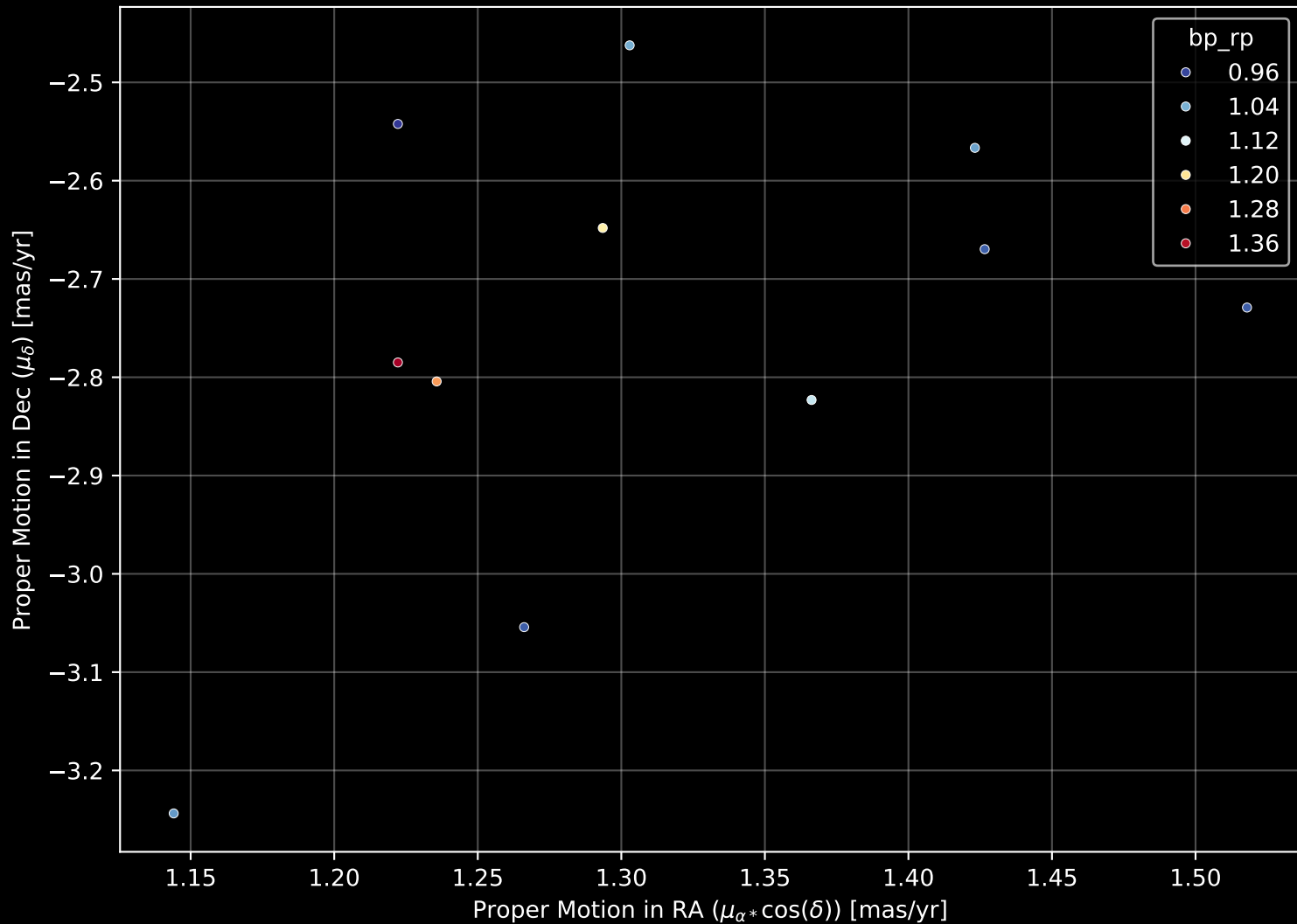
Gaia Stream: [C-19] Proper Motion Diagram (n= 11)
