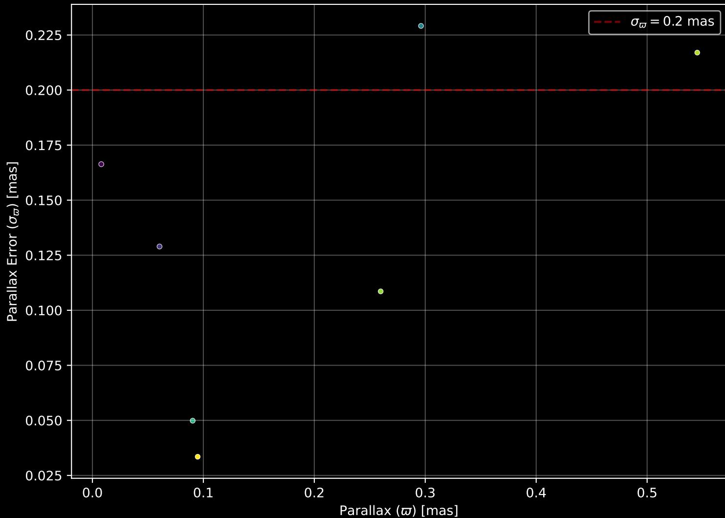
Gaia Stream: [C-20] Parallax Quality (n= 7)
