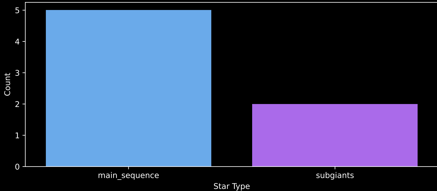
Gaia Stream: [C-20] Count plot of Star Type
