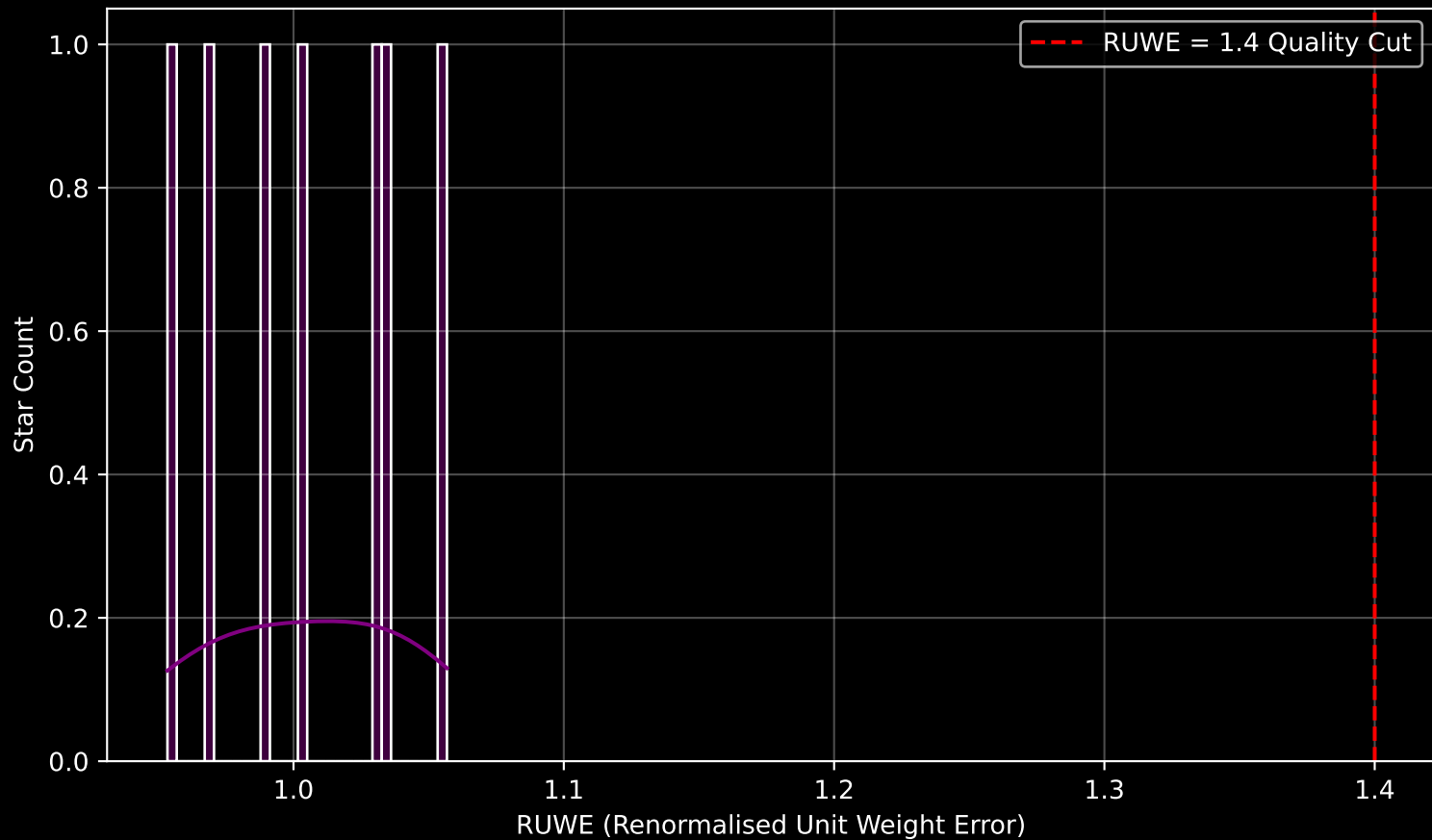
Gaia Stream: [C-20] RUWE Distribution (n= 7)
