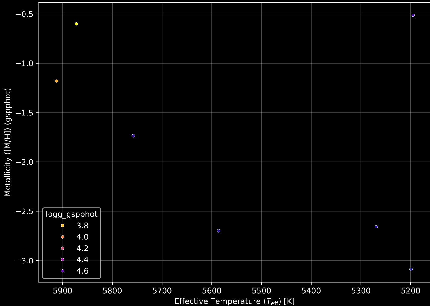
Gaia Stream: [C-20] Stellar Population Parameters (n= 7)
