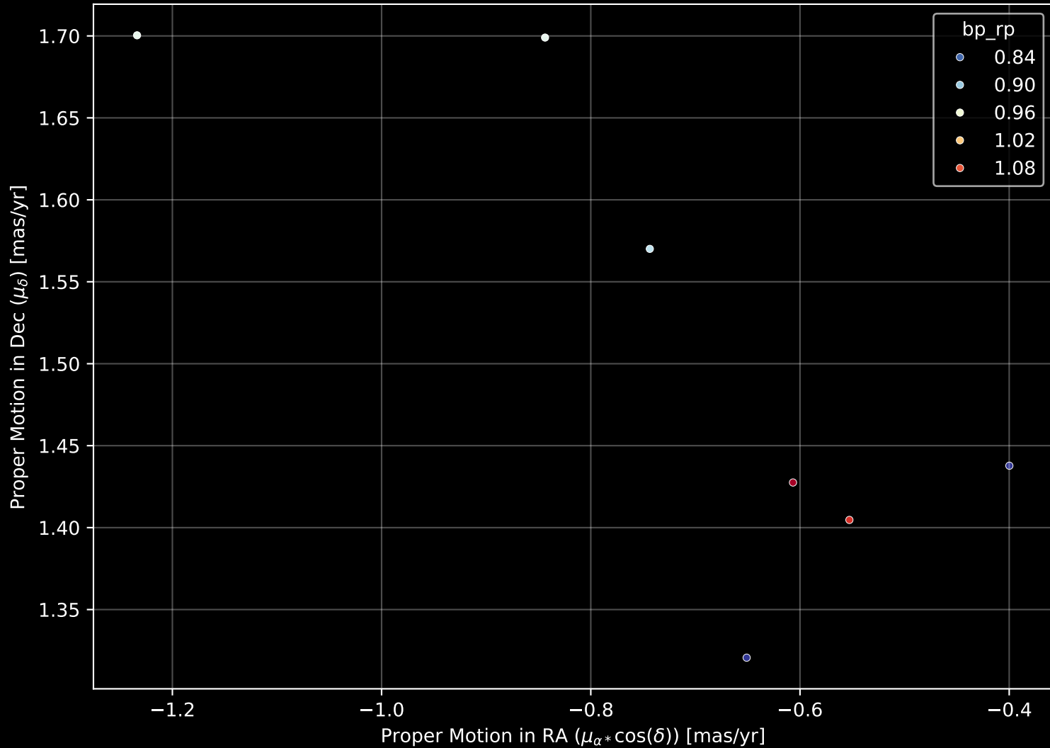
Gaia Stream: [C-20] Proper Motion Diagram (n= 7)
