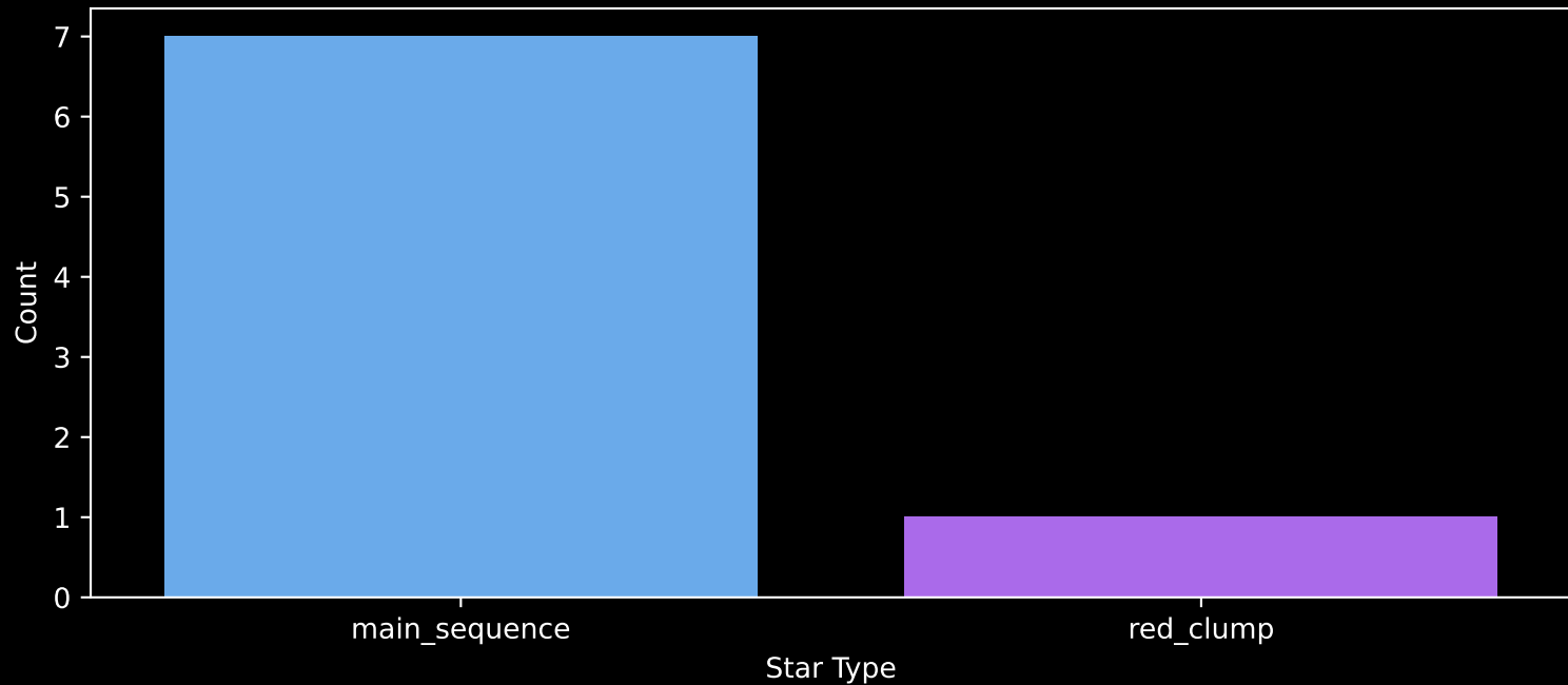
Gaia Stream: [C-22] Count plot of Star Type
