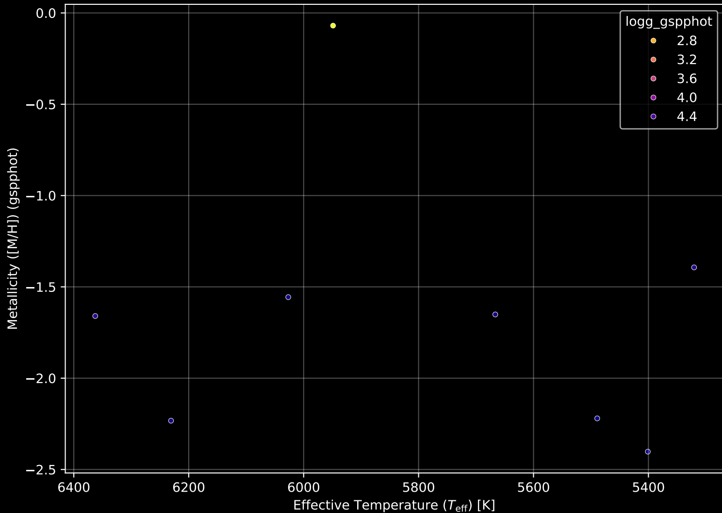
Gaia Stream: [C-22] Stellar Population Parameters (n= 8)
