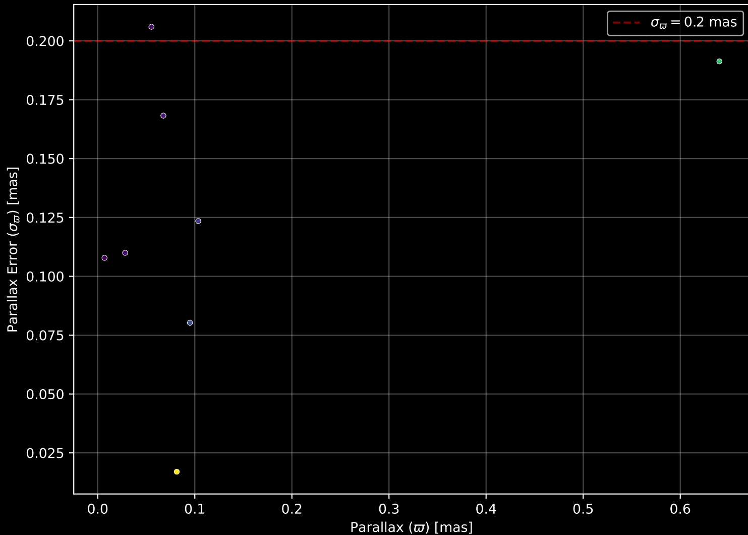
Gaia Stream: [C-22] Parallax Quality (n= 8)
