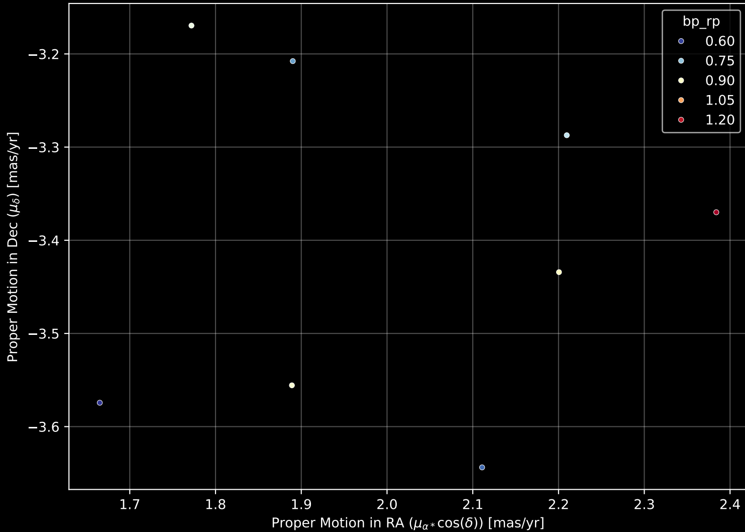
Gaia Stream: [C-22] Proper Motion Diagram (n= 8)
