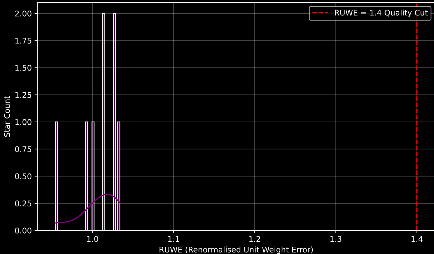
Gaia Stream: [C-22] RUWE Distribution (n= 8)
