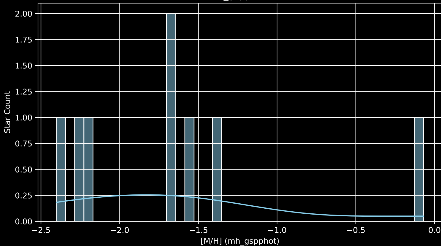
Gaia Stream: [C-22 [M/H] (mh_gspphot) (n= 8)
