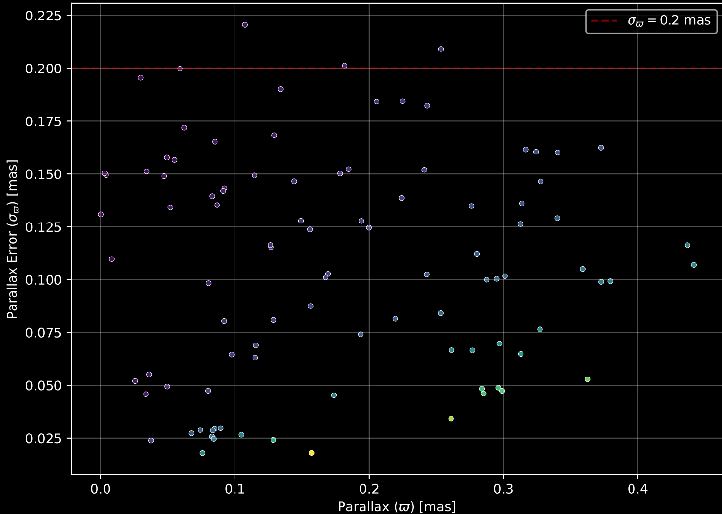
Gaia Stream: [C-24] Parallax Quality (n= 97)
