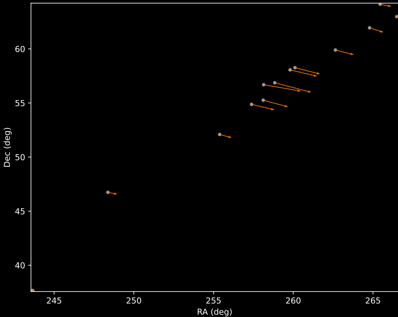
Gaia DR3 Cluster 2 Proper Motion Vectors (n=13)
