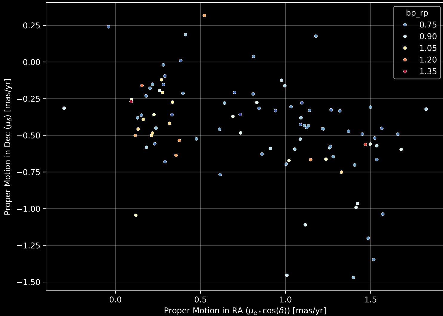
Gaia Stream: [C-24] Proper Motion Diagram (n= 97)
