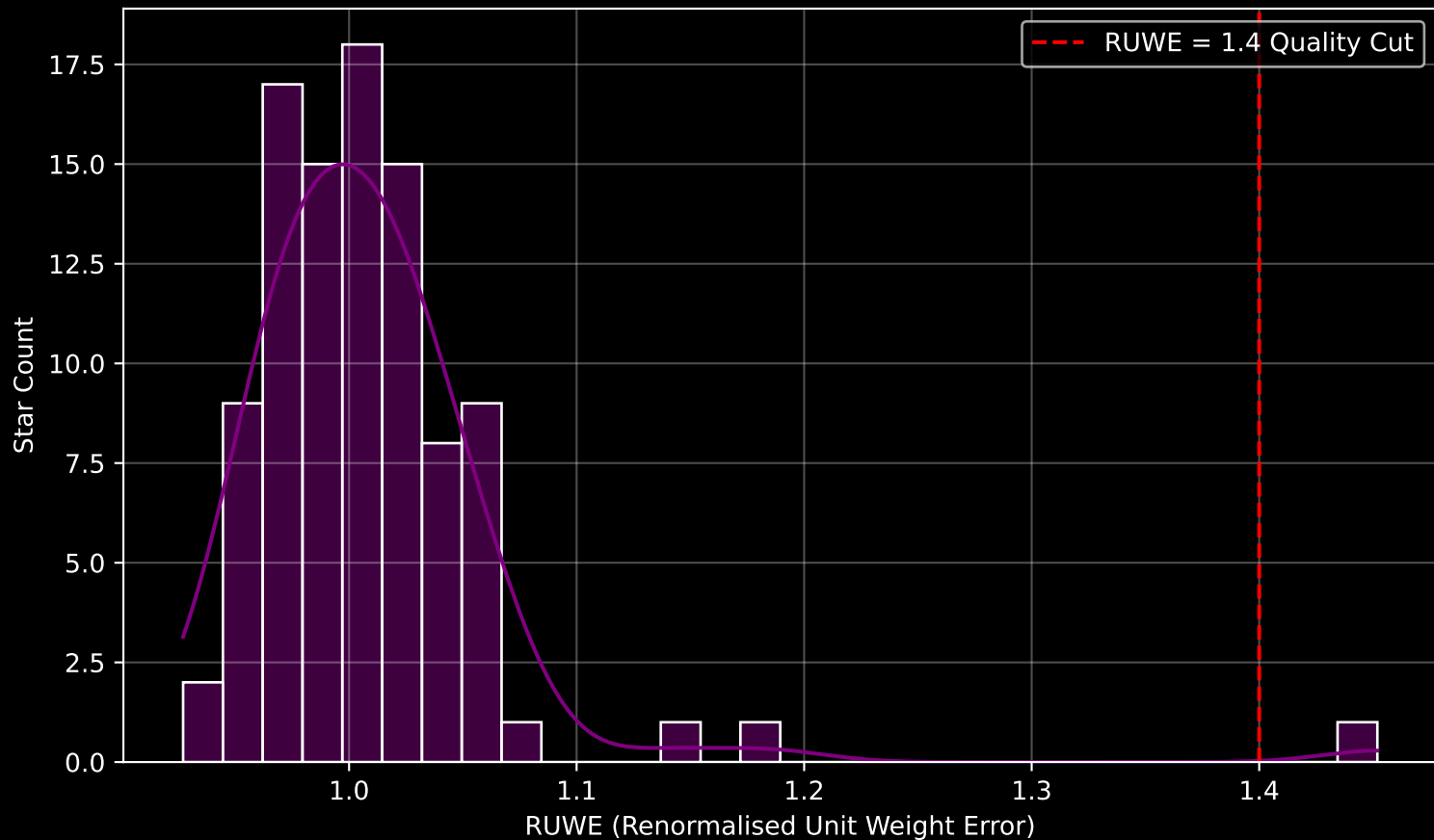
Gaia Stream: [C-24] RUWE Distribution (n= 97)
