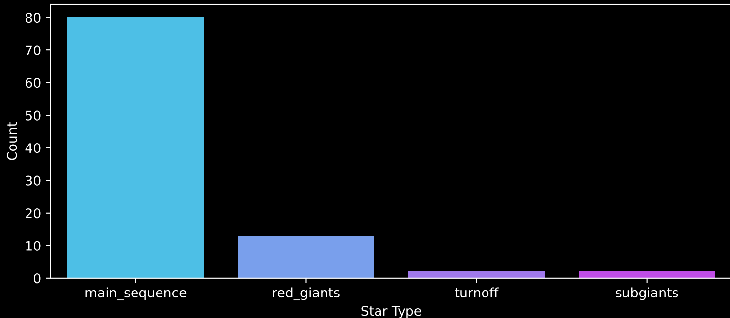
Gaia Stream: [C-24] Count plot of Star Type
