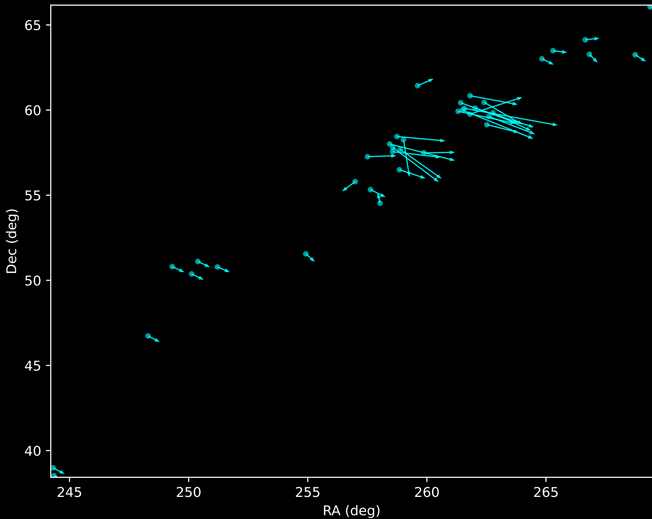
Gaia DR3 Noise Stream Proper Motion Vectors (n=38)
