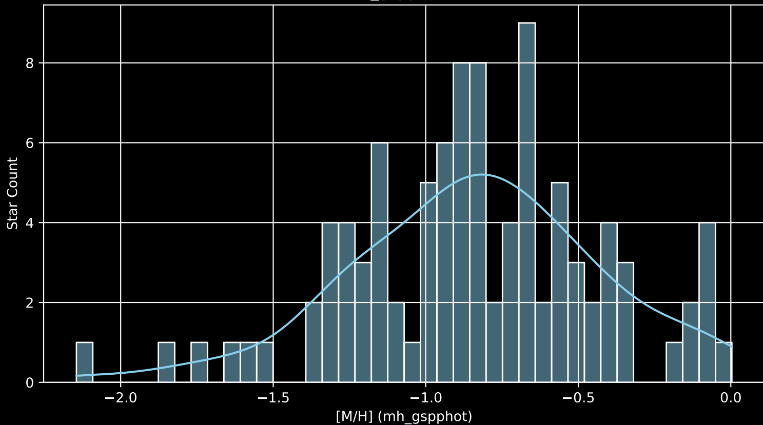
Gaia Stream: [C-24 [M/H] (mh_gspphot) (n= 97)
