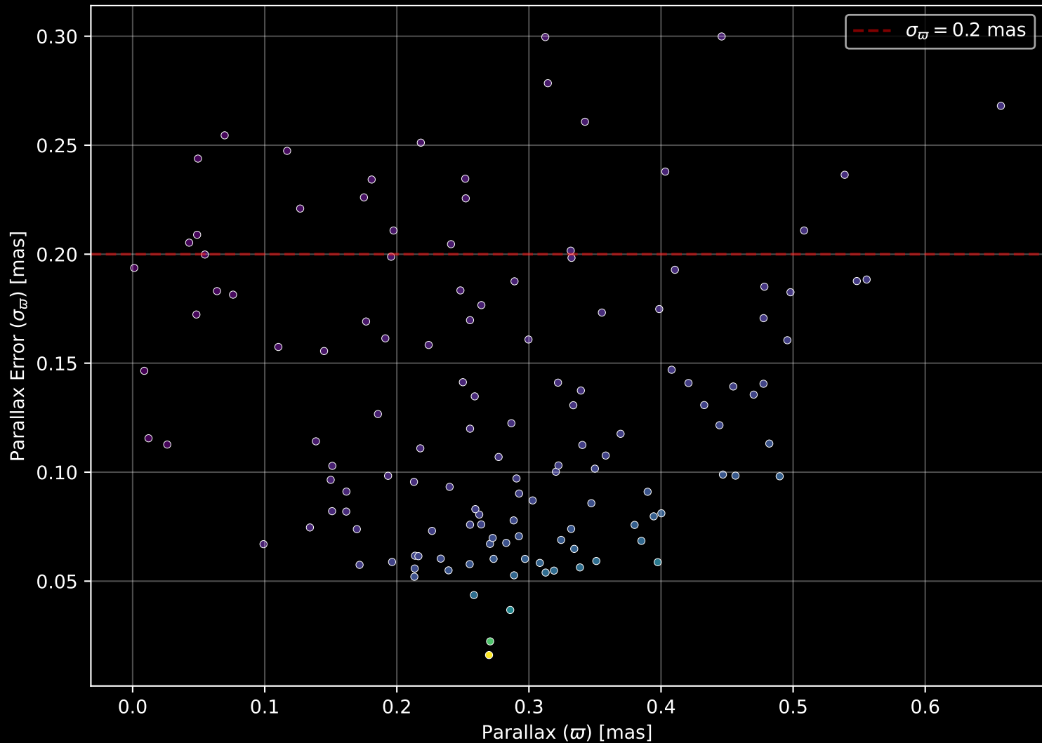
Gaia Stream: [C-9] Parallax Quality (n= 134)
