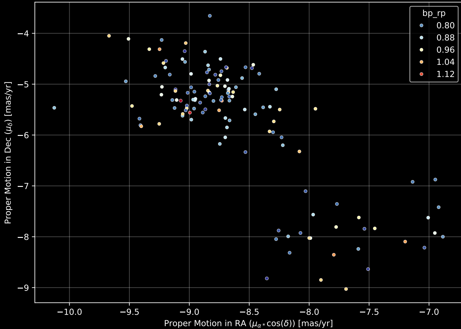
Gaia Stream: [C-9] Proper Motion Diagram (n= 134)
