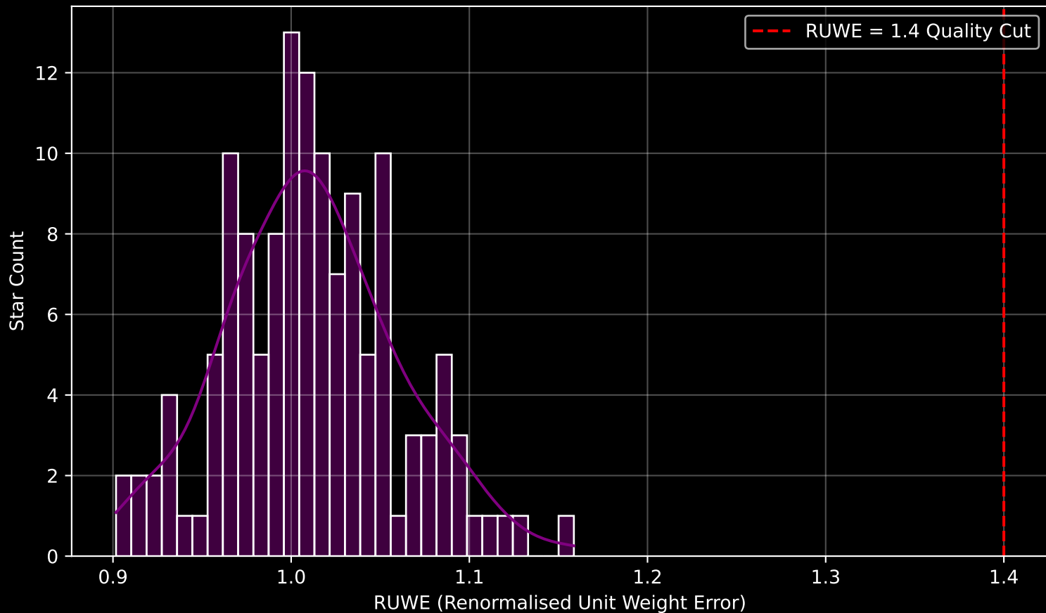
Gaia Stream: [C-9] RUWE Distribution (n= 134)
