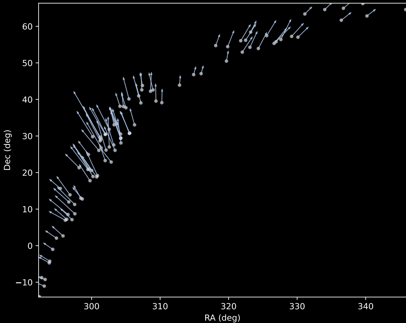
Gaia DR3 Cluster 1 Proper Motion Vectors (n=90)
