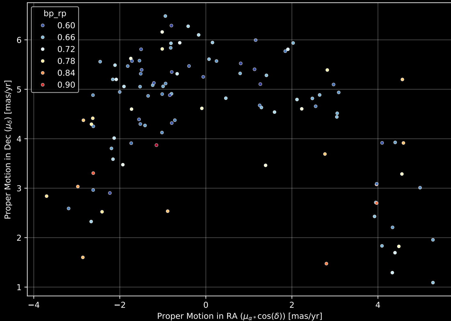
Gaia Stream: [Fjorm] Proper Motion Diagram (n= 111)
