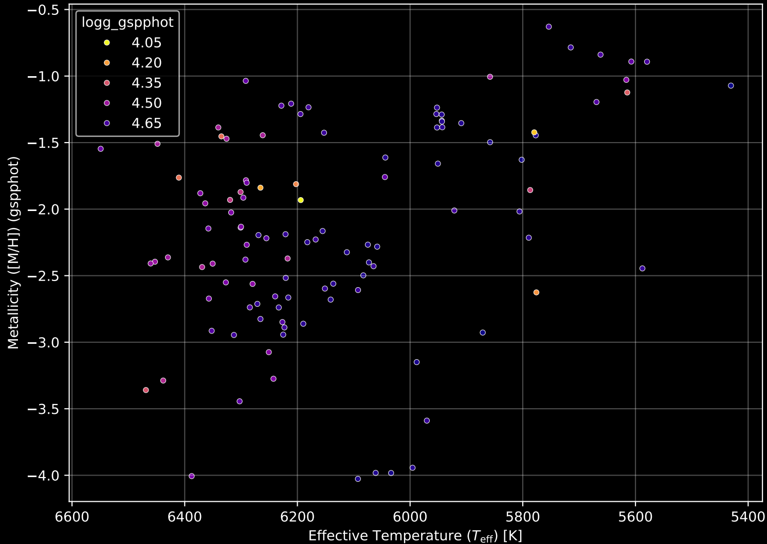
Gaia Stream: [F form ] Stellar Population Parameters (n= 111)
