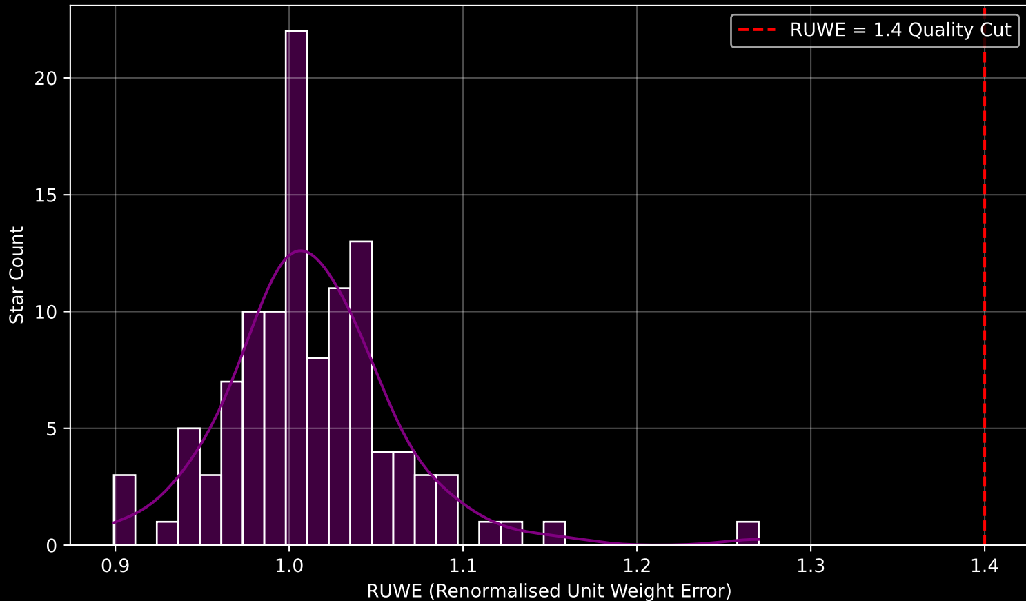
Gaia Stream: [Fform] RUWE Distribution (n= 111)
