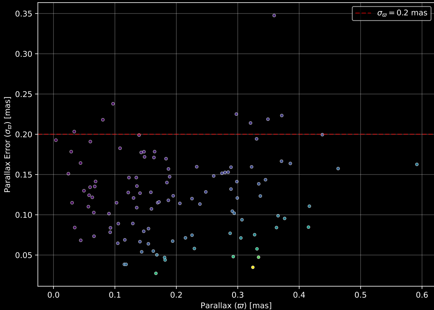
Gaia Stream: [Fform] Parallax Quality (n= 111)
