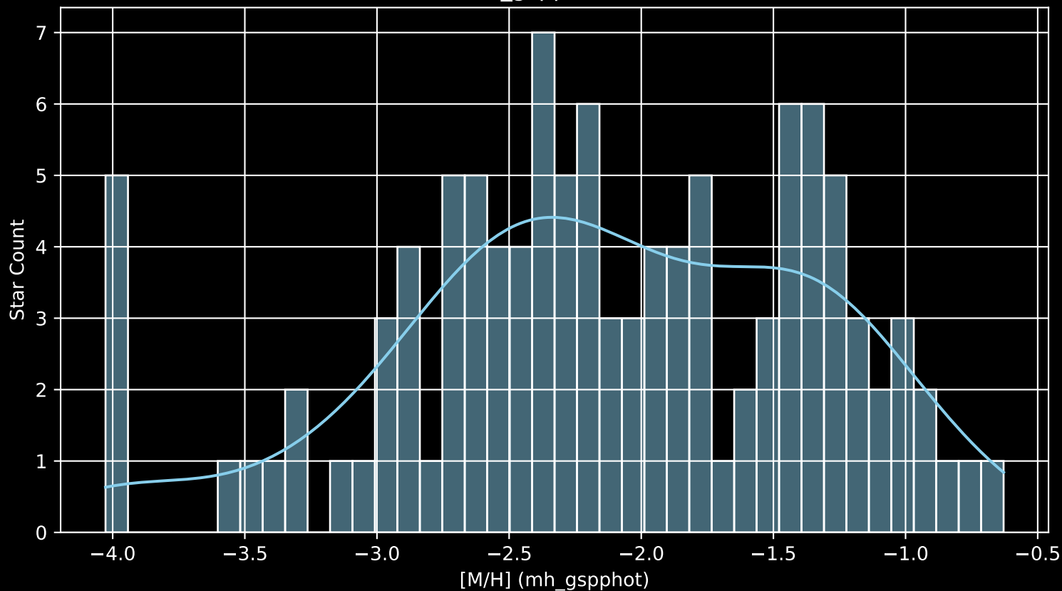
Gaia Stream: [Fjorm [M/H] (mh_gspphot) (n= 111)
