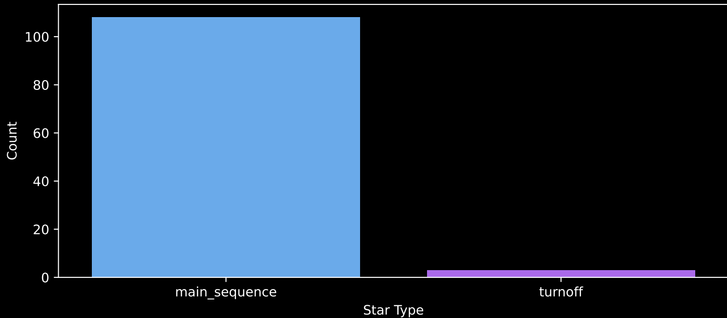
Gaia Stream: [Fjorm] Count plot of Star Type
