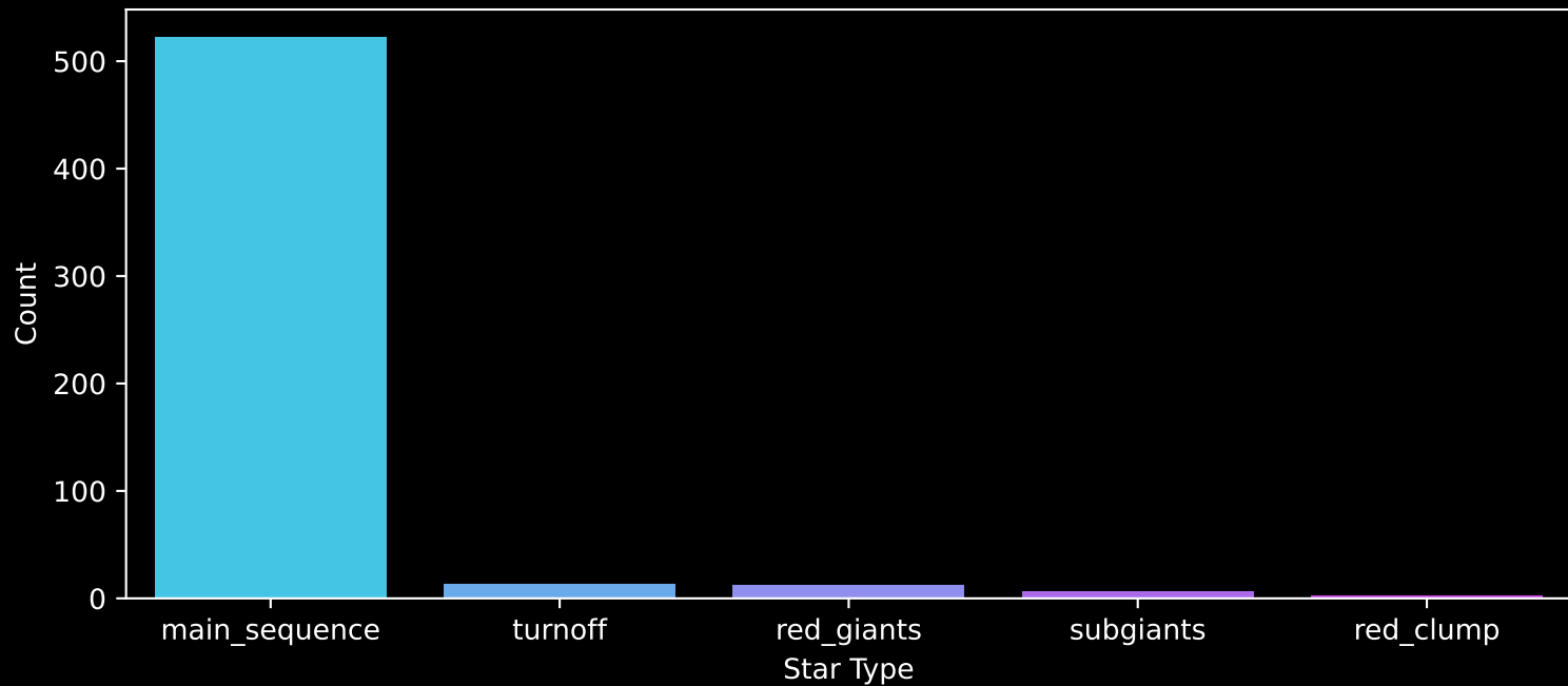
Gaia Stream: [GD-1] Count plot of Star Type
