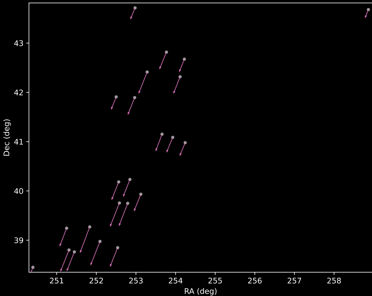
Gaia DR3 Cluster 12 Proper Motion Vectors (n=23)
