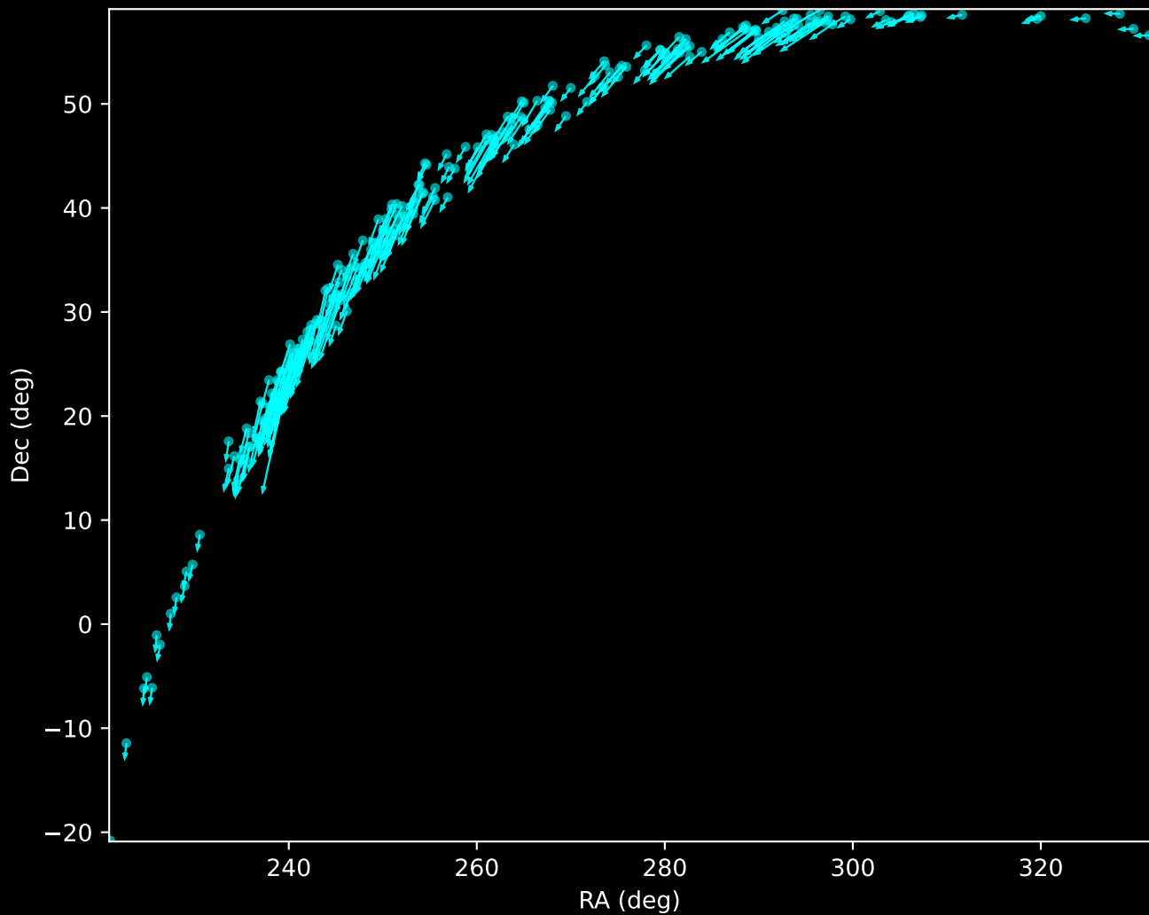
Gaia DR3 Noise Stream Proper Motion Vectors (n=241)
