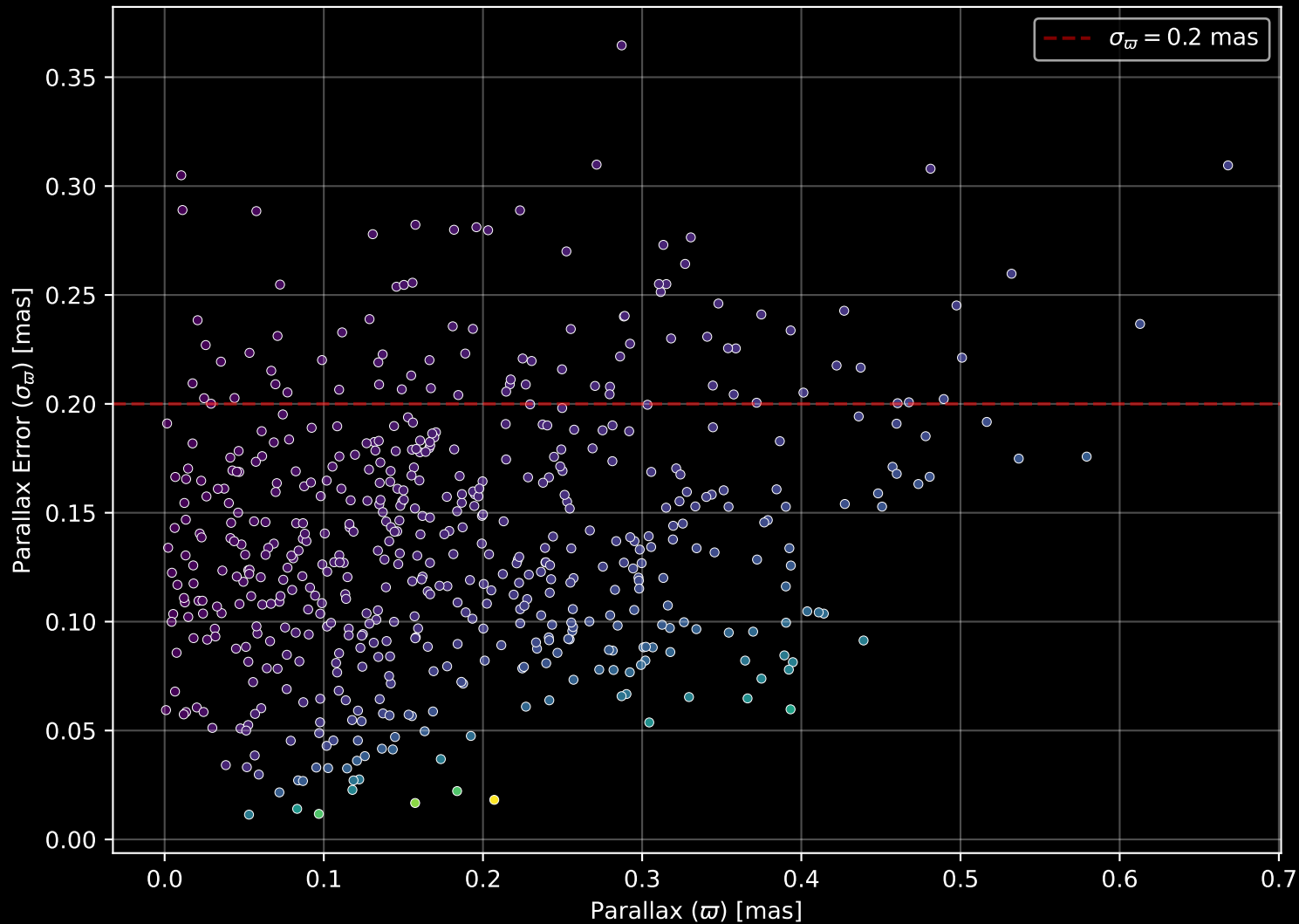
Gaia Stream: [GD-1] Parallax Quality (n= 555)
