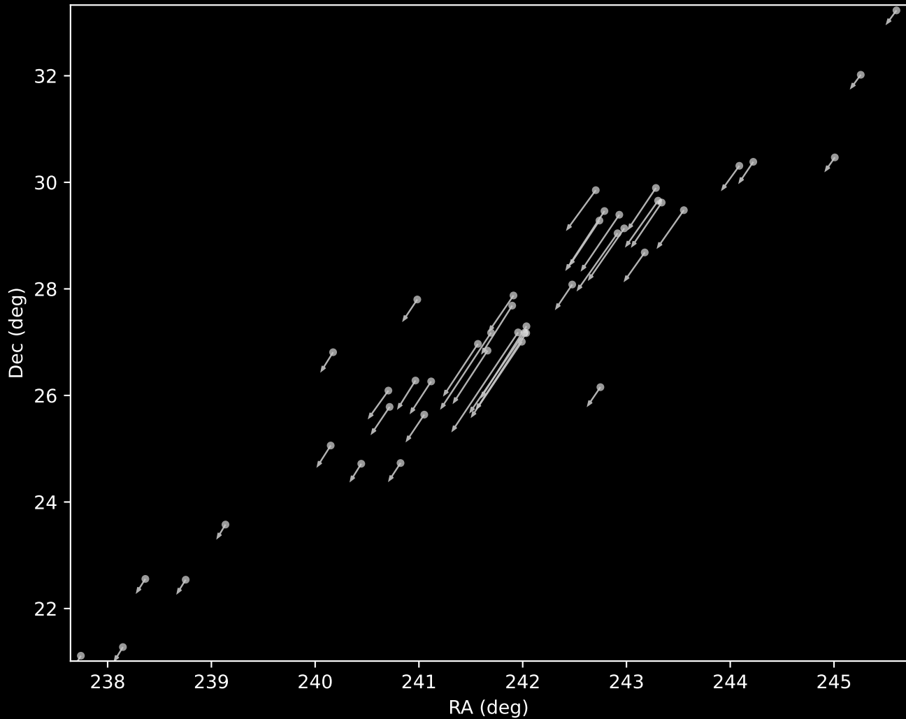
Gaia DR3 Cluster 15 Proper Motion Vectors (n=43)
