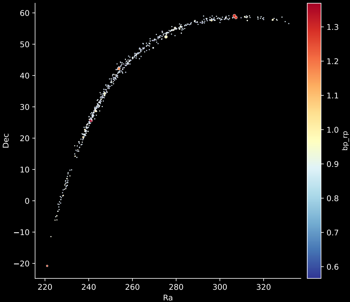
Gaia Stream: [GD-1] Stars: 555
