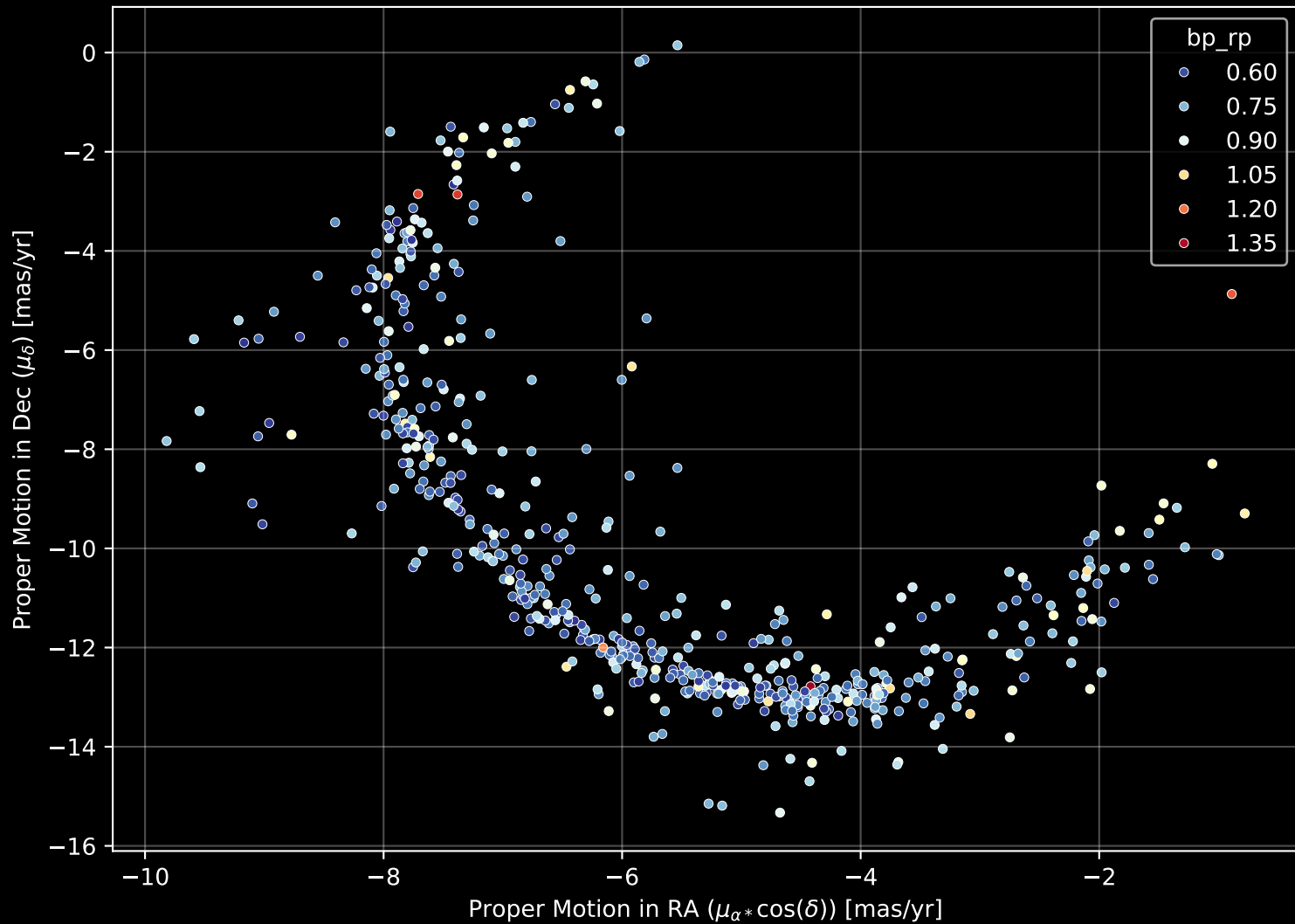
Gaia Stream: [GD-1] Proper Motion Diagram (n= 555)
