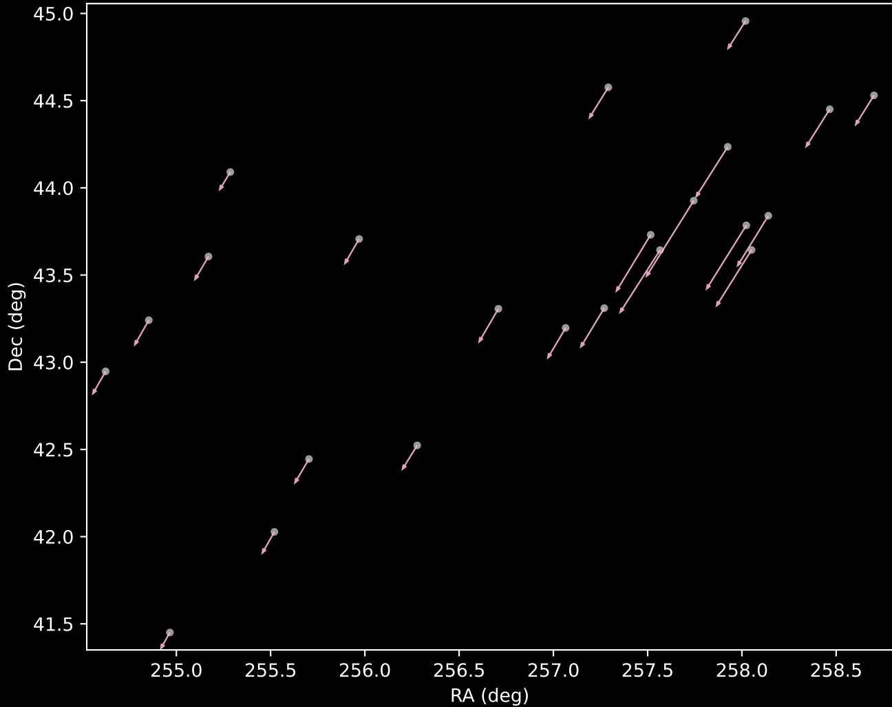
Gaia DR3 Cluster 13 Proper Motion Vectors (n=23)
