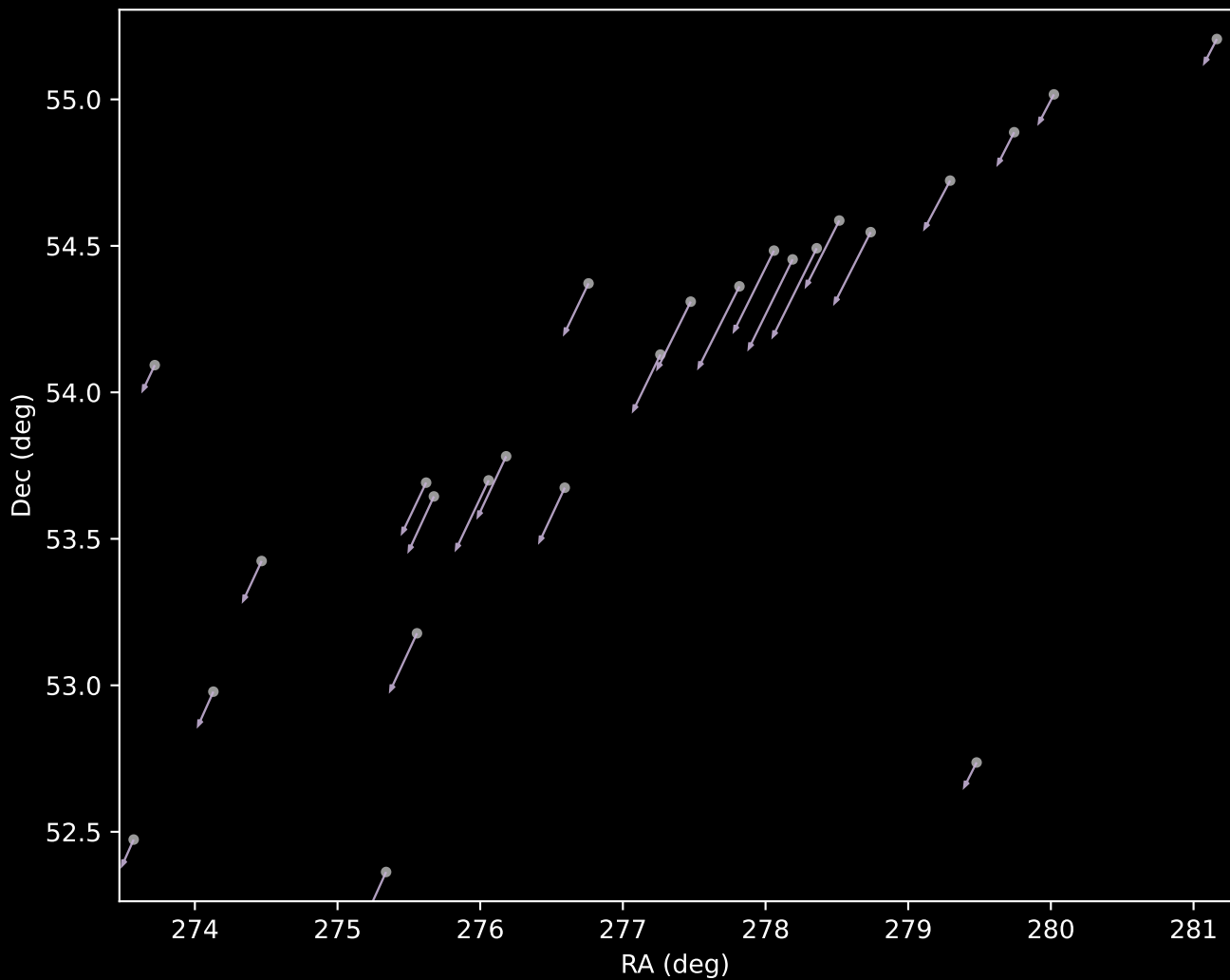
Gaia DR3 Cluster 9 Proper Motion Vectors (n=25)
