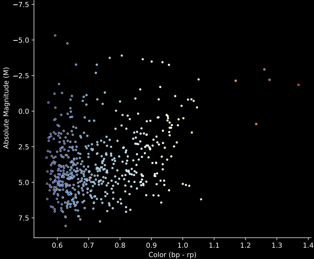
Gaia Stream: [GD-1] Stream (n= 555) Hertzsprung-Russel Diagram
