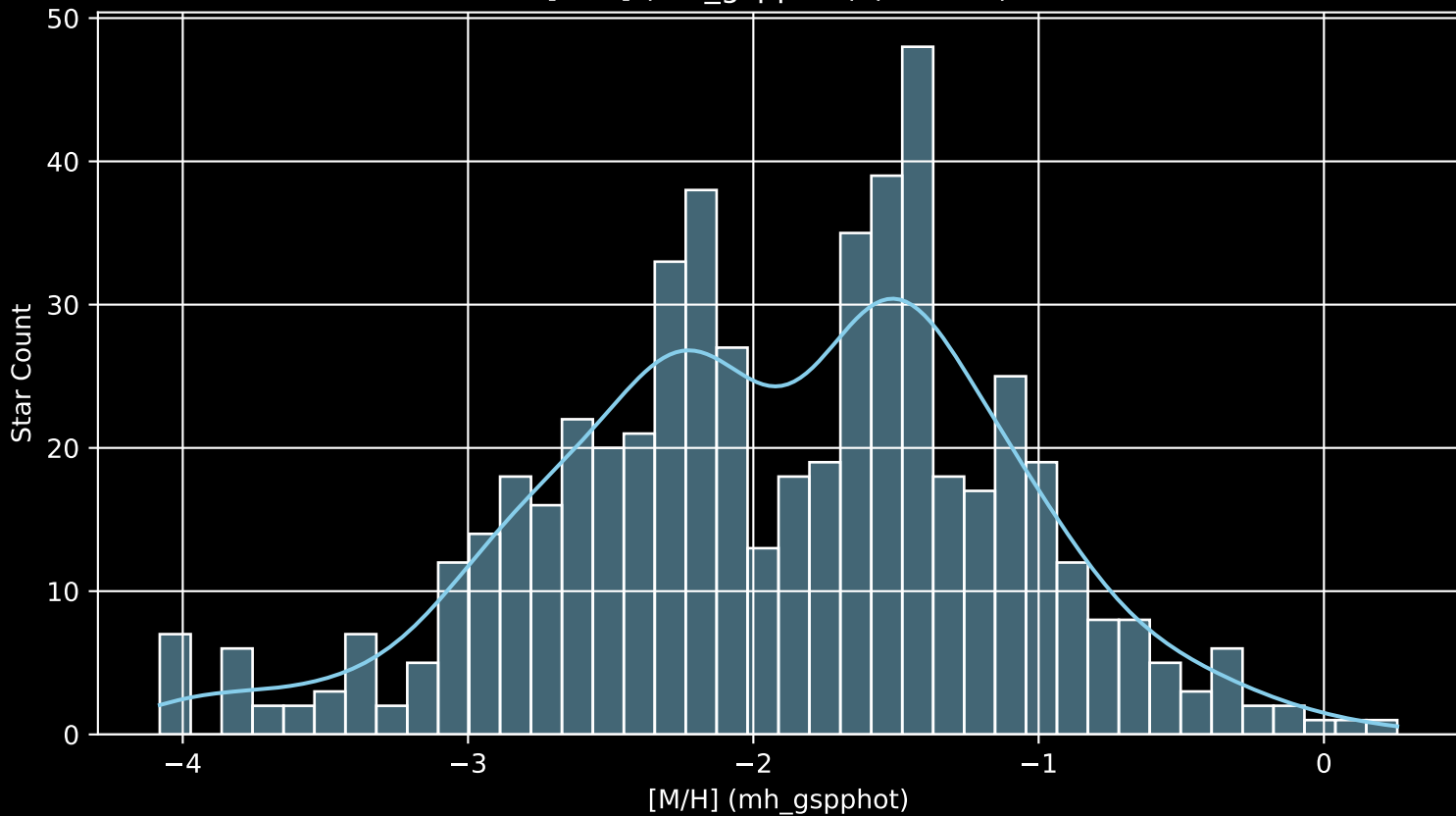
Gaia Stream: [GD-1 [M/H] (mh_gspphot) (n= 555)
