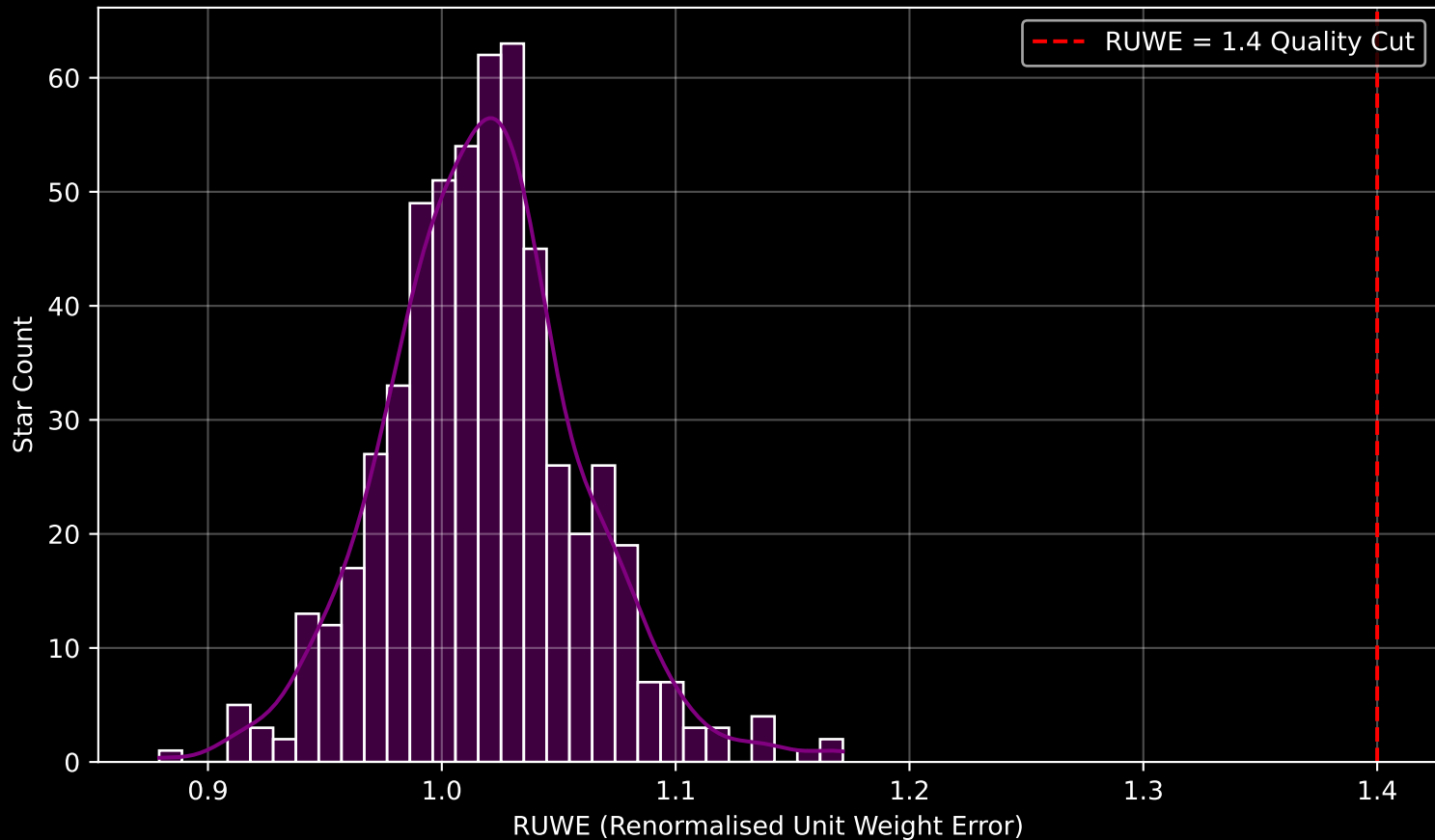
Gaia Stream: [GD-1] RUWE Distribution (n= 555)
