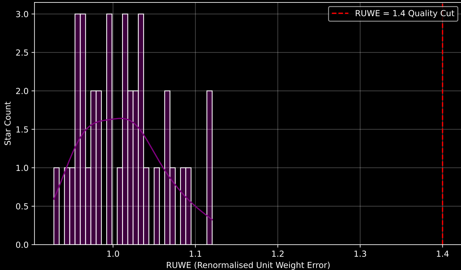
Gaia Stream: [Gaia-10] RUWE Distribution (n= 37)
