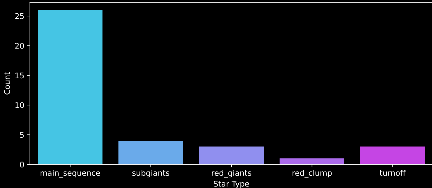
Gaia Stream: [Gaia-10] Count plot of Star Type
