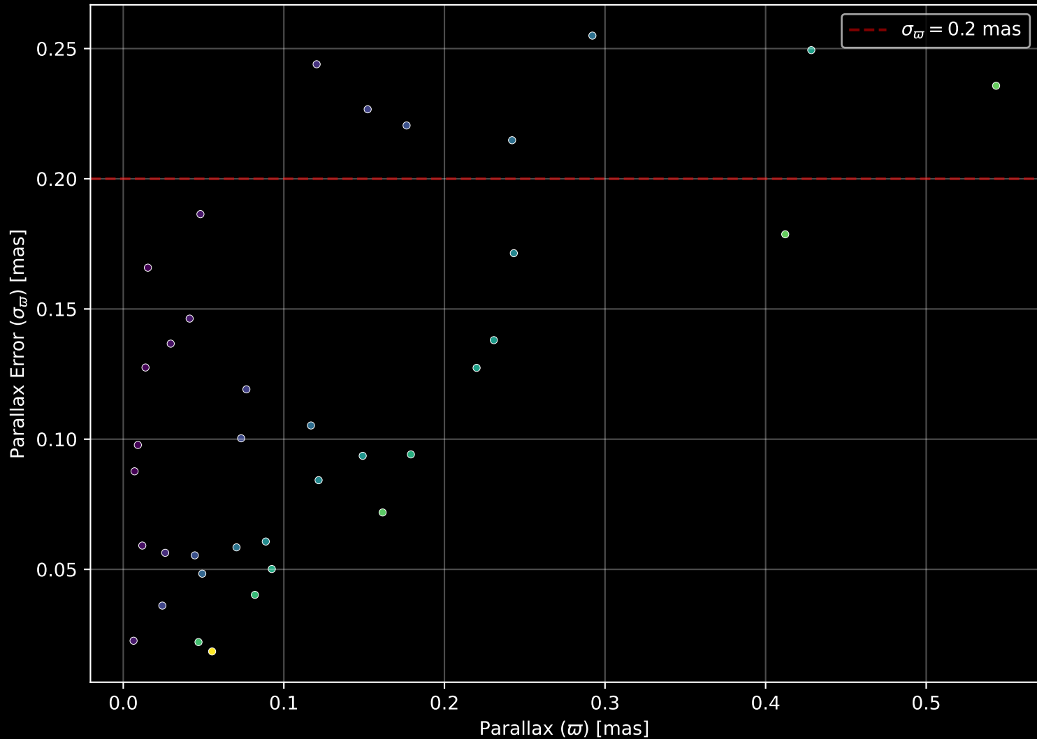
Gaia Stream: [Gaia-10] Parallax Quality (n= 37)
