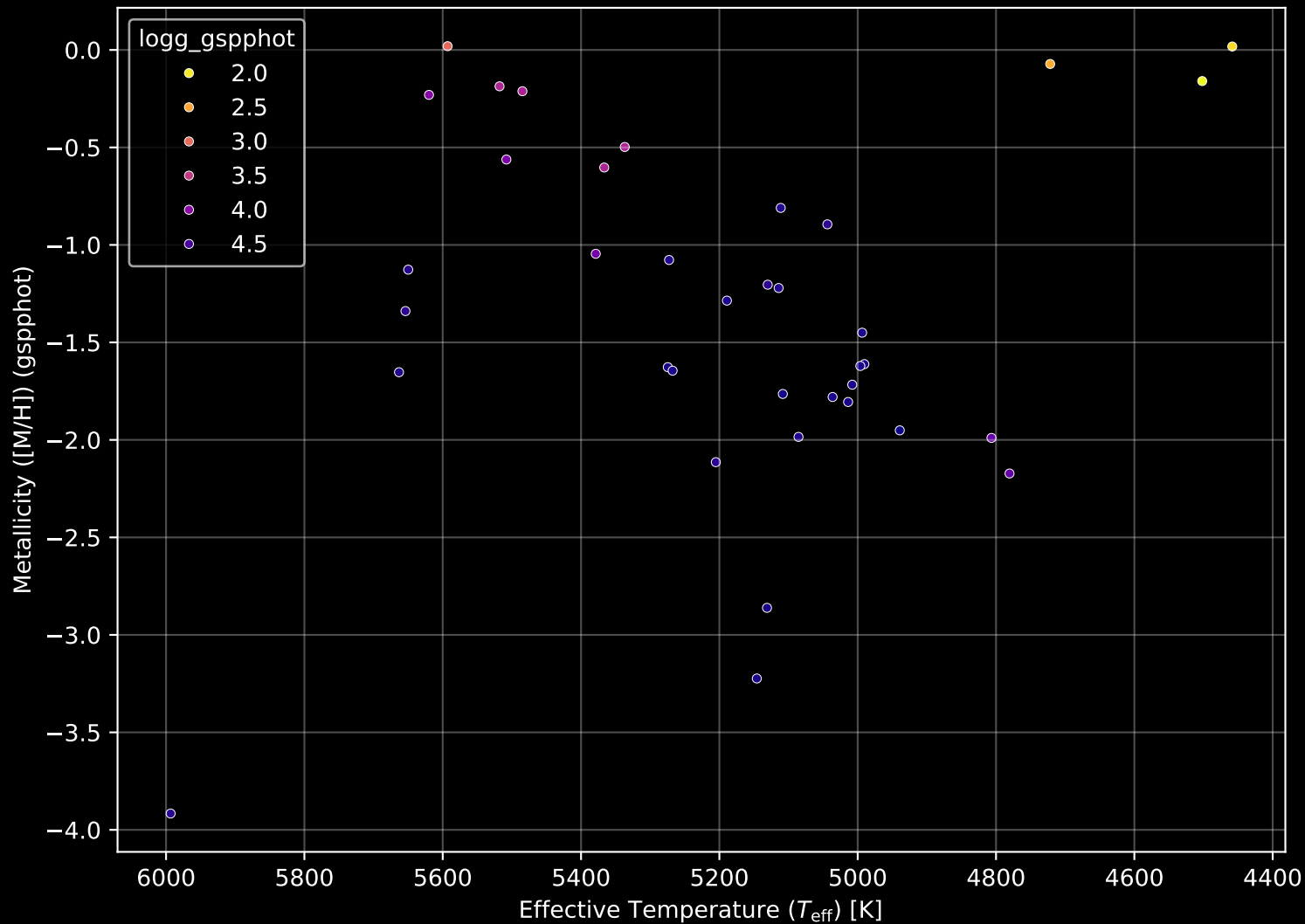
Gaia Stream: [Gaia-10] Stellar Population Parameters (n= 37)
