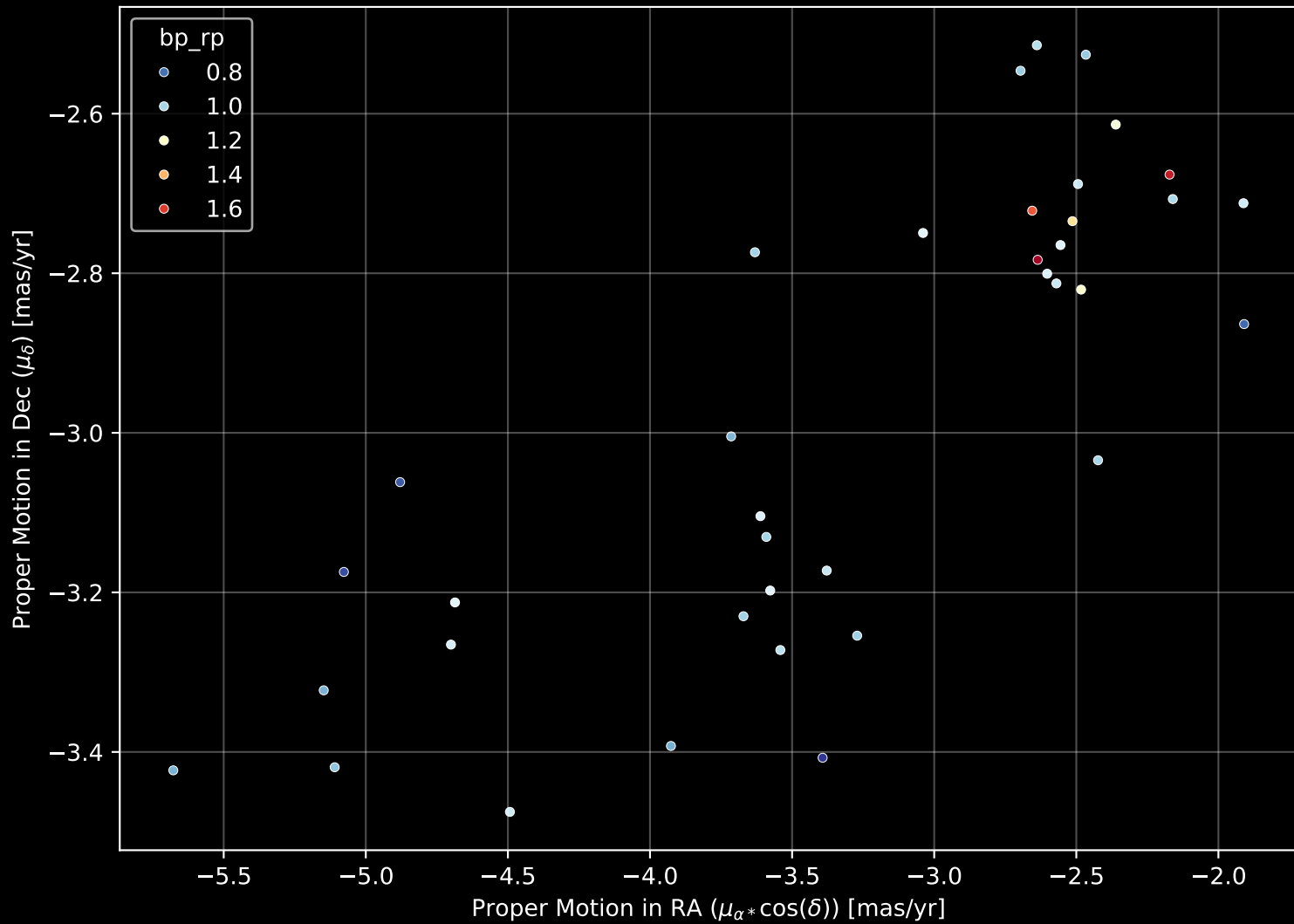
Gaia Stream: [Gaia-10] Proper Motion Diagram (n= 37)
