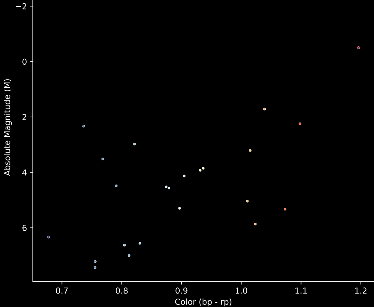
Gaia Stream: [Gaia-12] Stream (n= 24) Hertzsprung-Russel Diagram
