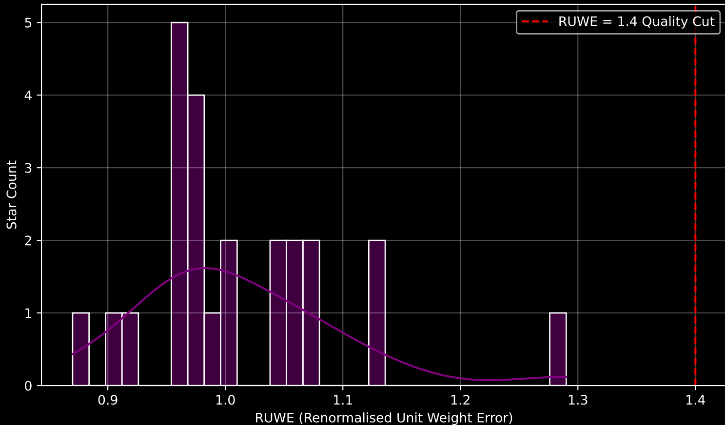
Gaia Stream: [Gaia-12] RUWE Distribution (n= 24)
