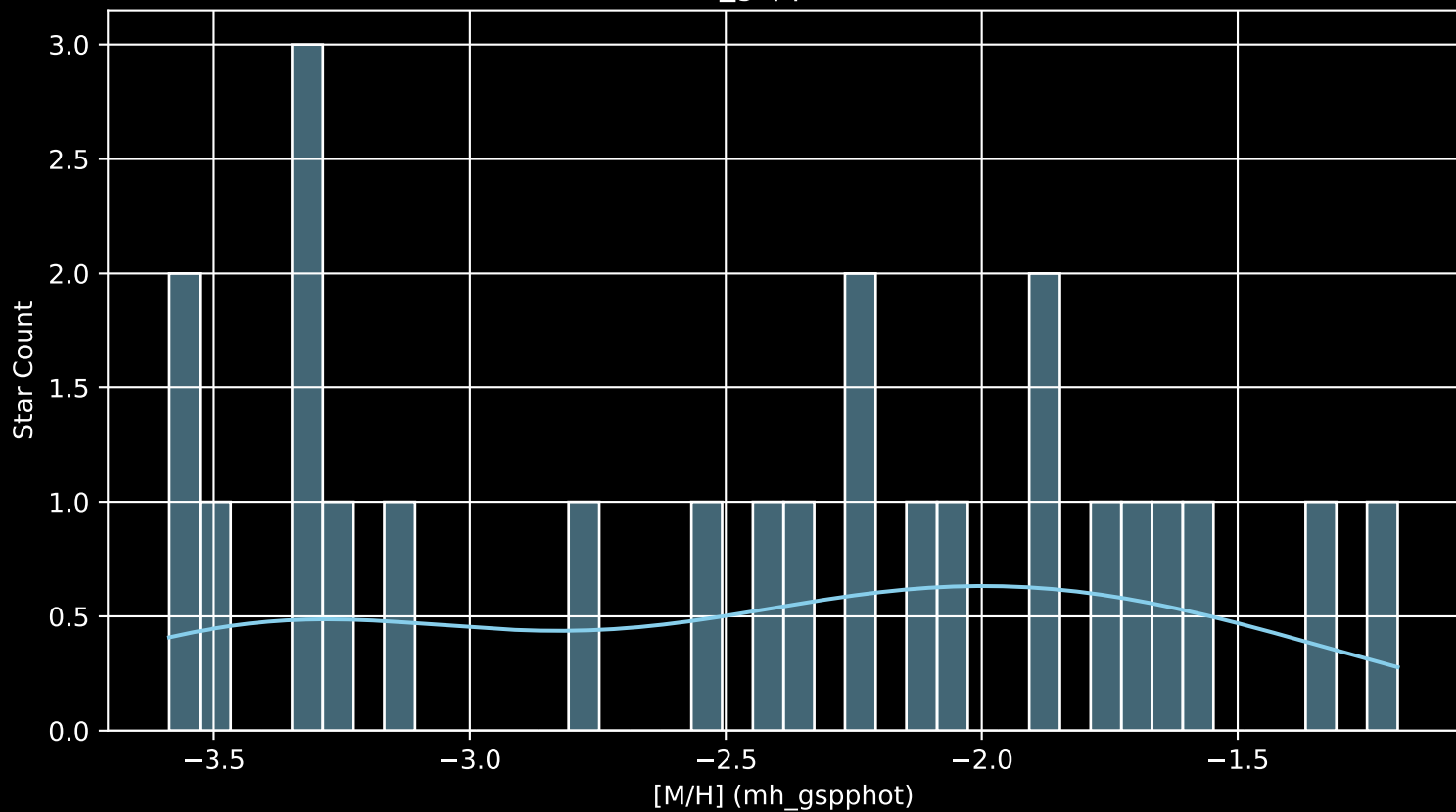
Gaia Stream: [Gaia-12 [M/H] (mh_gspphot) (n= 24)
