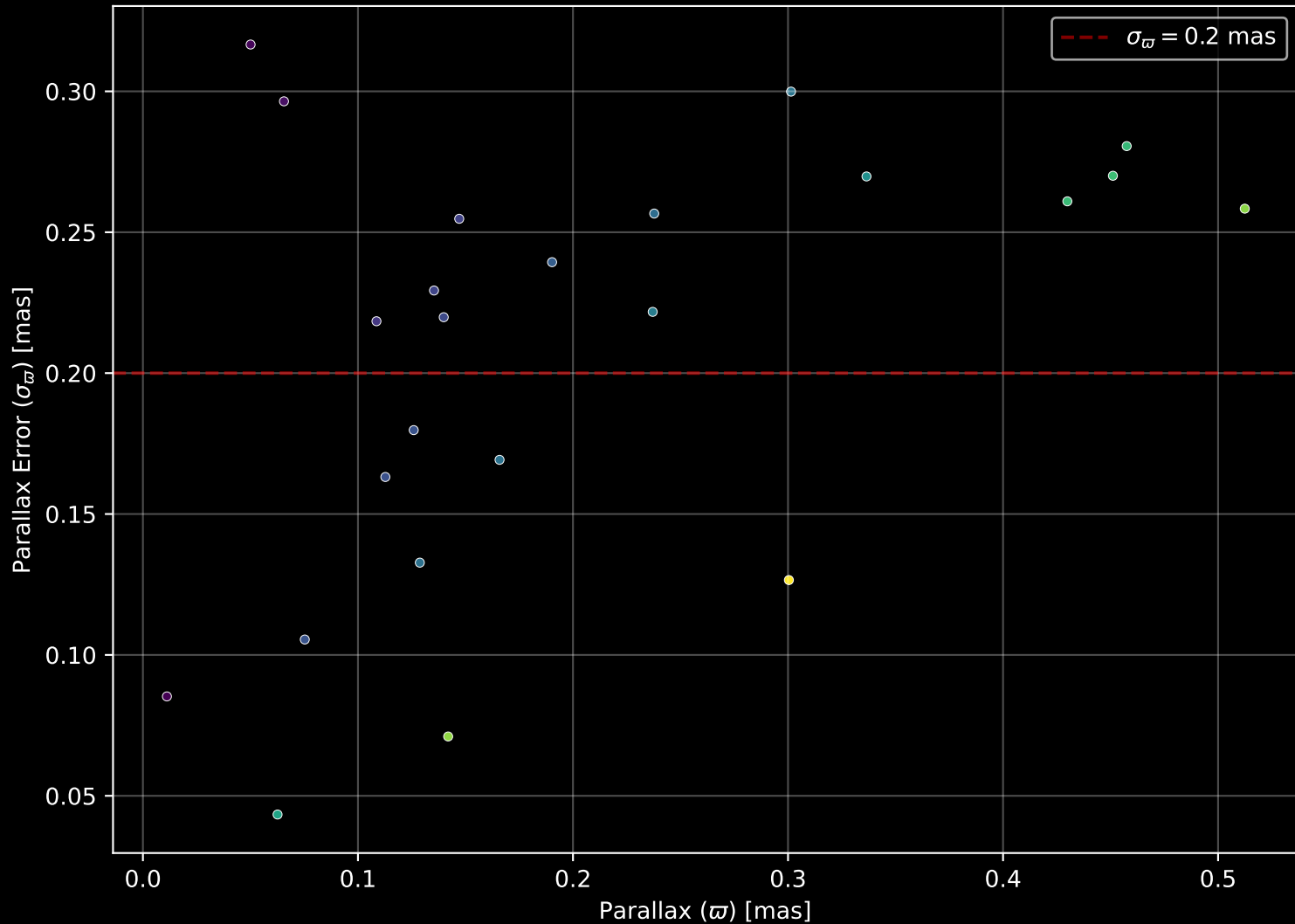
Gaia Stream: [Gaia-12] Parallax Quality (n= 24)
