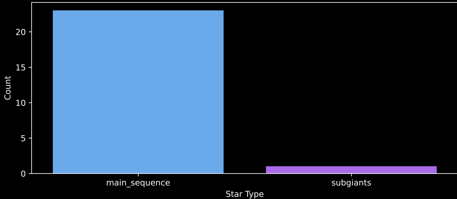
Gaia Stream: [Gaia-12] Count plot of Star Type
