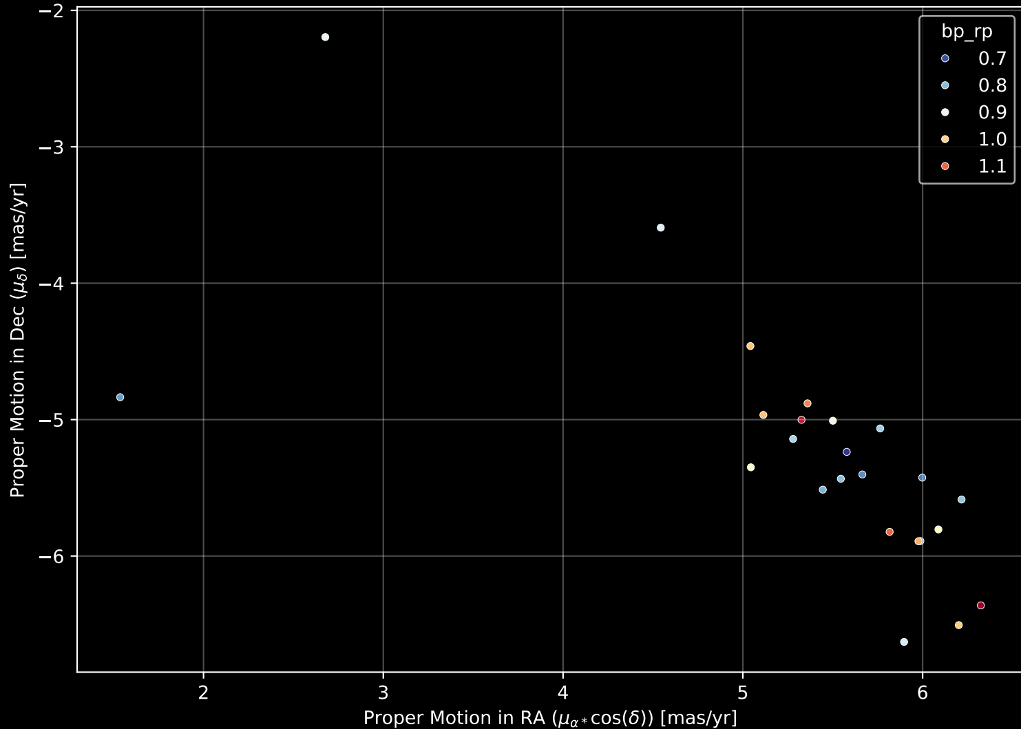
Gaia Stream: [Gaia-12] Proper Motion Diagram (n= 24)
