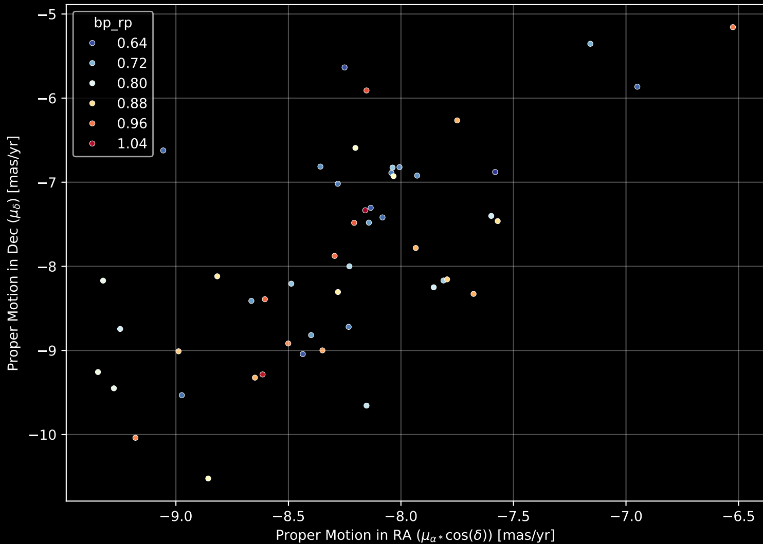
Gaia Stream: [Gaia-6] Proper Motion Diagram (n= 51)
