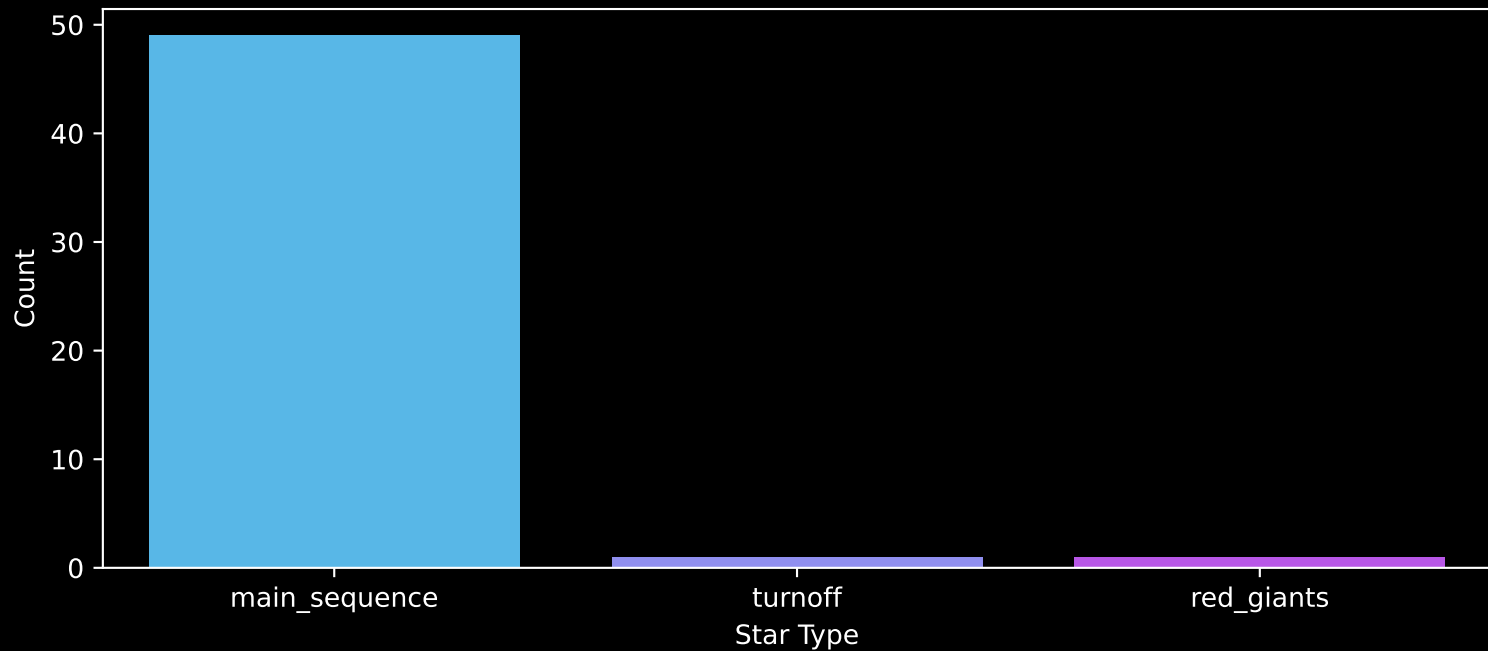
Gaia Stream: [Gaia-6] Count plot of Star Type
