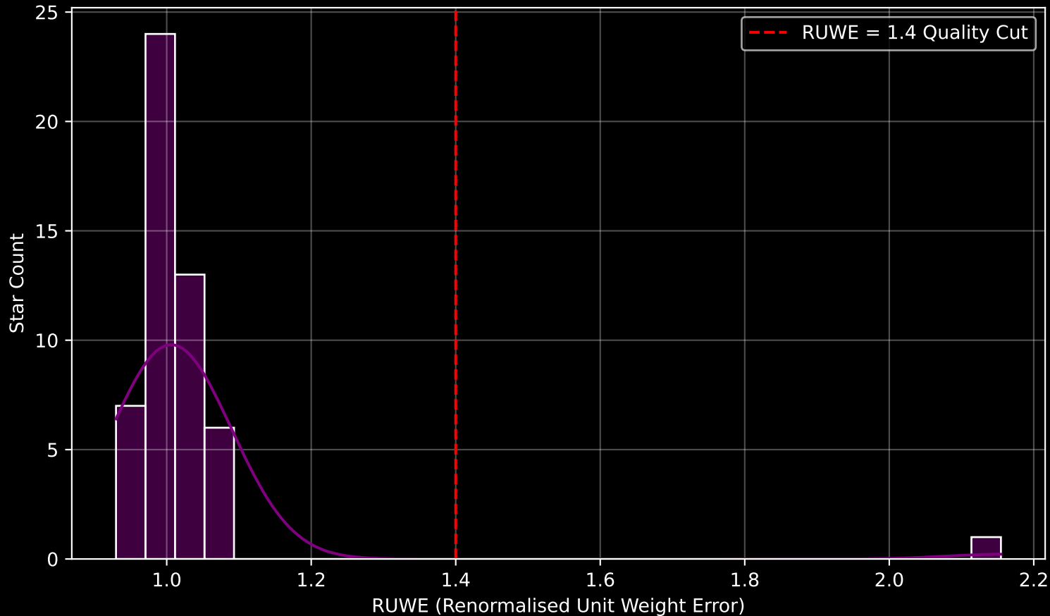
Gaia Stream: [Gaia-6] RUWE Distribution (n= 51)
