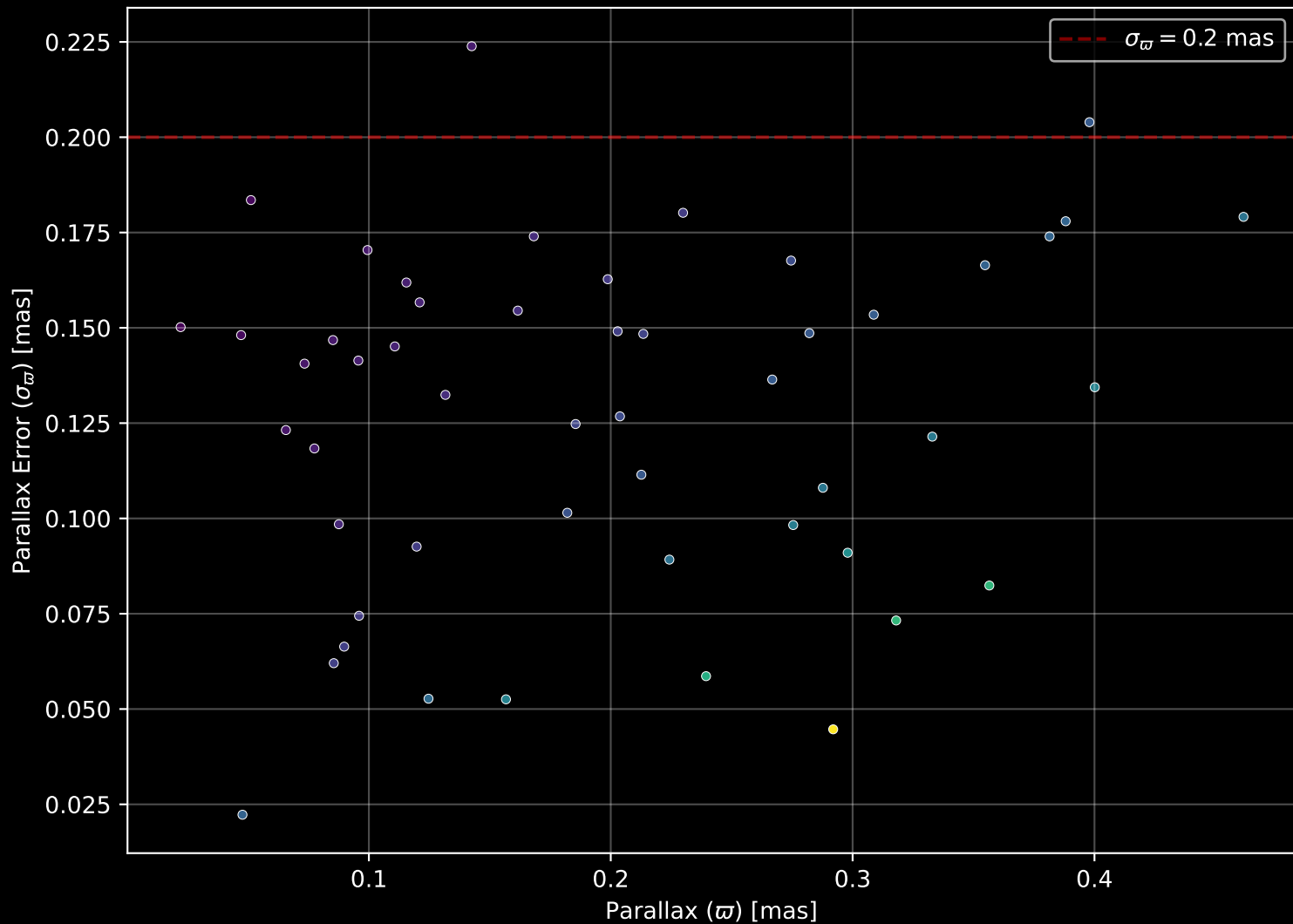
Gaia Stream: [Gaia-6] Parallax Quality (n= 51)
