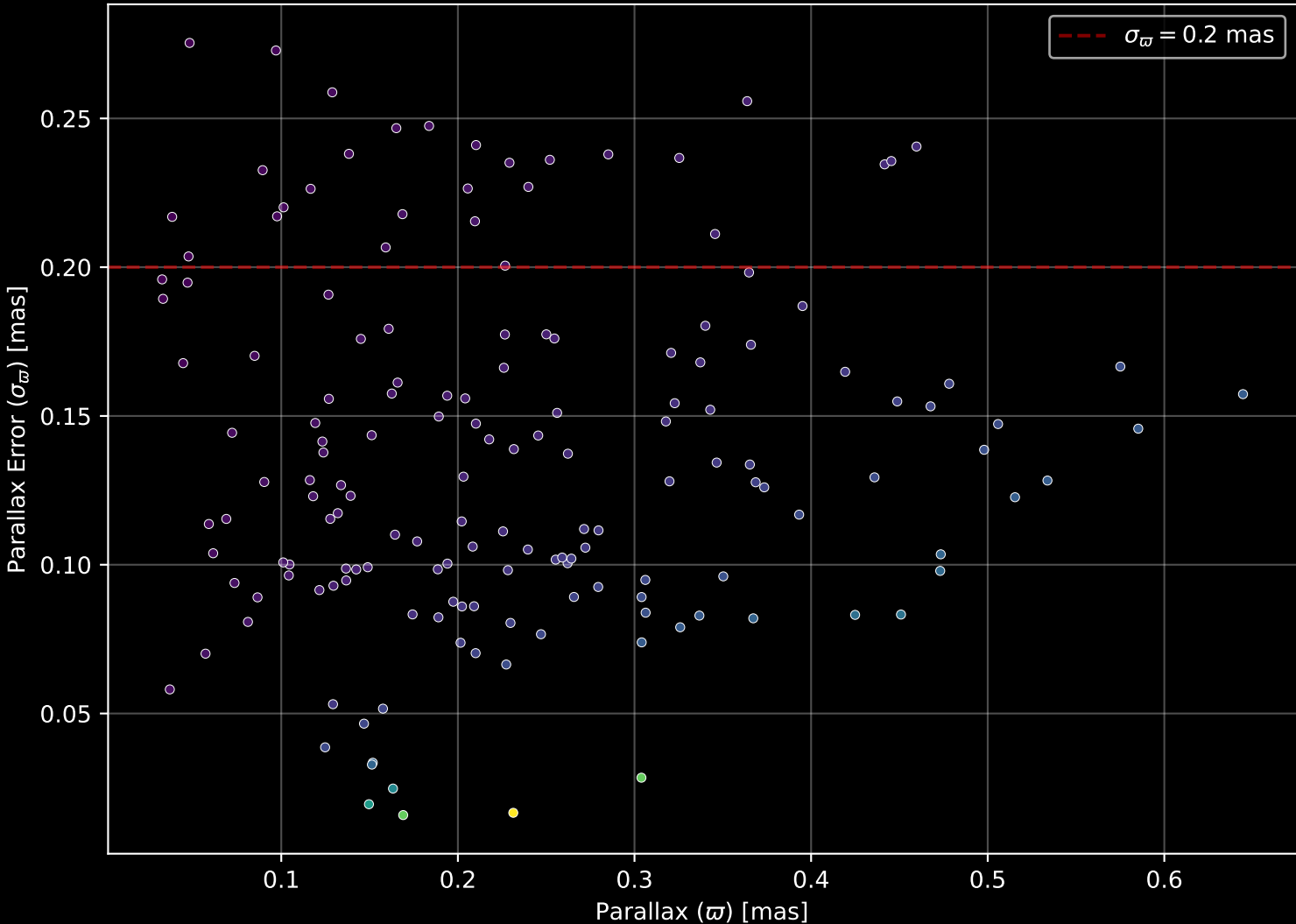
Gaia Stream: [Gaia-7] Parallax Quality (n= 160)
