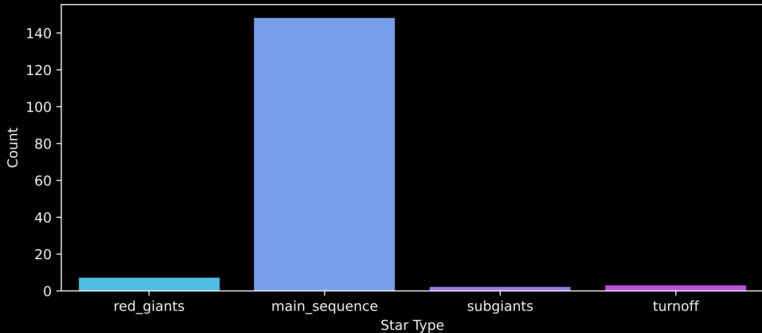
Gaia Stream: [Gaia-7] Count plot of Star Type
