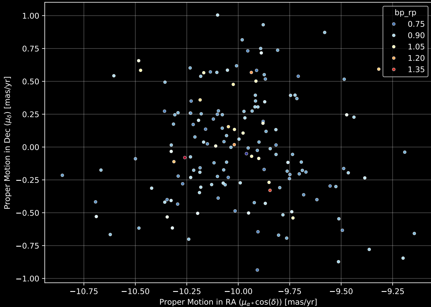
Gaia Stream: [Gaia-7] Proper Motion Diagram (n= 160)
