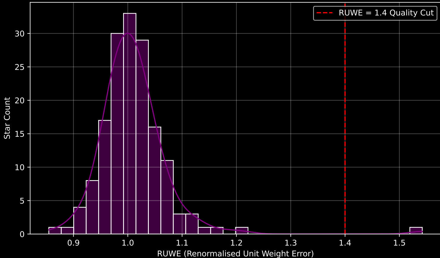
Gaia Stream: [Gaia-7] RUWE Distribution (n= 160)
