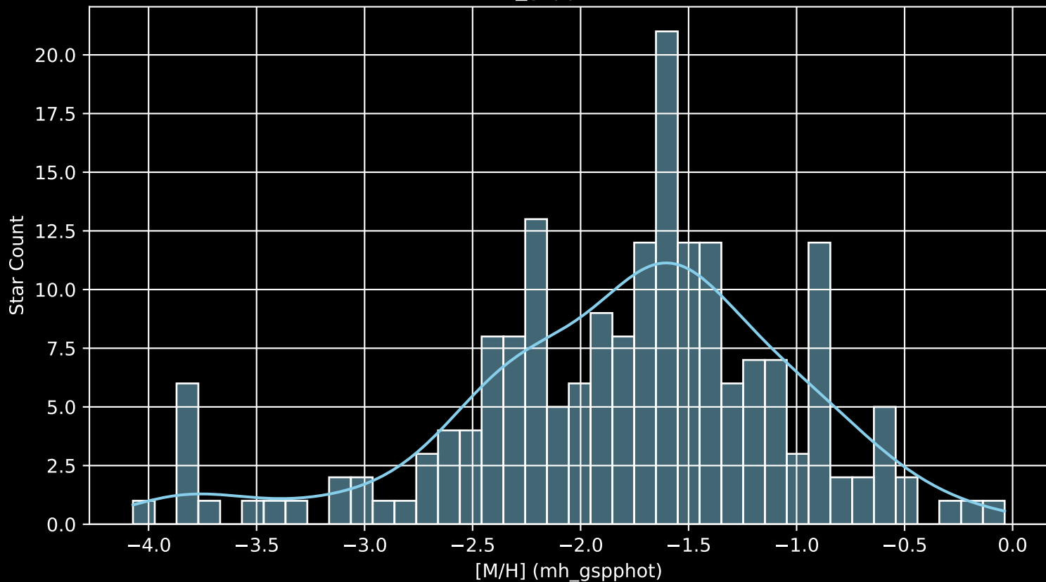
Gaia Stream: [Gaia-8 [M/H] (mh_gspphot) (n= 191)
