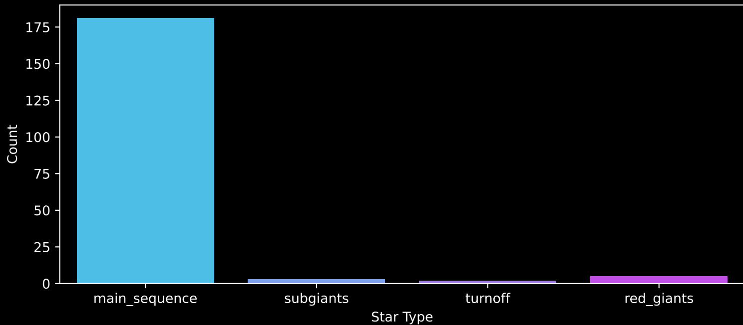
Gaia Stream: [Gaia-8] Count plot of Star Type
