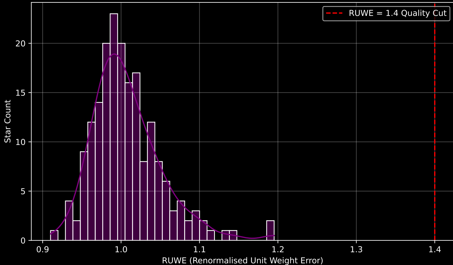
Gaia Stream: [Gaia-8] RUWE Distribution (n= 191)
