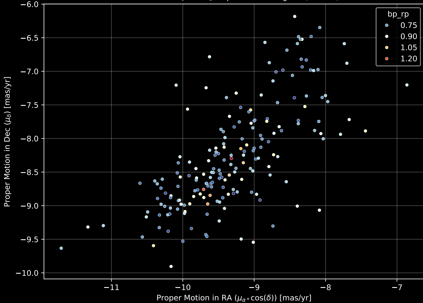
Gaia Stream: [Gaia-8] Proper Motion Diagram (n= 191)
