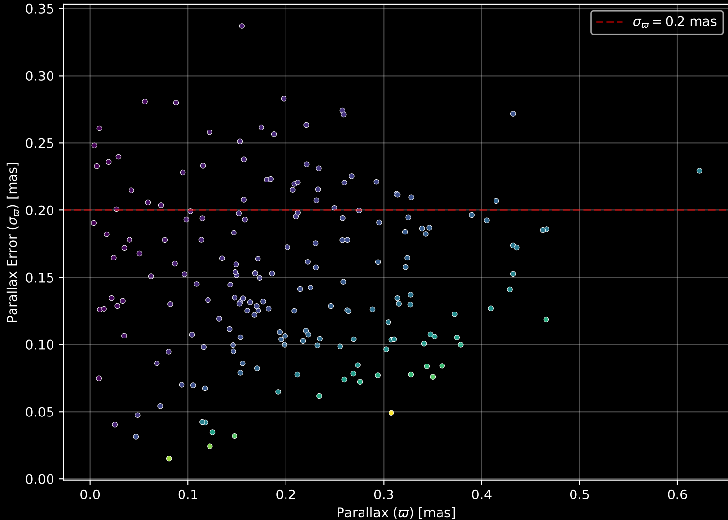
Gaia Stream: [Gaia-8] Parallax Quality (n= 191)
