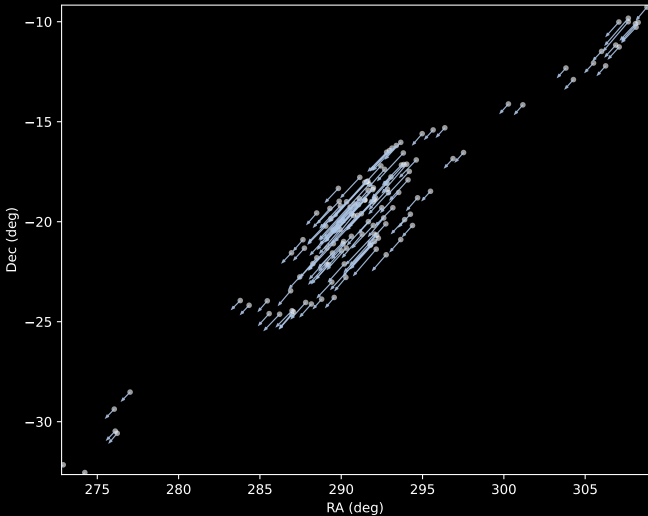
Gaia DR3 Cluster 1 Proper Motion Vectors (n=132)
