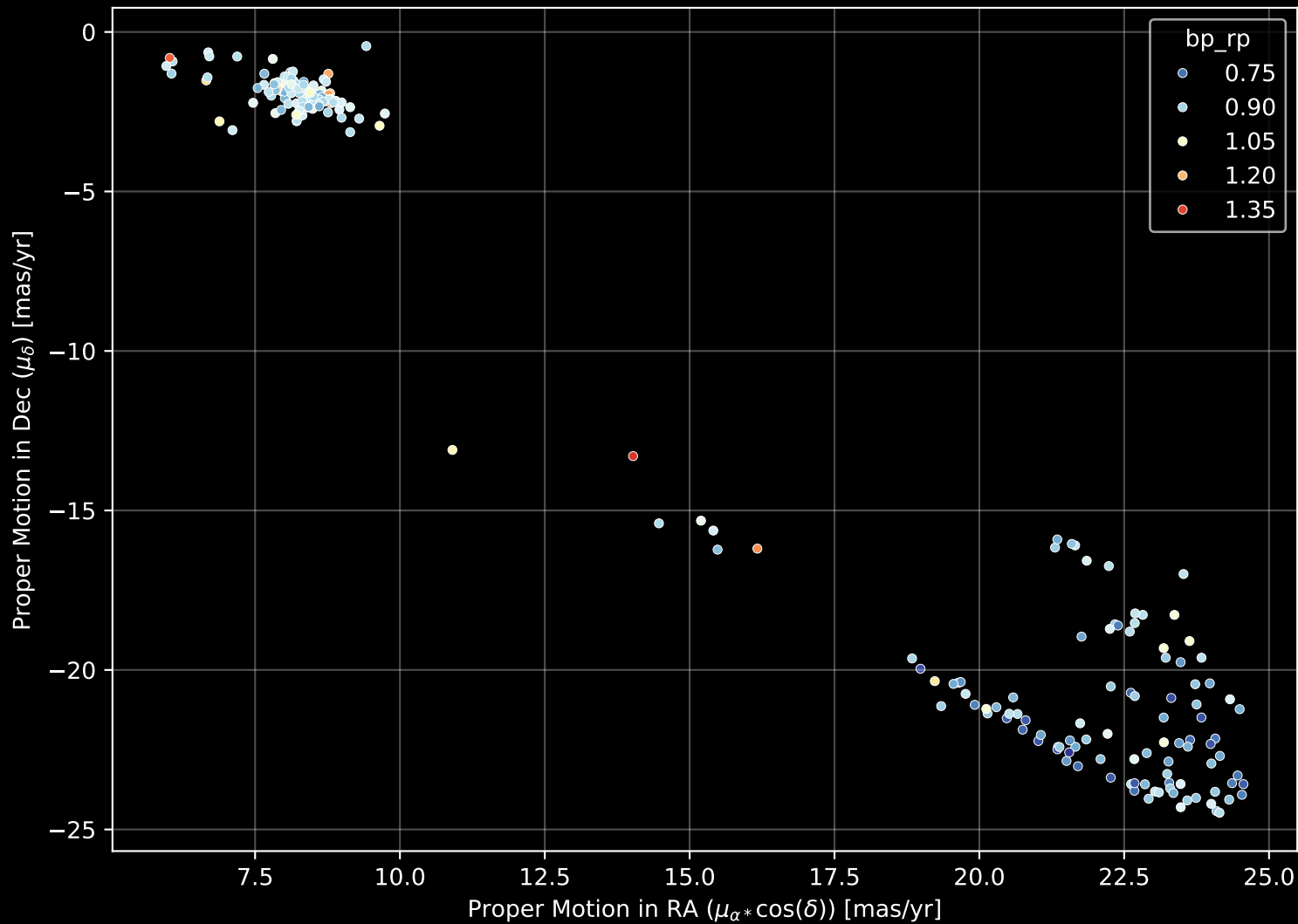
Gaia Stream: [Gjoll] Proper Motion Diagram (n= 249)
