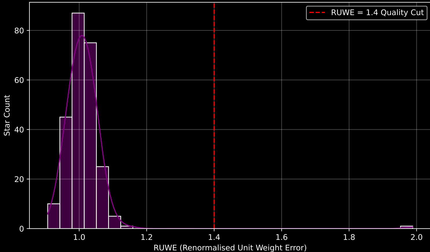
Gaia Stream: [Gjoll] RUWE Distribution (n= 249)
