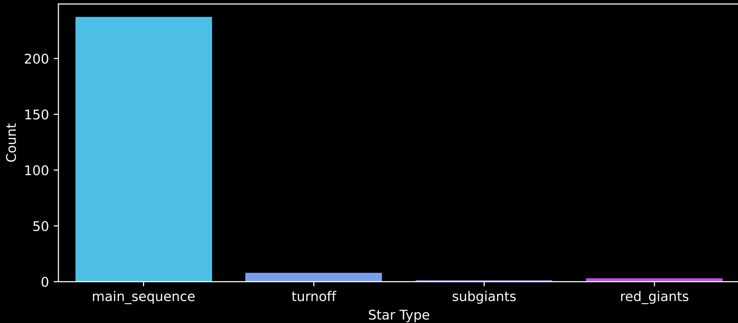
Gaia Stream: [Gjoll] Count plot of Star Type
