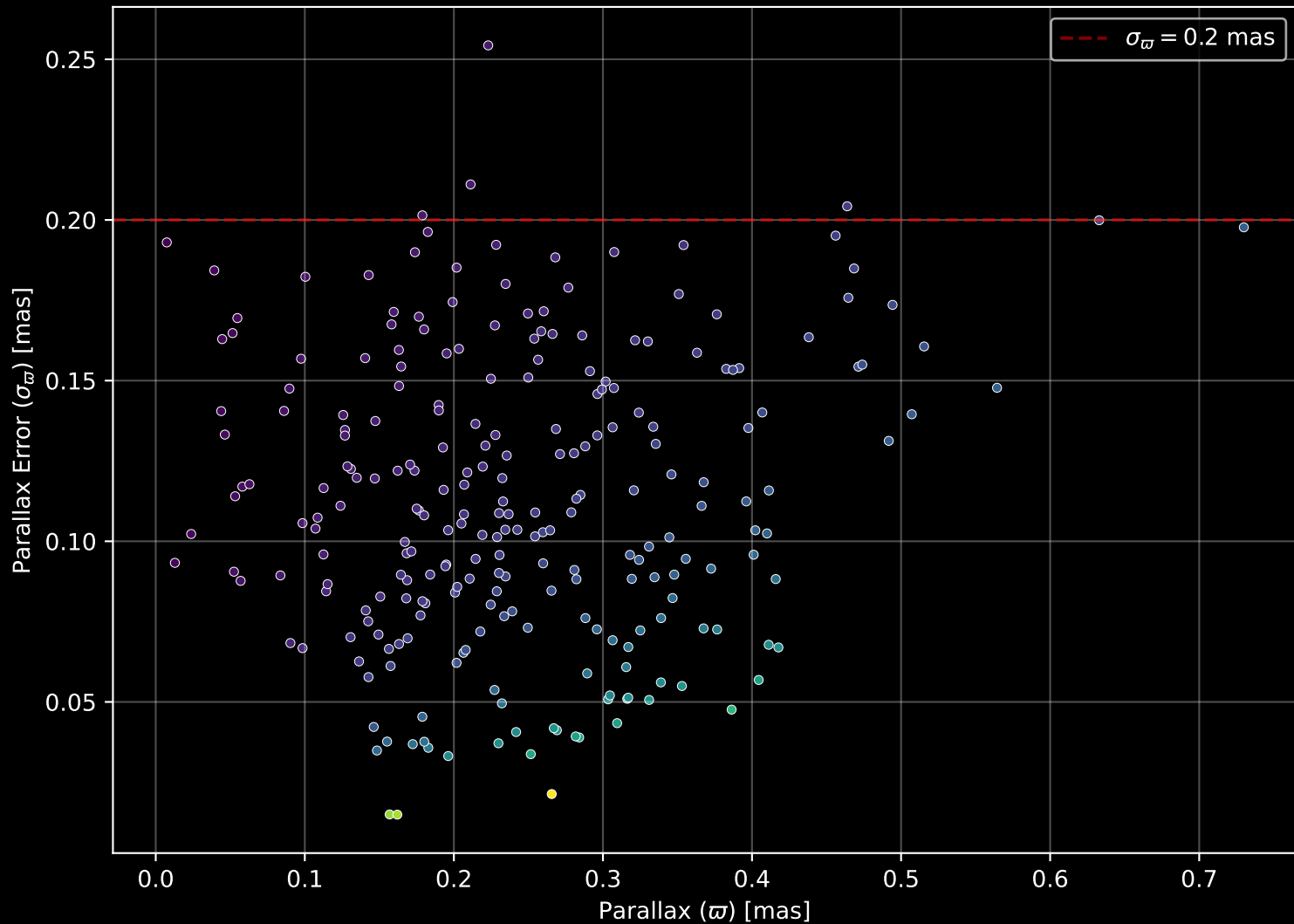
Gaia Stream: [Gjoll] Parallax Quality (n = 249)
