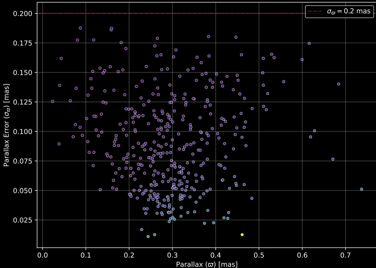
Gaia Stream: [Hrid] Parallax Quality (n= 393)
