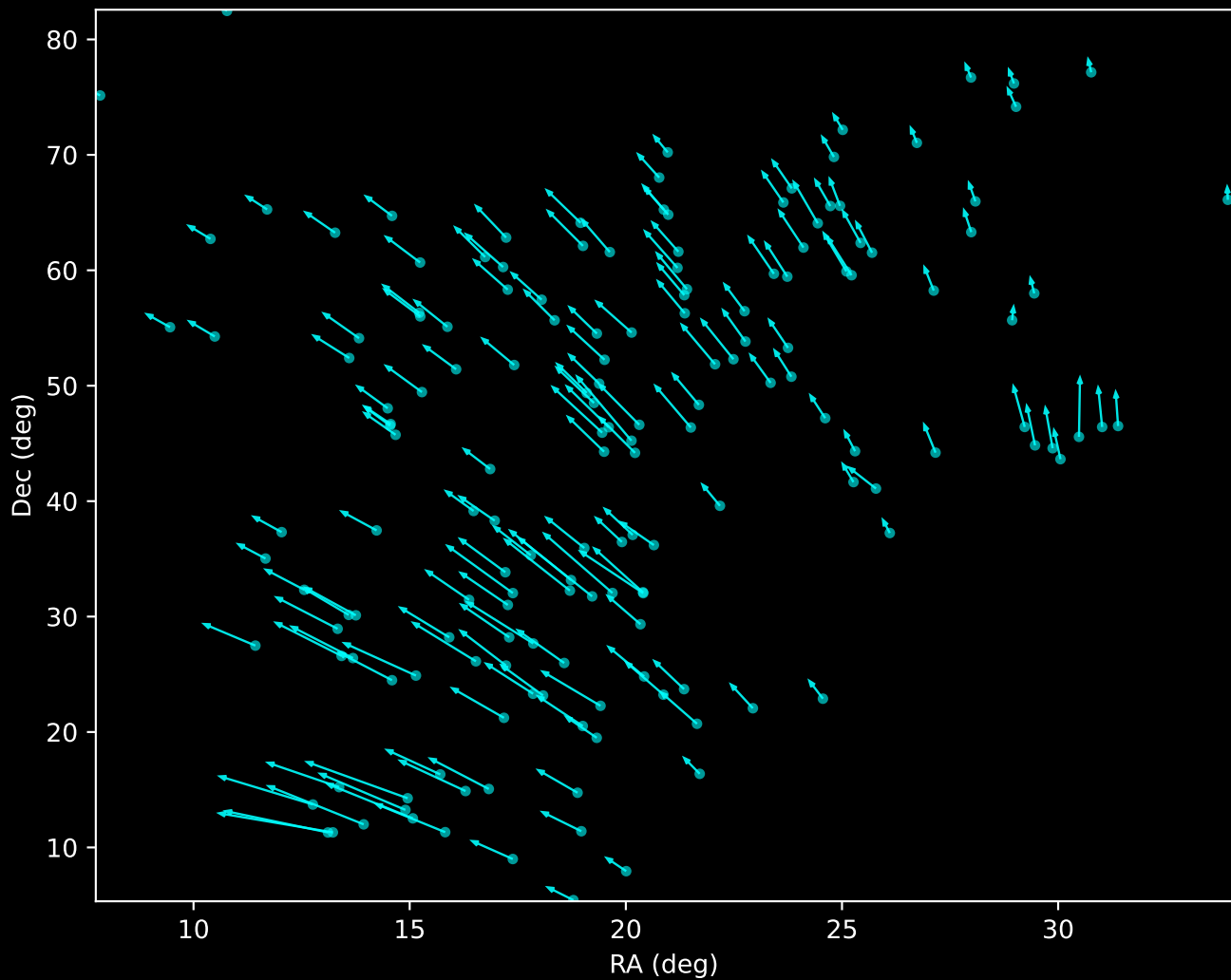
Gaia DR3 Noise Stream Proper Motion Vectors (n=166)
