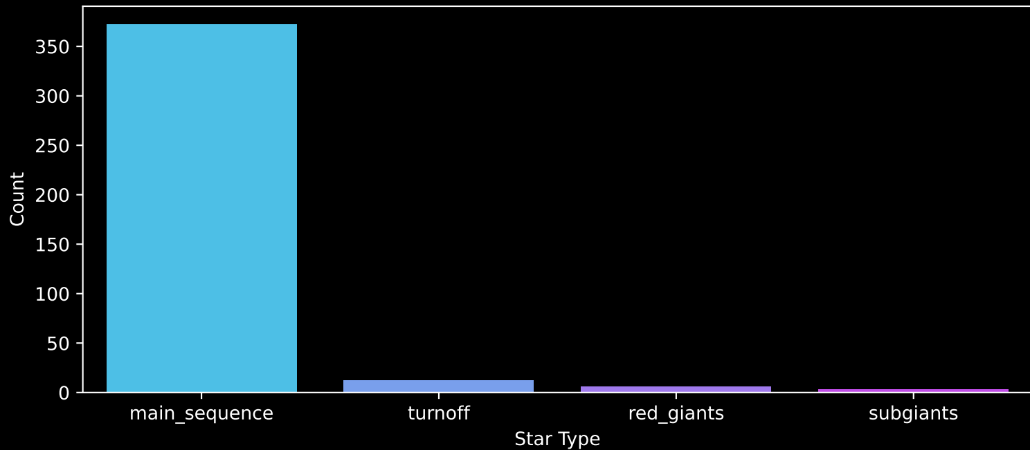
Gaia Stream: [Hrid] Count plot of Star Type
