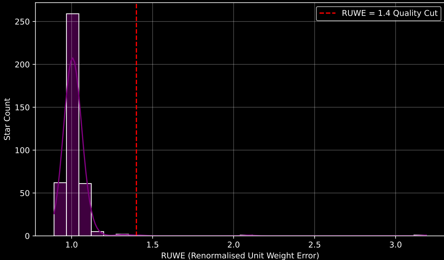
Gaia Stream: [Hrid] RUWE Distribution (n= 392)
