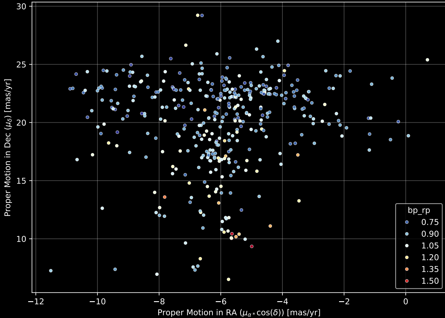
Gaia Stream: [Hrid] Proper Motion Diagram (n= 393)
