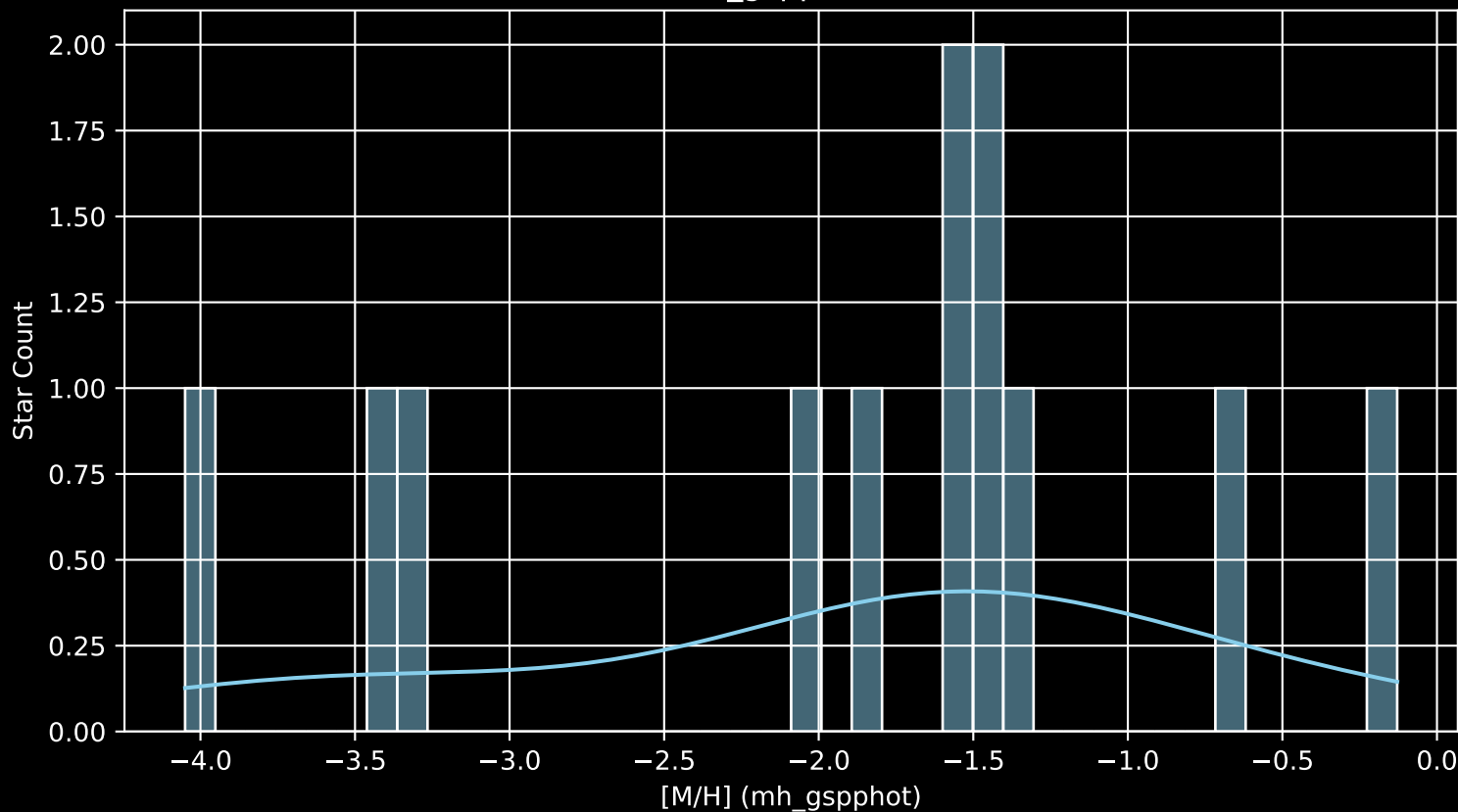
Gaia Stream: [Hydrus [M/H] (mh_gspphot) (n= 12)
