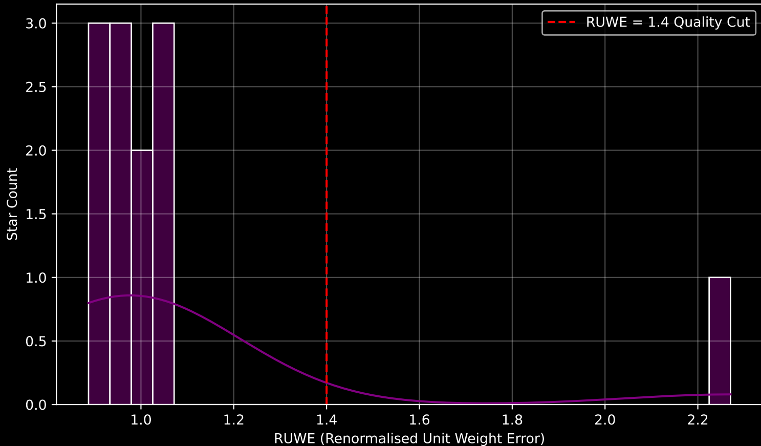
Gaia Stream: [Hydrus] RUWE Distribution (n= 12)
