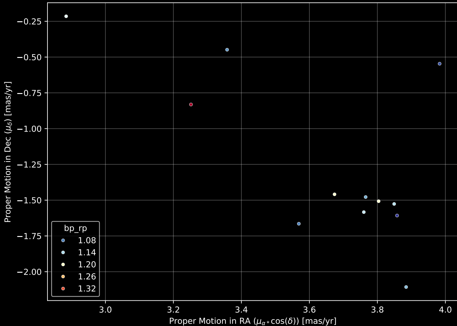
Gaia Stream: [Hydrus] Proper Motion Diagram (n= 12)
