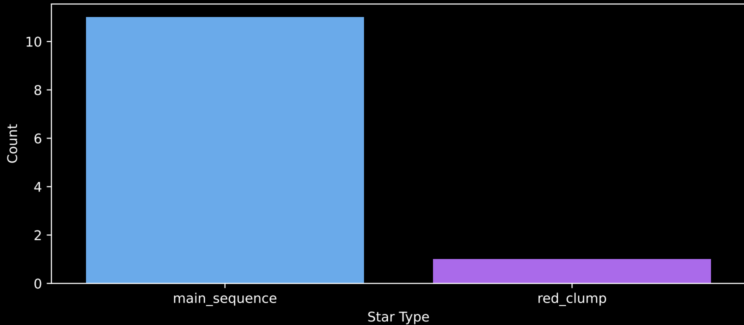
Gaia Stream: [Hydrus] Count plot of Star Type
