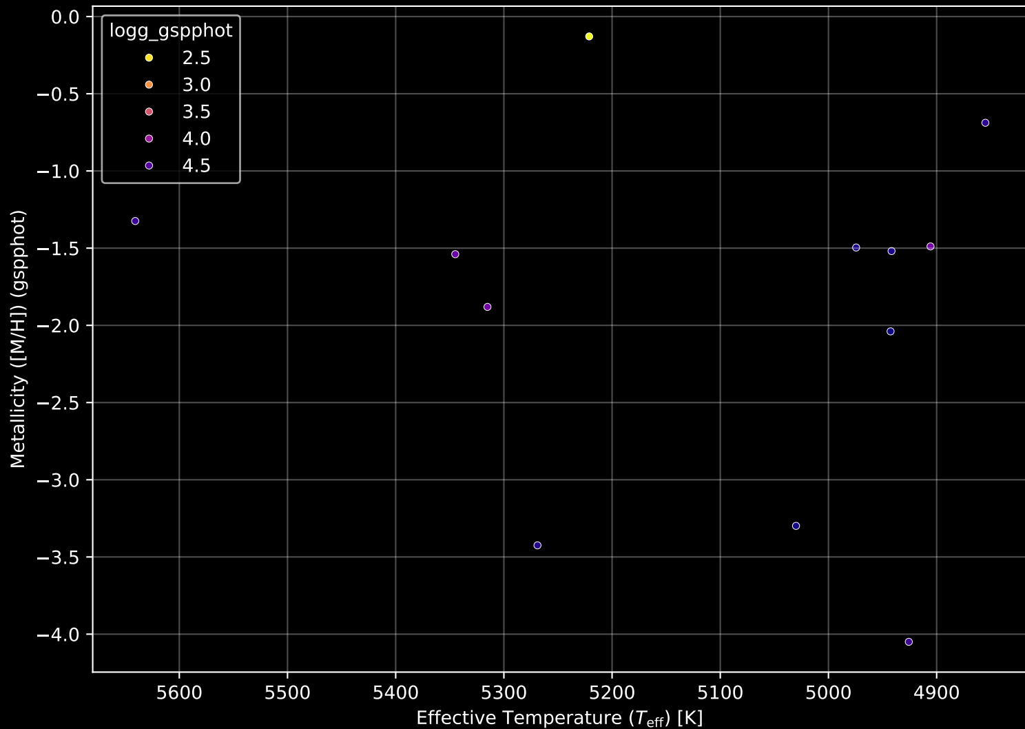
Gaia Stream: [Hydrus] Stellar Population Parameters (n= 12)
