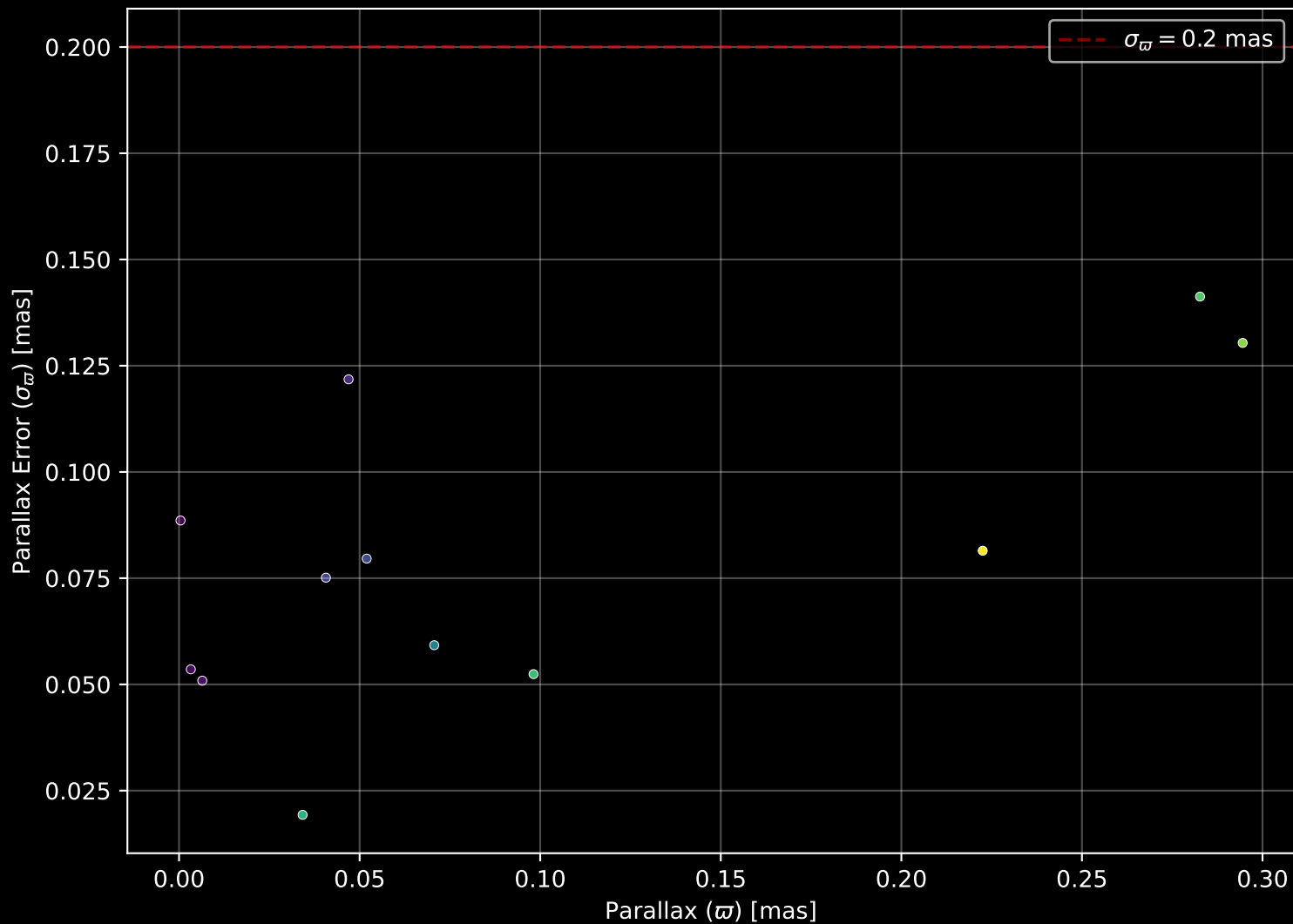
Gaia Stream: [Hydrus] Parallax Quality (n= 12)
