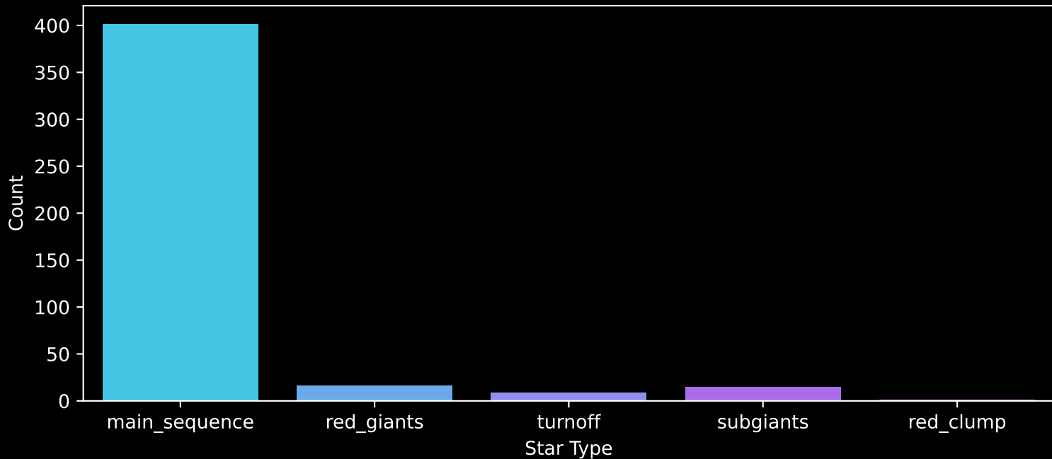
Gaia Stream: [Indus] Count plot of Star Type
