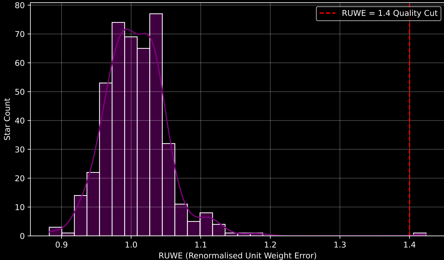
Gaia Stream: [Indus] RUWE Distribution (n= 442)
