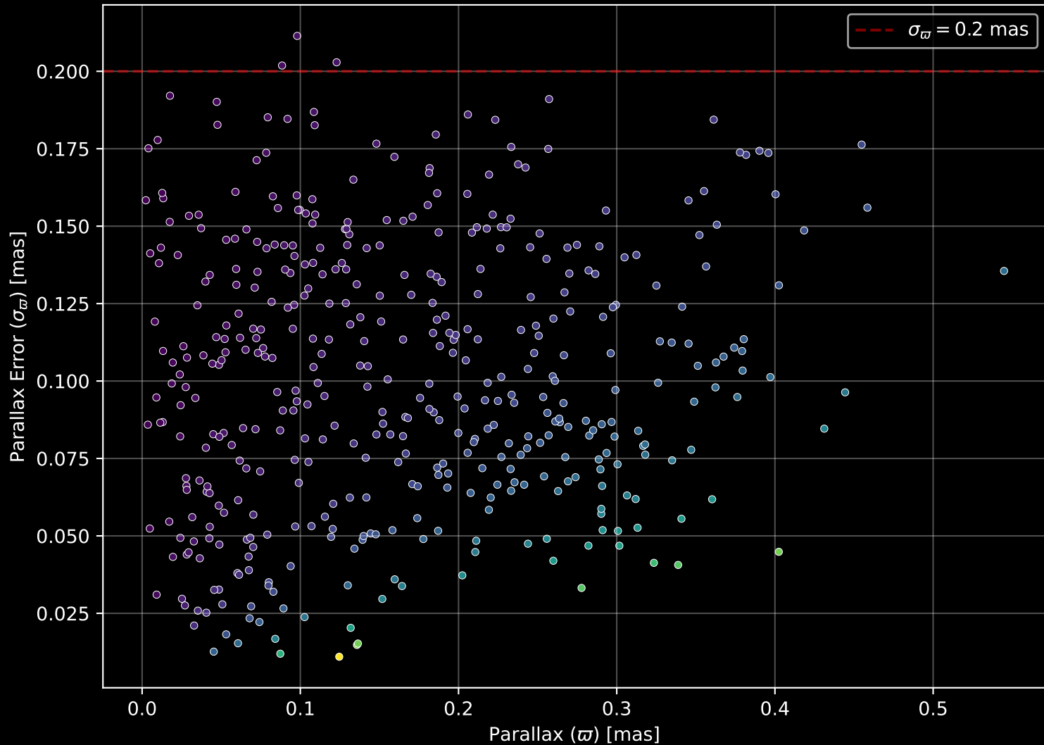
Gaia Stream: [Indus] Parallax Quality (n= 442)
