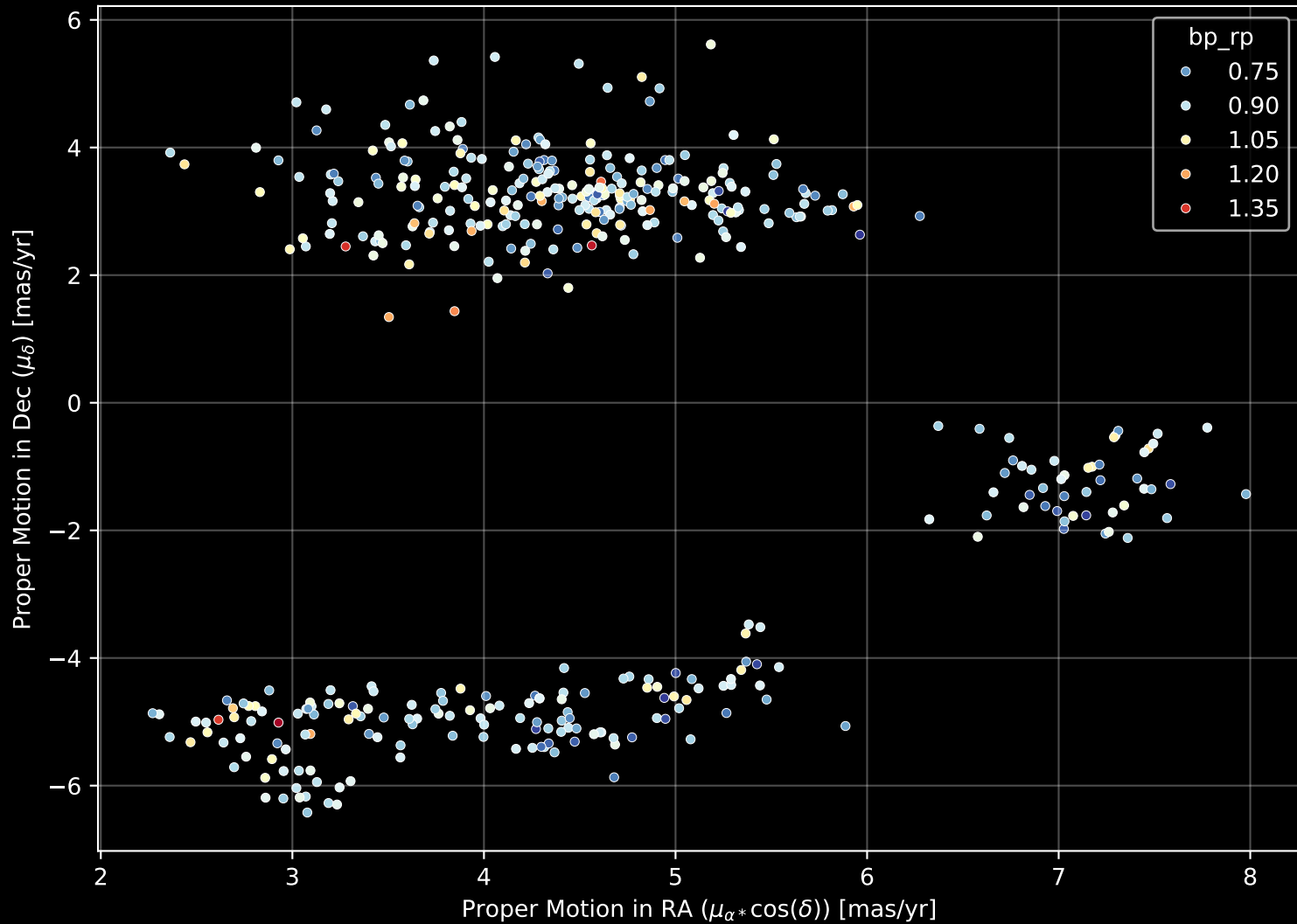
Gaia Stream: [Indus] Proper Motion Diagram (n= 442)
