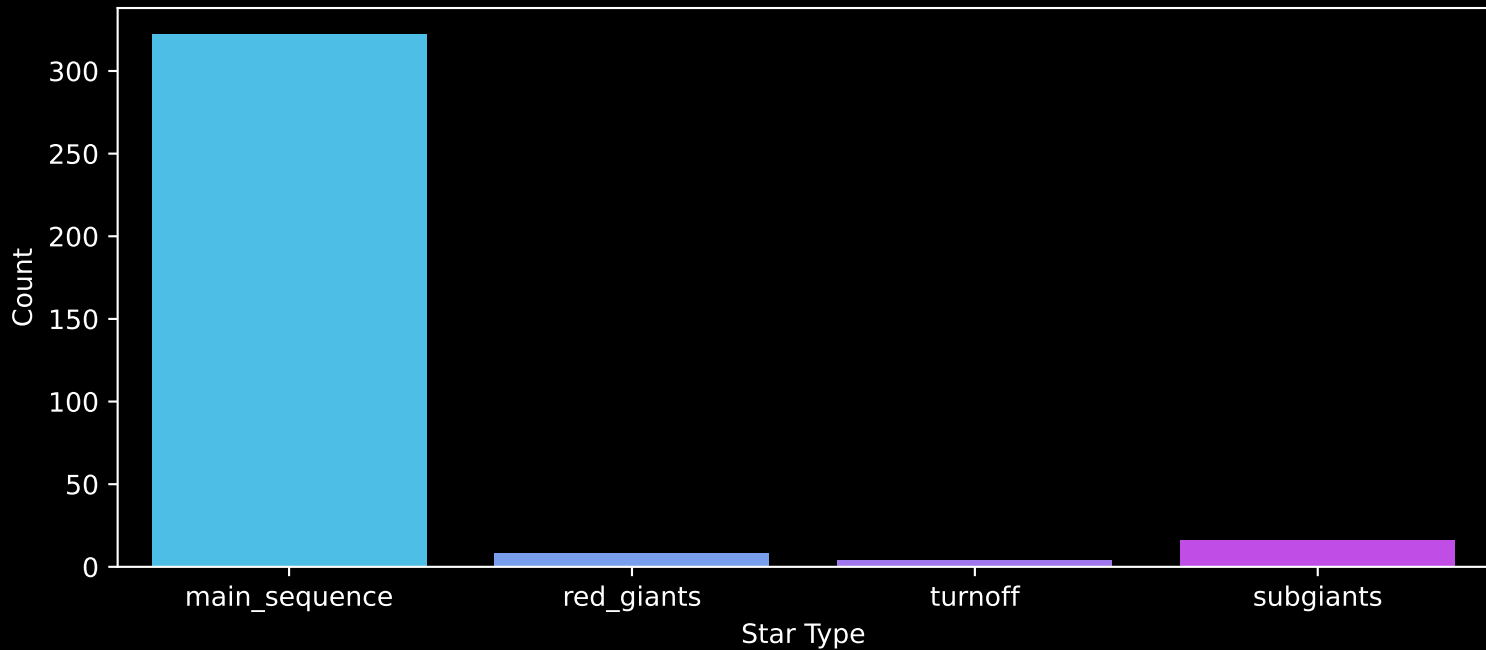
Gaia Stream: [Jhelum] Count plot of Star Type
