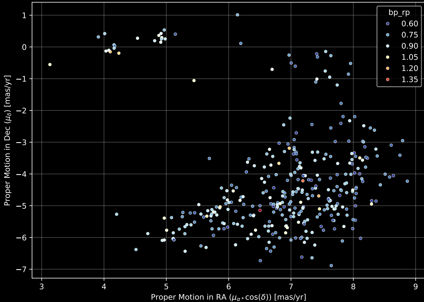
Gaia Stream: [Jhelum] Proper Motion Diagram (n= 350)
