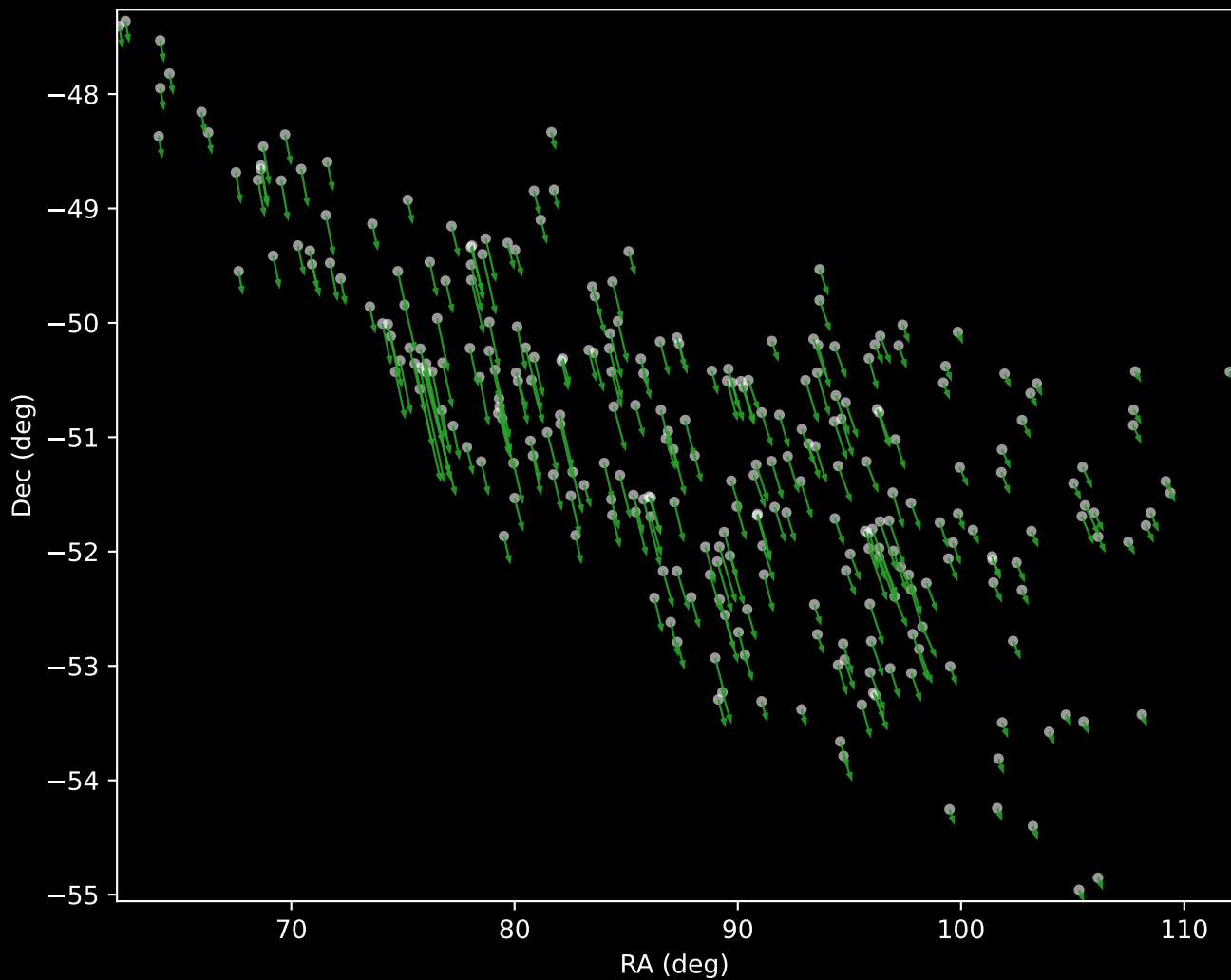
Gaia DR3 Cluster 4 Proper Motion Vectors (n=284)
