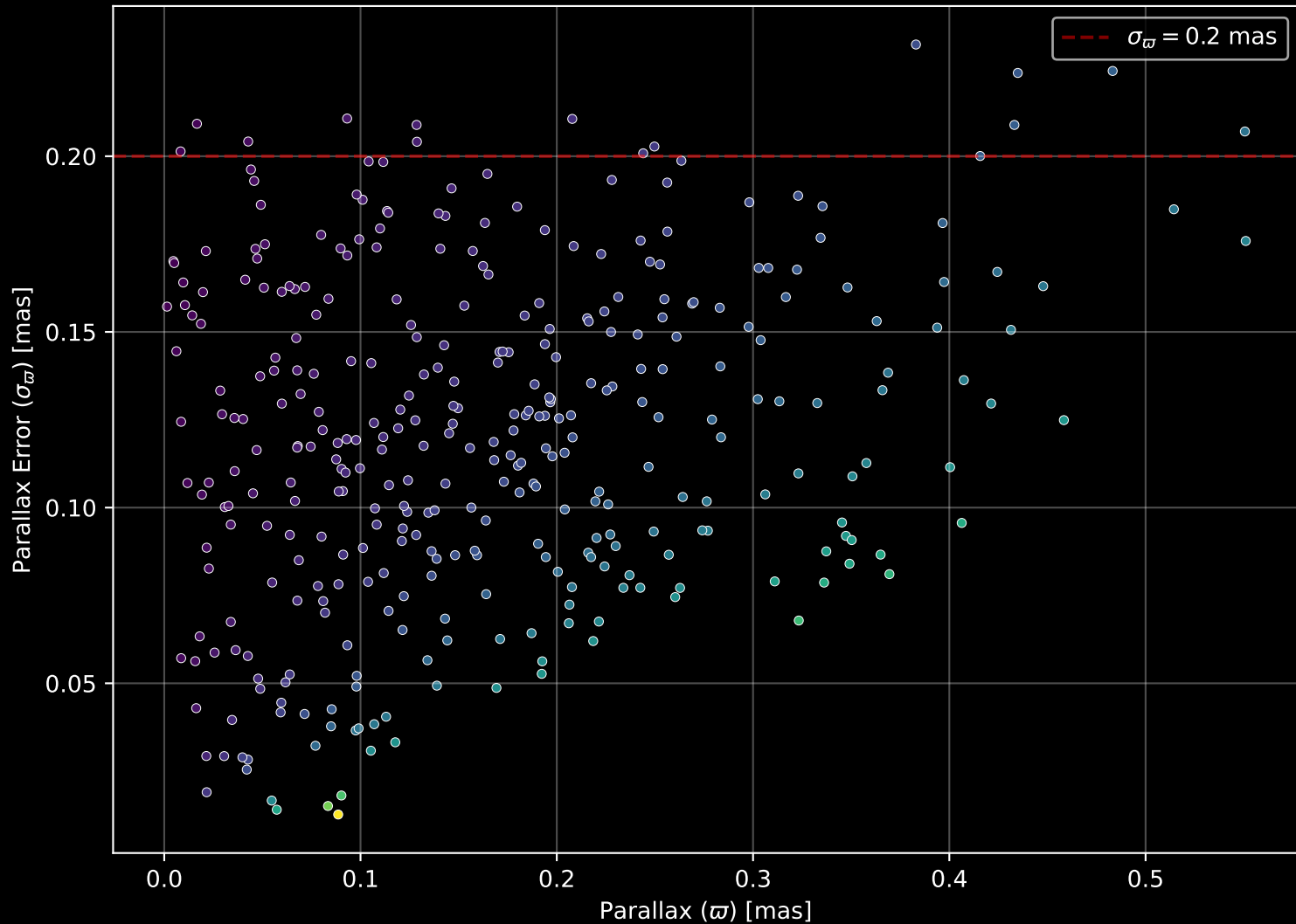
Gaia Stream: [Jhelum] Parallax Quality (n= 350)
