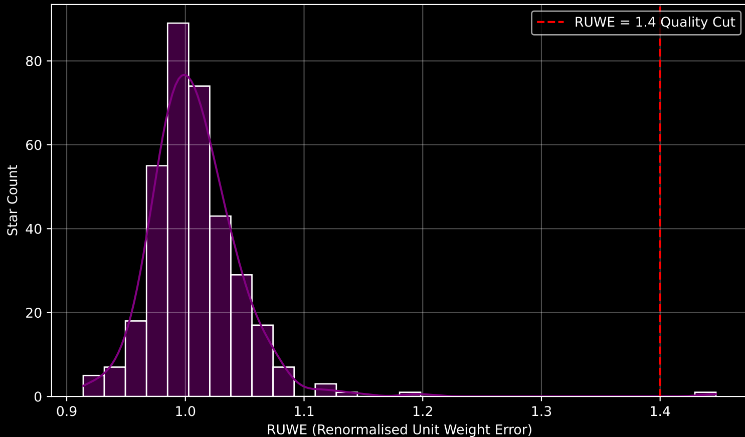
Gaia Stream: [Jhelum] RUWE Distribution (n= 350)
