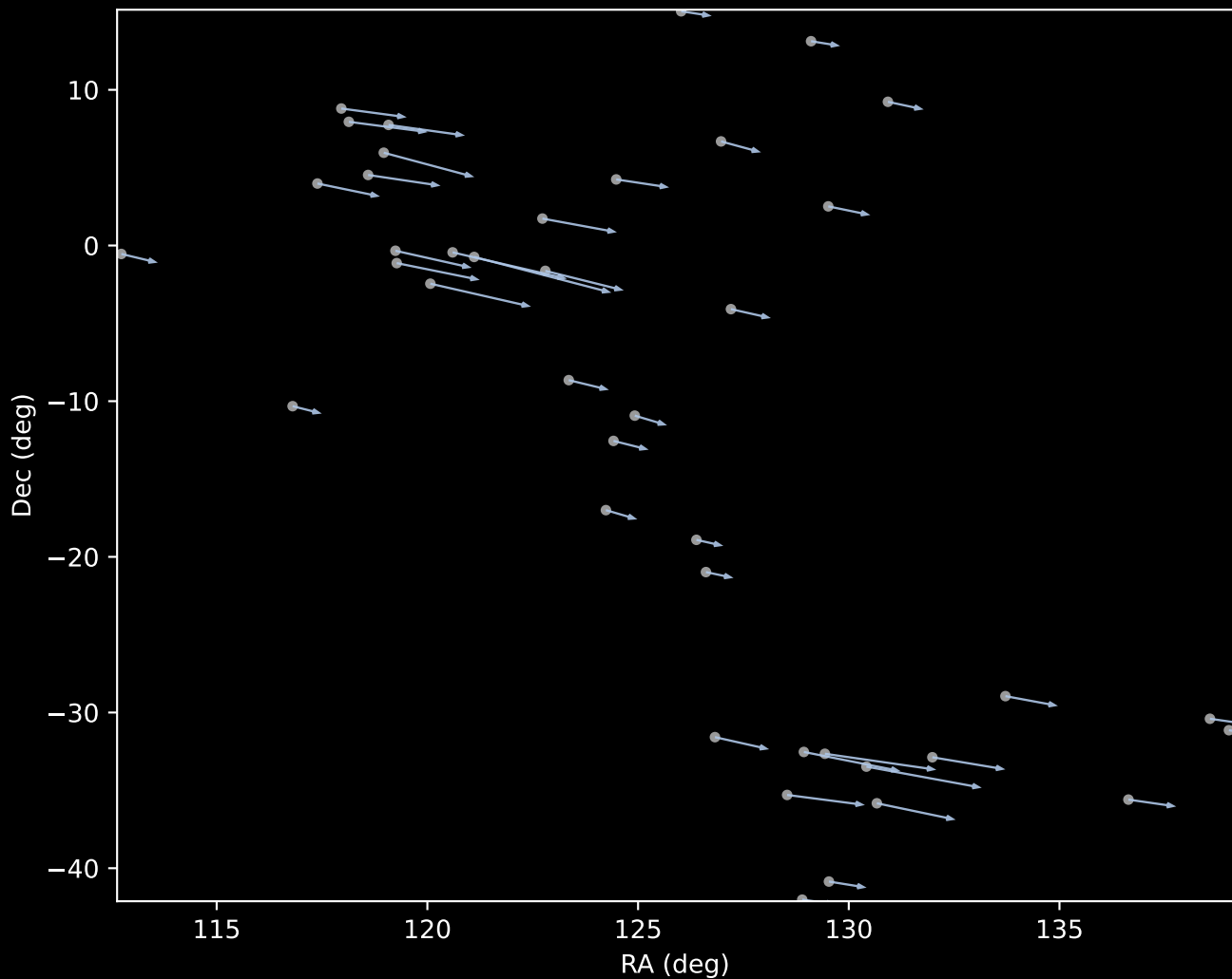
Gaia DR3 Cluster 1 Proper Motion Vectors (n=41)
