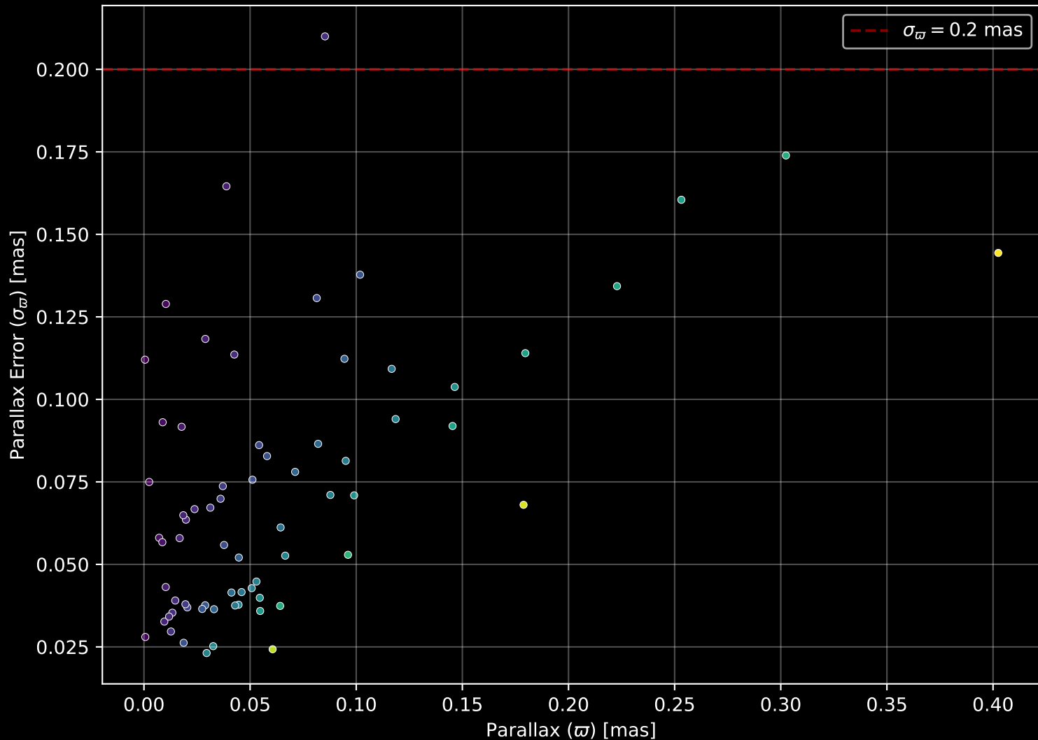
Gaia Stream: [Kwando] Parallax Quality (n= 69)
