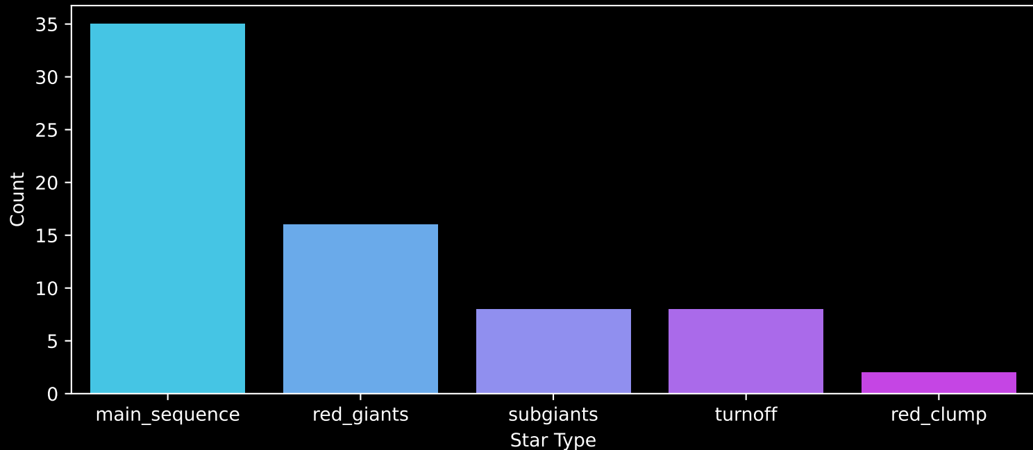
Gaia Stream: [Kwando] Count plot of Star Type
