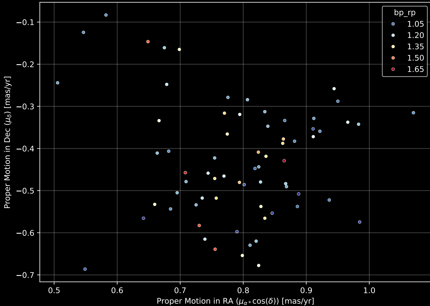
Gaia Stream: [Kwando] Proper Motion Diagram (n= 69)
