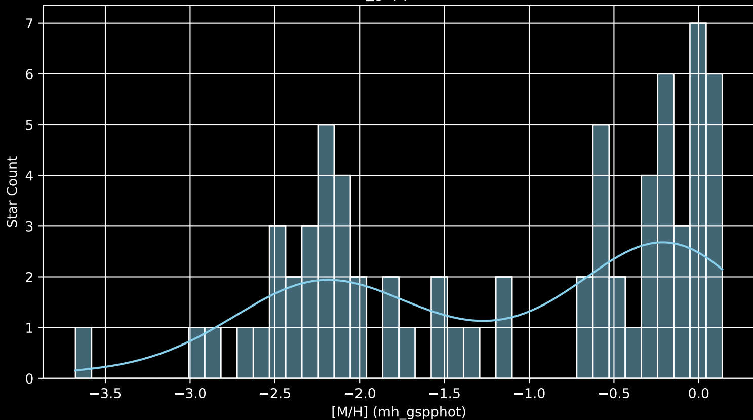
Gaia Stream: [Kwando [M/H] (mh_gspphot) (n= 69)
