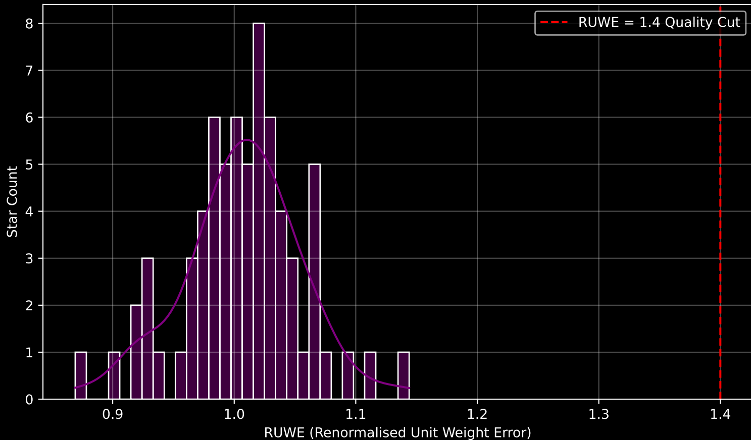
Gaia Stream: [Kwando] RUWE Distribution (n= 69)
