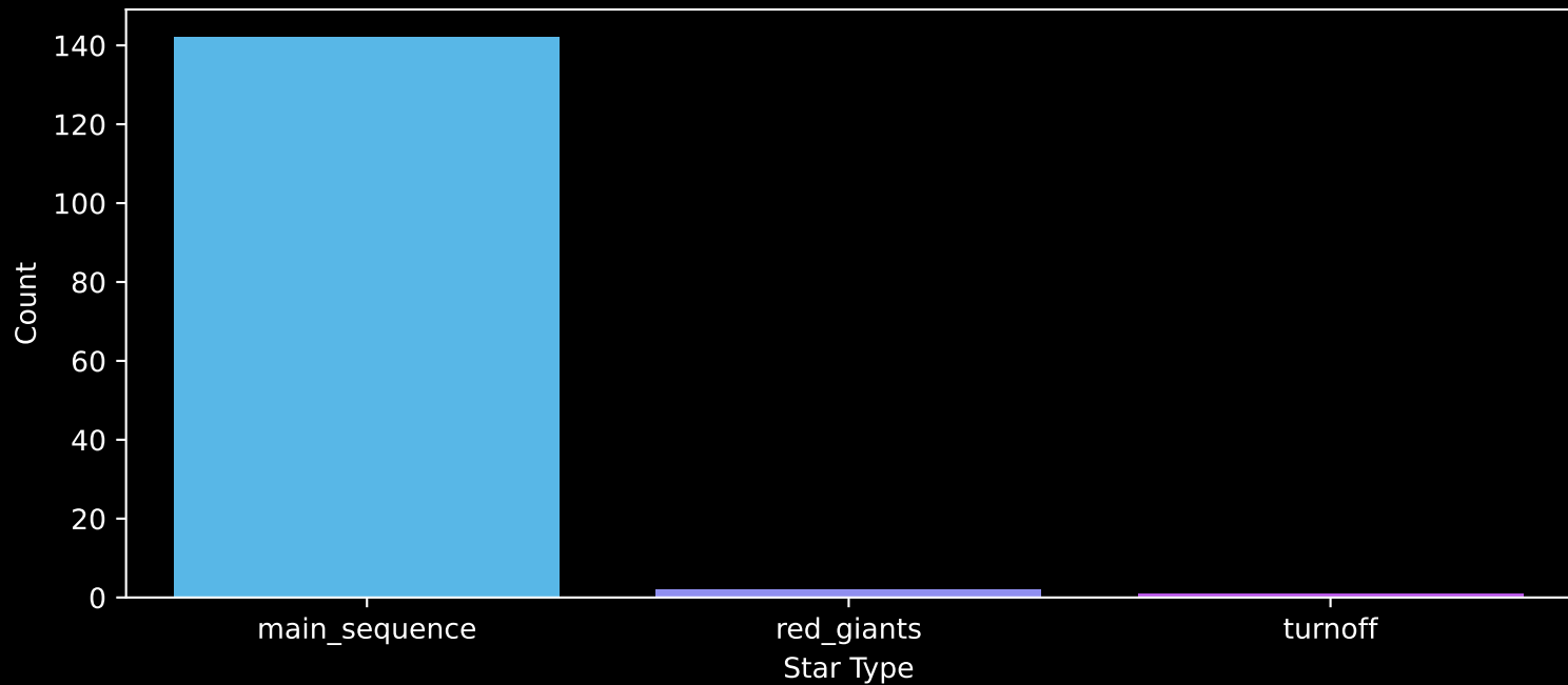
Gaia Stream: [Leiptr] Count plot of Star Type
