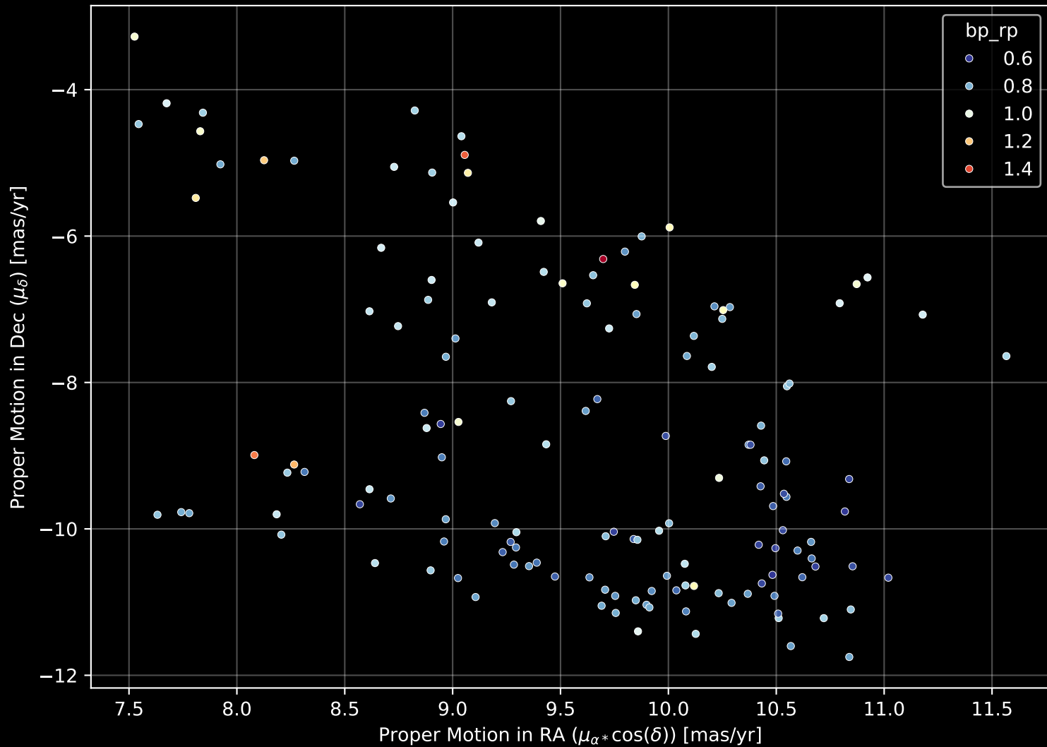
Gaia Stream: [Leiptr] Proper Motion Diagram (n= 145)
