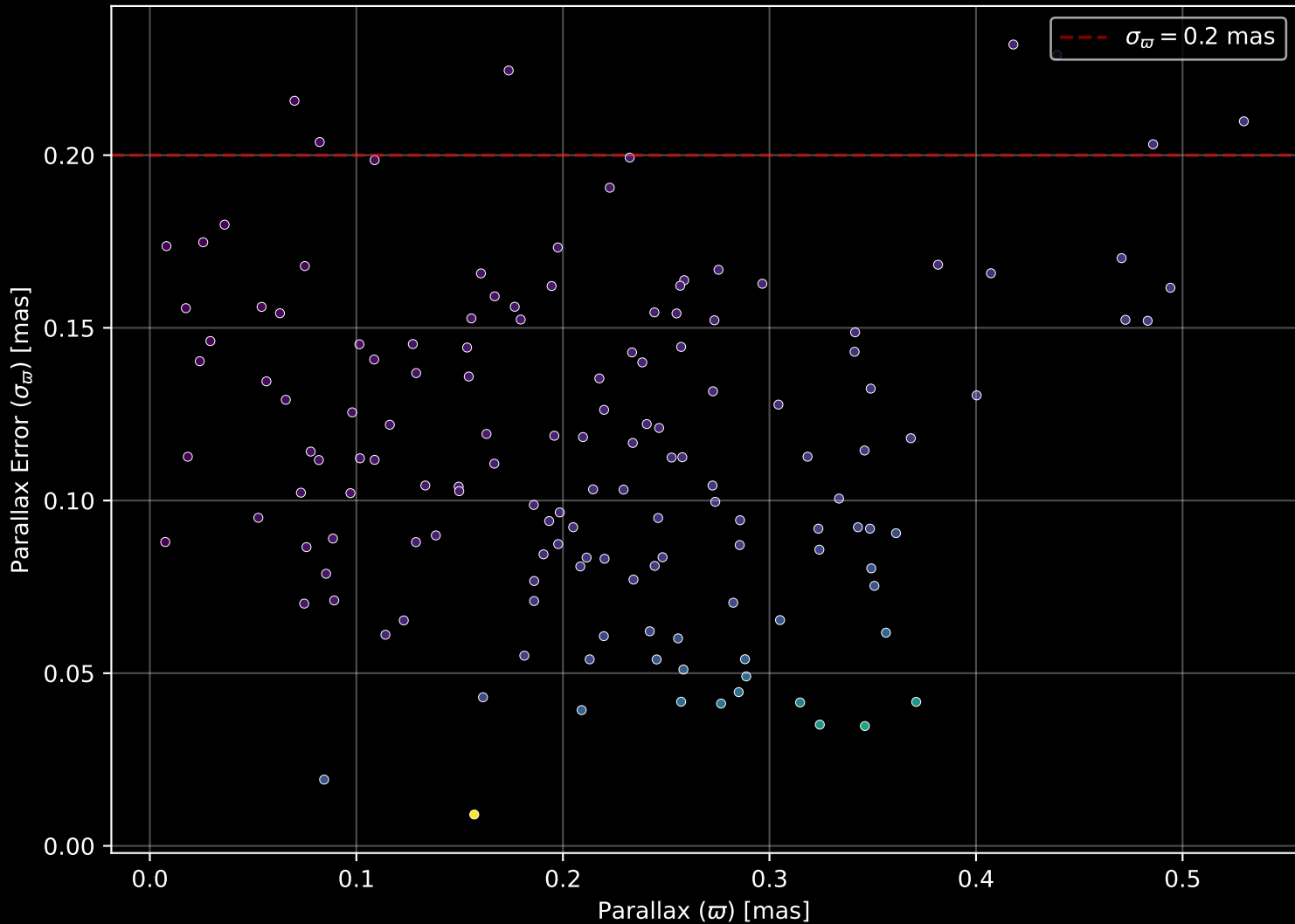
Gaia Stream: [Leiptr] Parallax Quality (n= 145)
