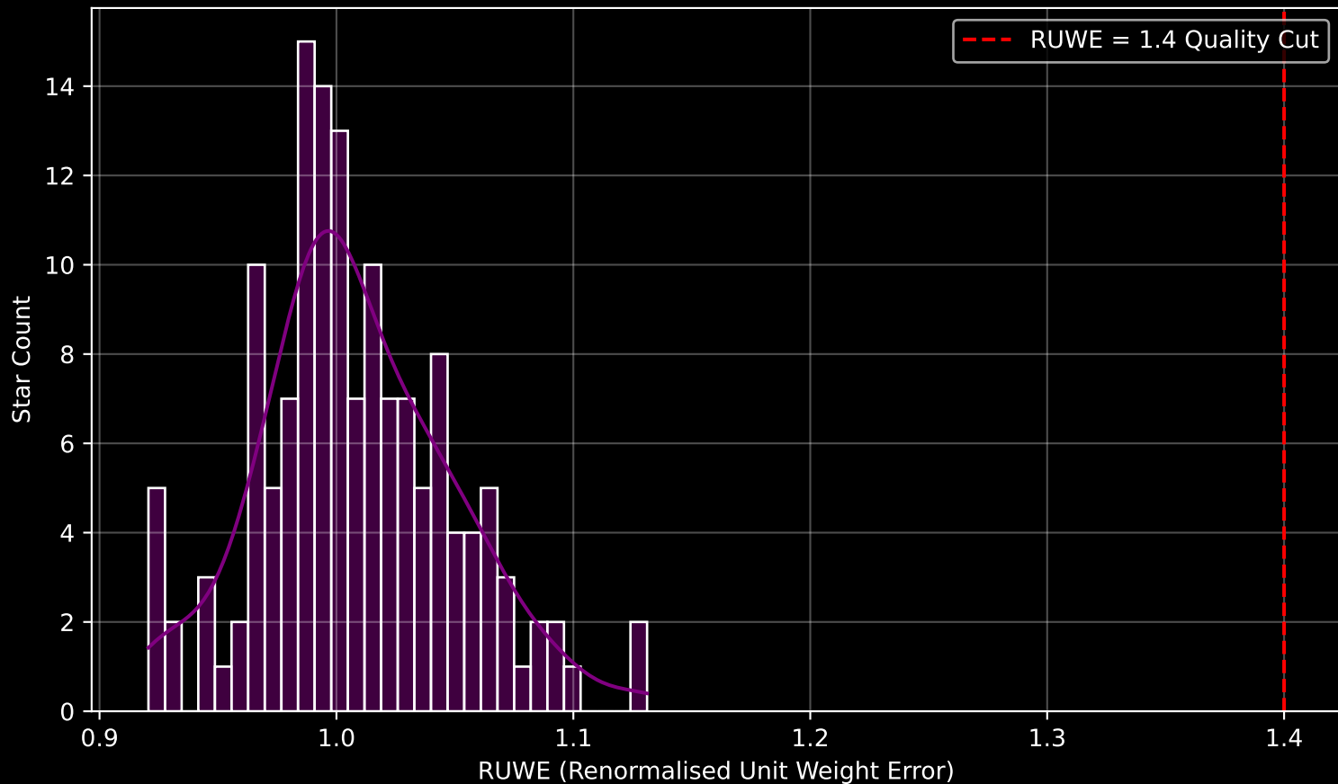
Gaia Stream: [Leiptr] RUWE Distribution (n= 145)
