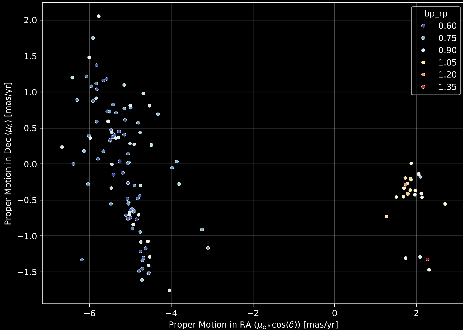
Gaia Stream: [M92] Proper Motion Diagram (n= 128)
