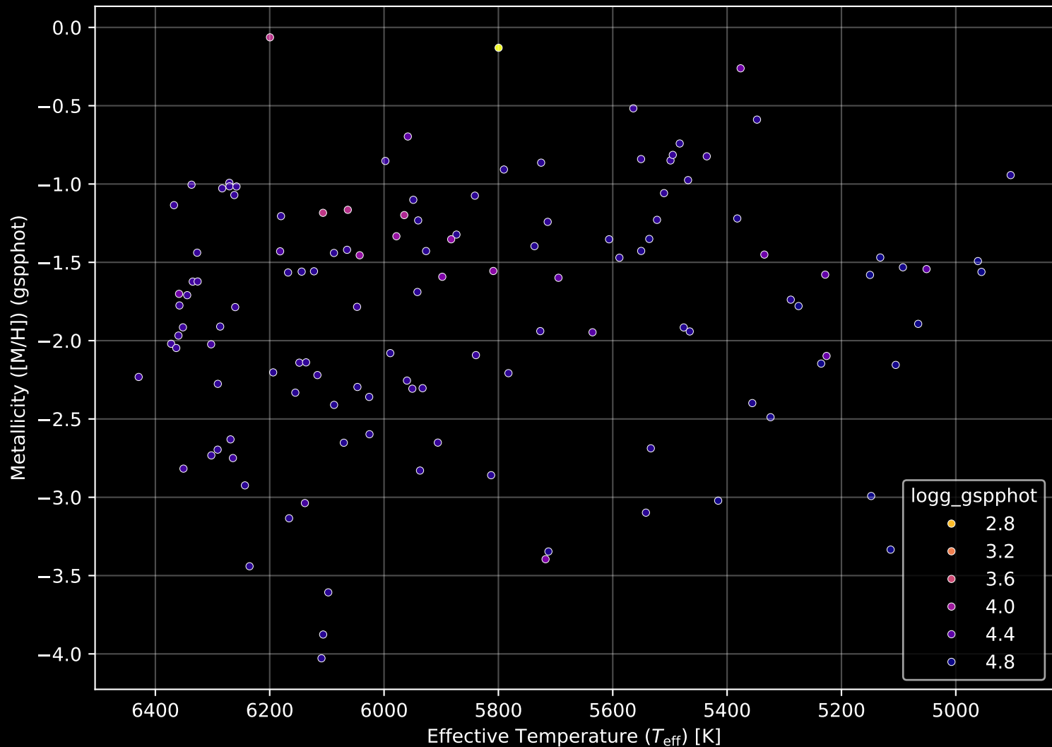
Gaia Stream: [M92] Stellar Population Parameters (n= 128)
