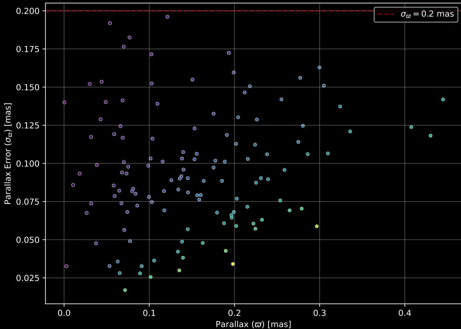
Gaia Stream: [M92] Parallax Quality (n= 128)
