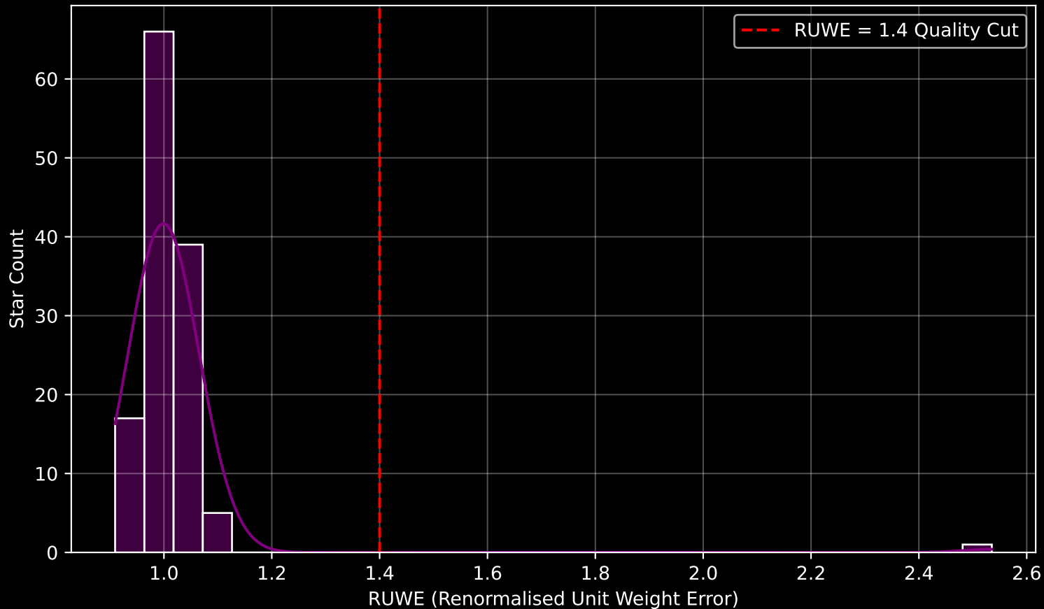
Gaia Stream: [M92] RUWE Distribution (n= 128)
