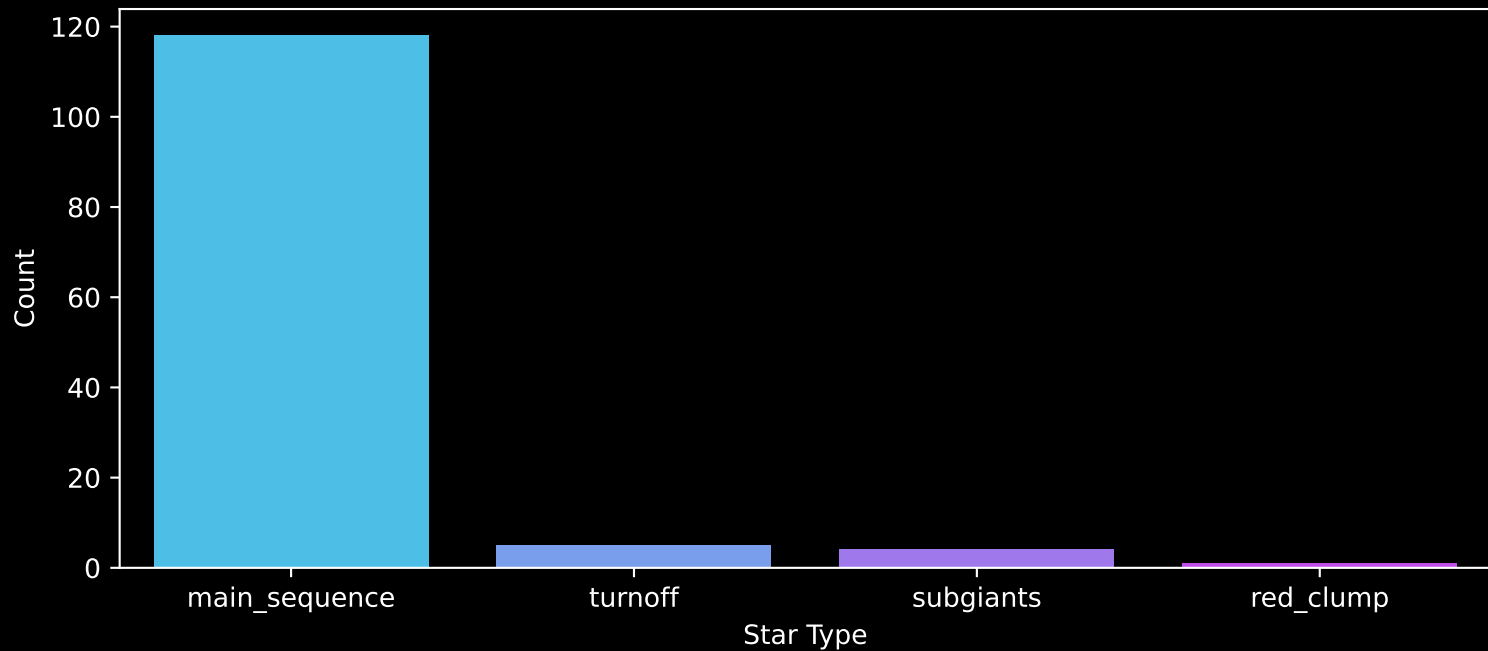
Gaia Stream: [M92] Count plot of Star Type
