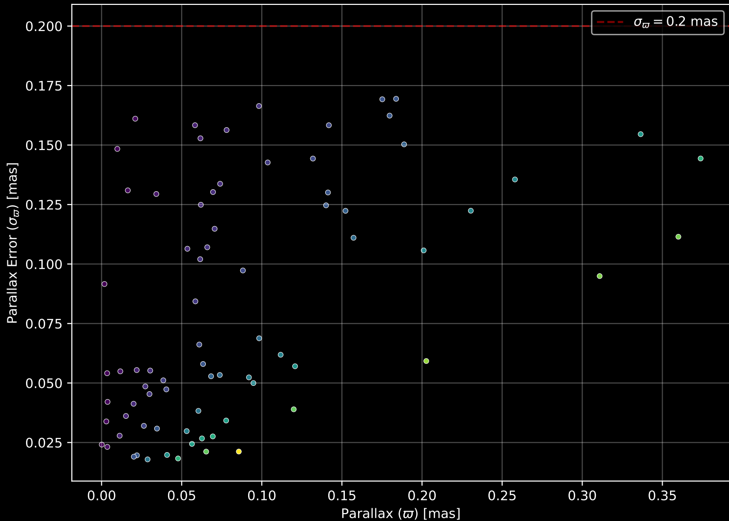
Gaia Stream: [NGC1261] Parallax Quality (n= 77)
