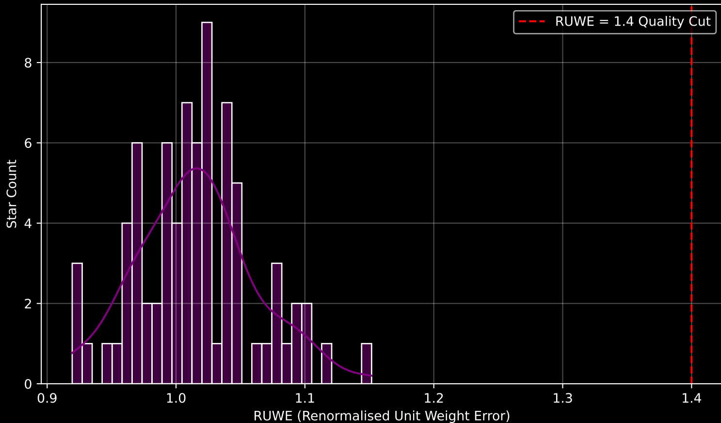
Gaia Stream: [NGC1261] RUWE Distribution (n= 77)
