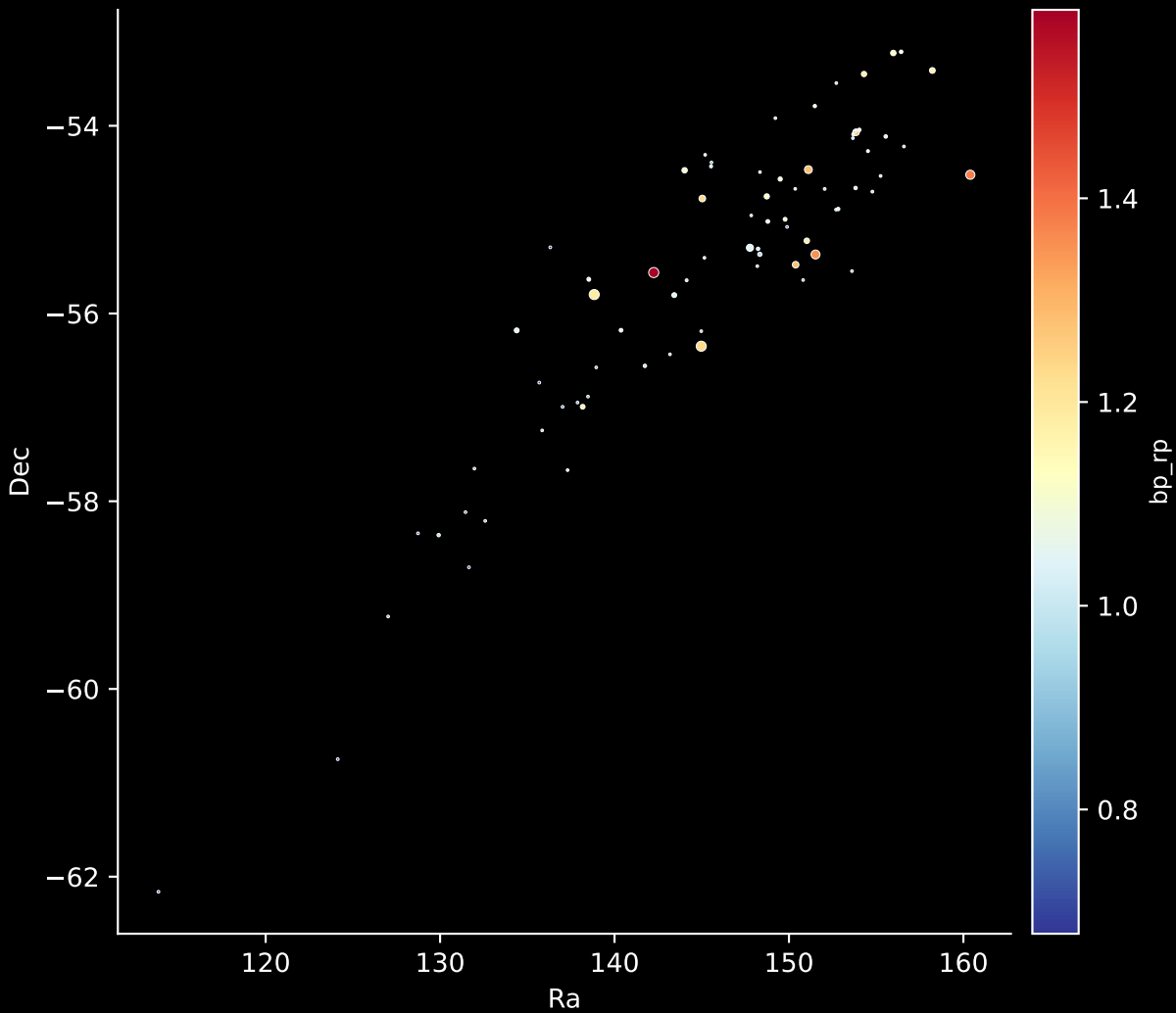
Gaia Stream: [NGC1261] Stars: 77
