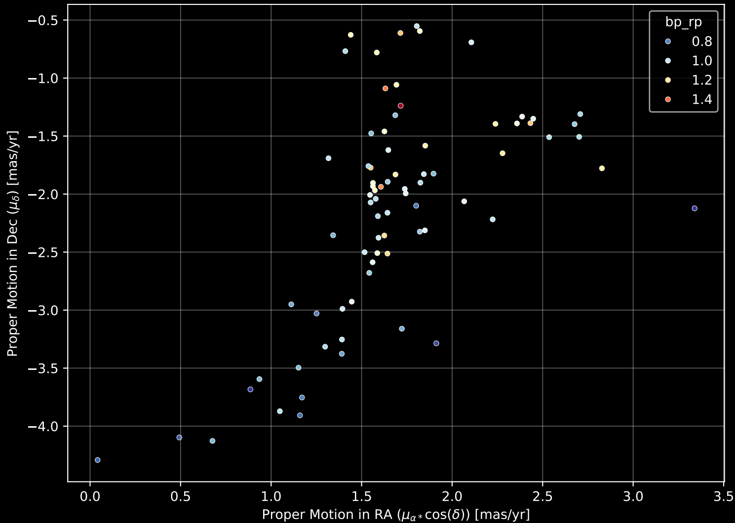
Gaia Stream: [NGC1261] Proper Motion Diagram (n= 77)
