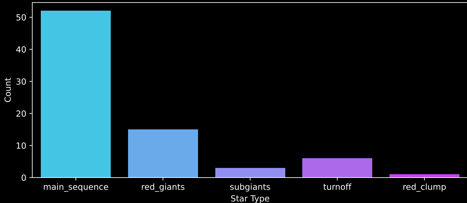
Gaia Stream: [NGC1261] Count plot of Star Type
