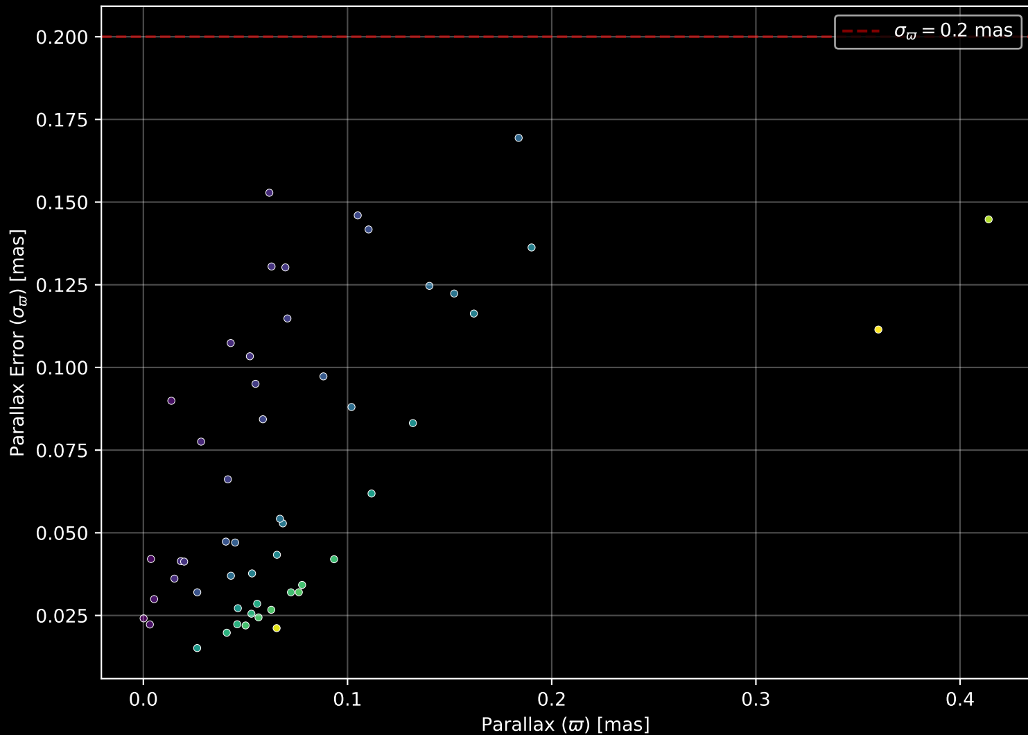
Gaia Stream: [NGC1261a] Parallax Quality (n= 53)
