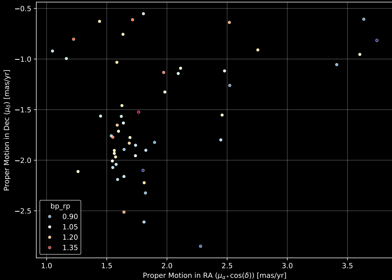
Gaia Stream: [NGC1261a] Proper Motion Diagram (n= 53)
