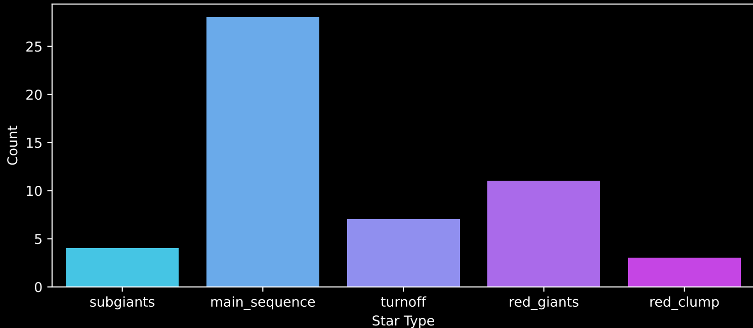
Gaia Stream: [NGC1261a] Count plot of Star Type
