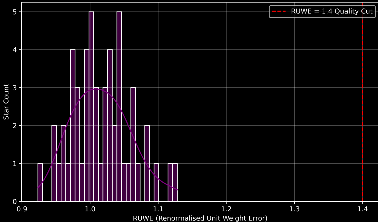
Gaia Stream: [NGC1261a] RUWE Distribution (n= 53)
