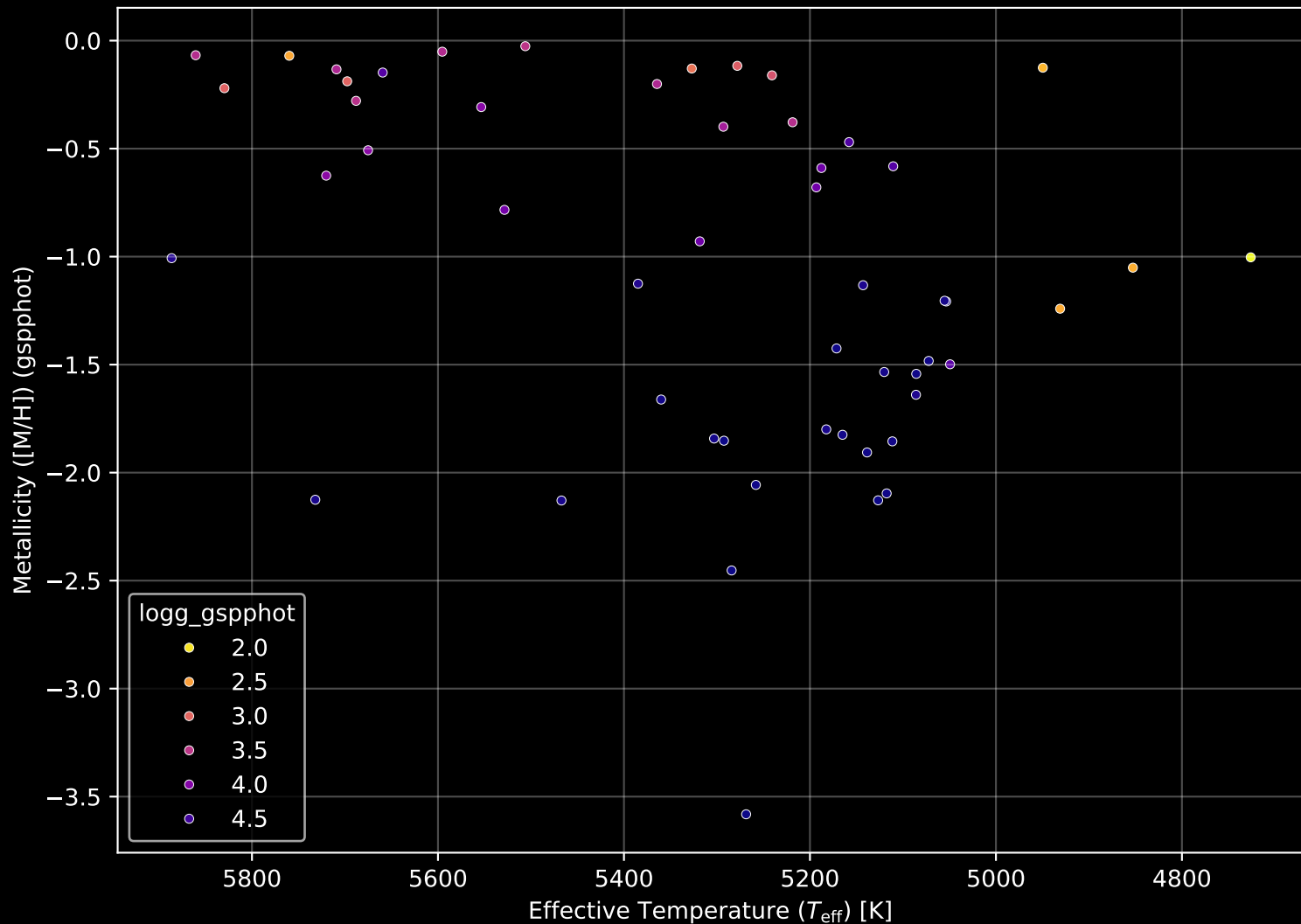
Gaia Stream: [NGC1261a] Stellar Population Parameters (n= 53)
