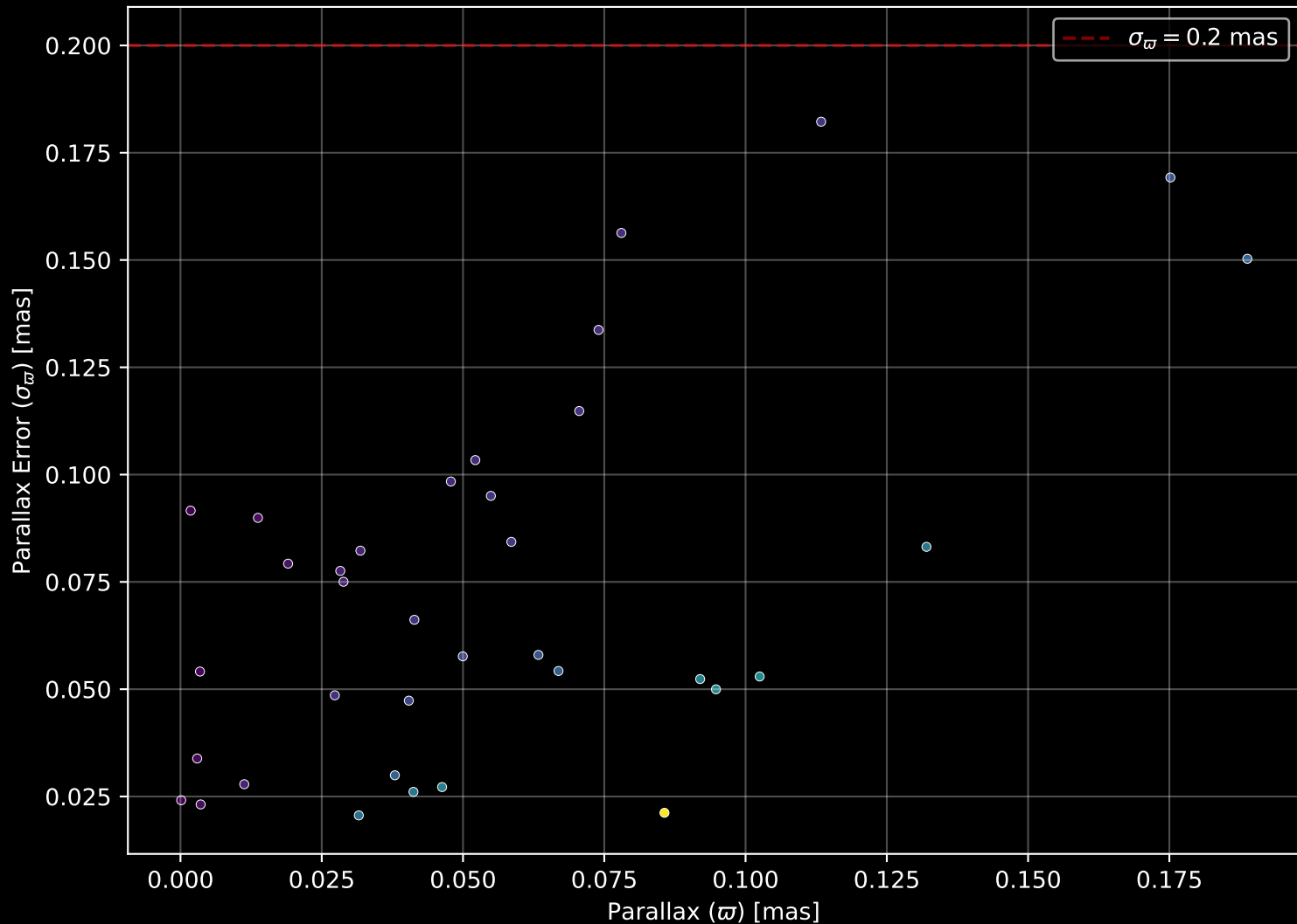
Gaia Stream: [NGC1261b] Parallax Quality (n= 36)
