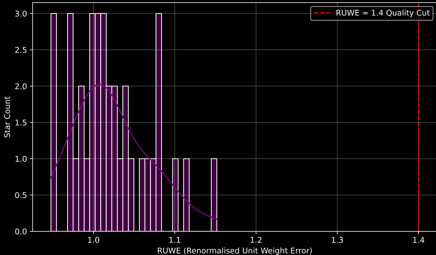
Gaia Stream: [NGC1261b] RUWE Distribution (n= 36)
