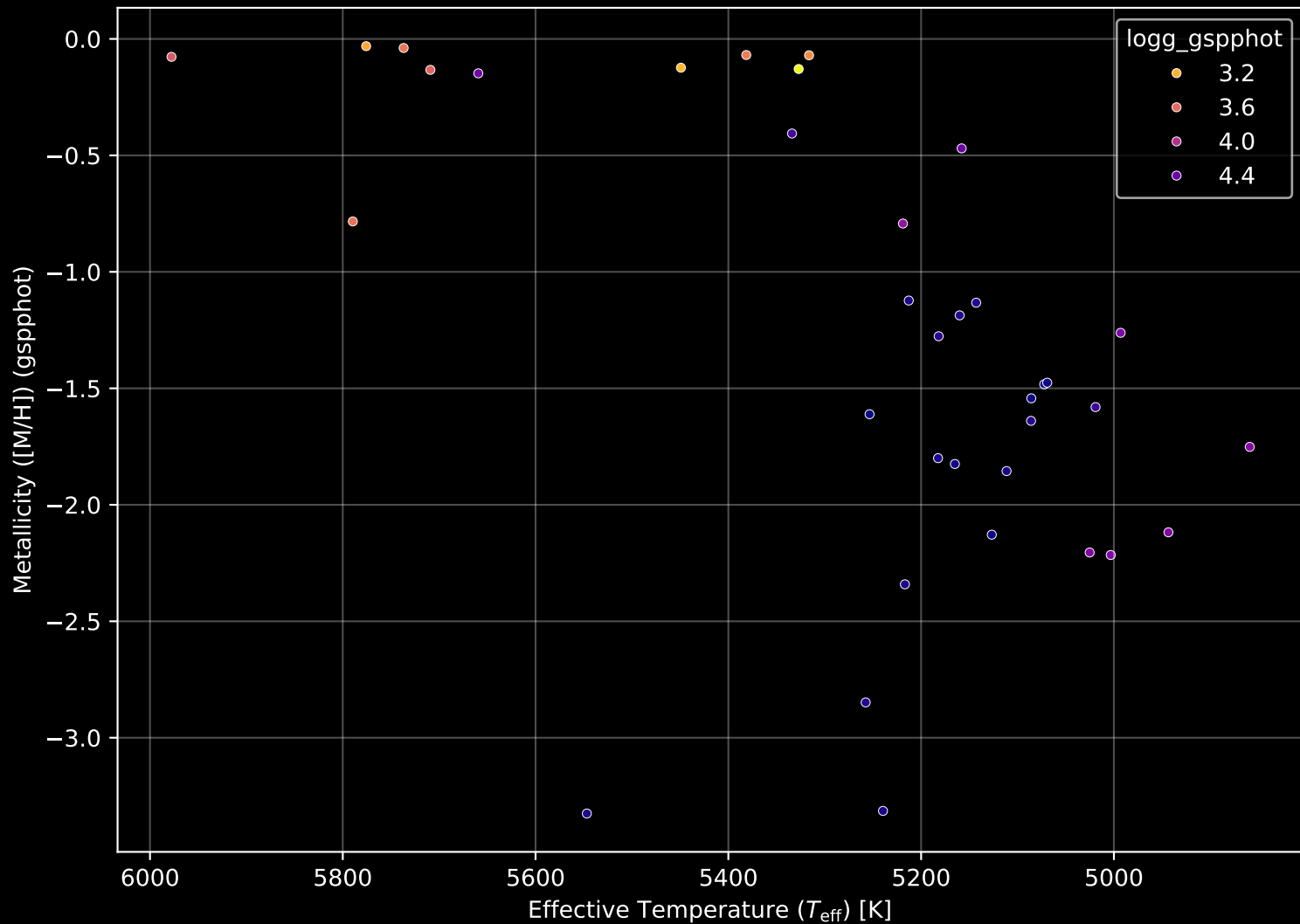
Gaia Stream: [NGC1261b] Stellar Population Parameters (n= 36)
