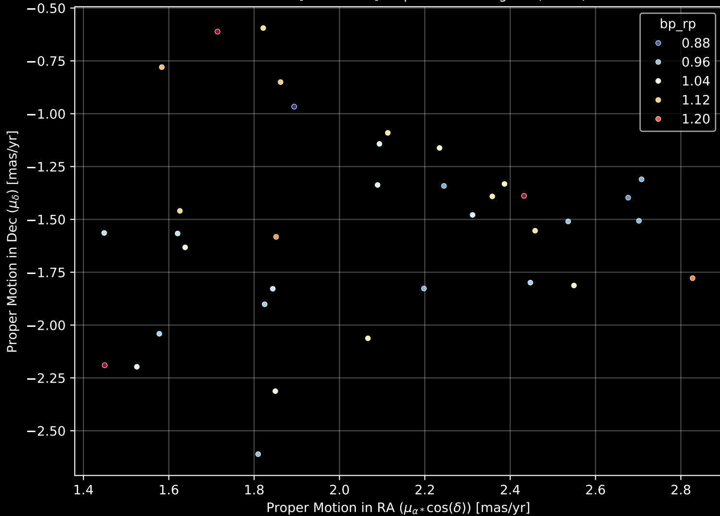
Gaia Stream: [NGC1261b] Proper Motion Diagram (n= 36)
