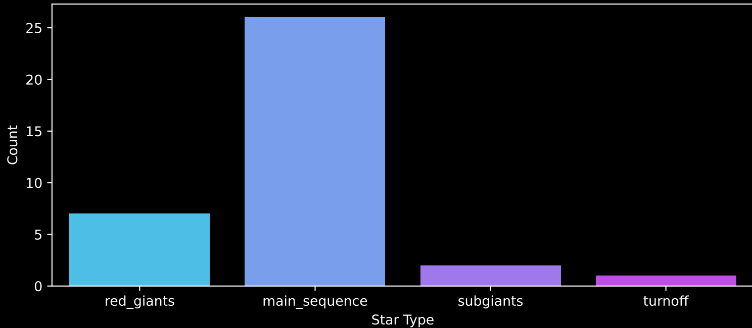
Gaia Stream: [NGC1261b] Count plot of Star Type
