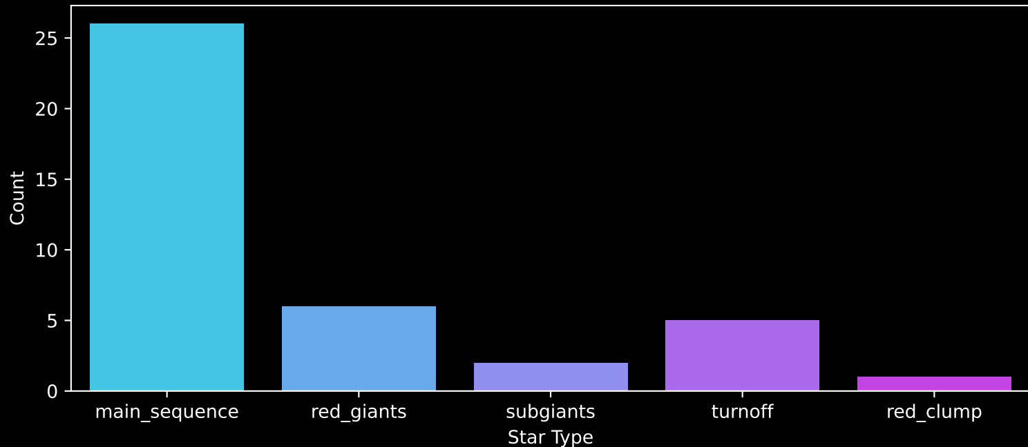
Gaia Stream: [NGC1851] Count plot of Star Type
