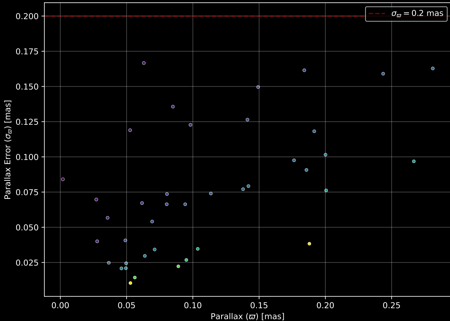
Gaia Stream: [NGC1851] Parallax Quality (n= 40)
