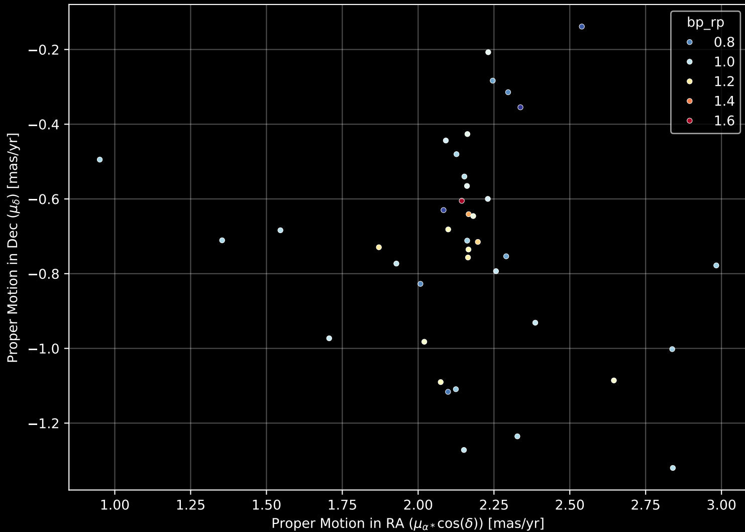
Gaia Stream: [NGC1851] Proper Motion Diagram (n= 40)
