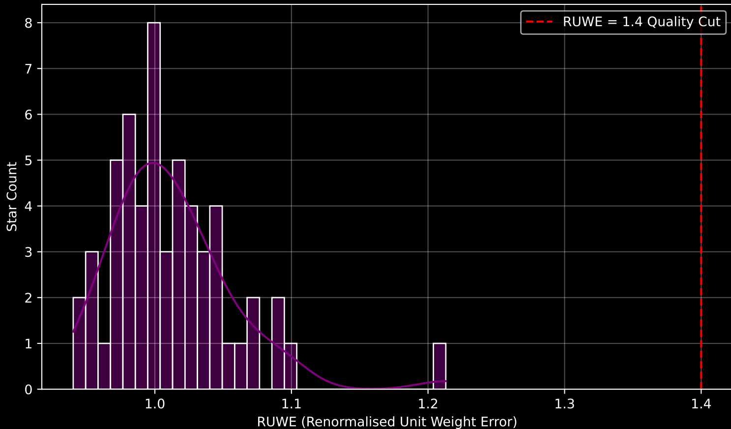
Gaia Stream: [NGC2298] RUWE Distribution (n= 56)
