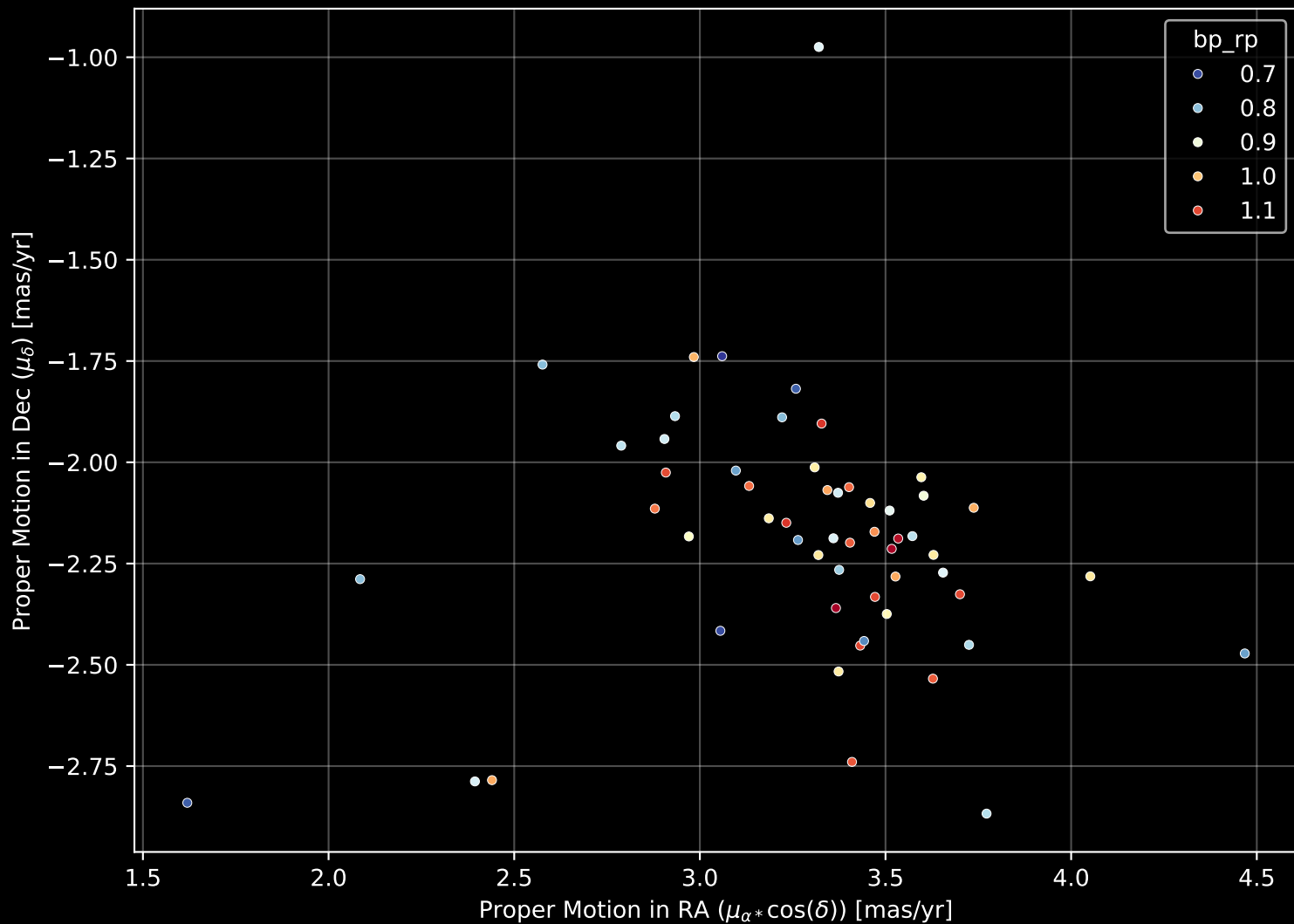
Gaia Stream: [NGC2298] Proper Motion Diagram (n= 56)
