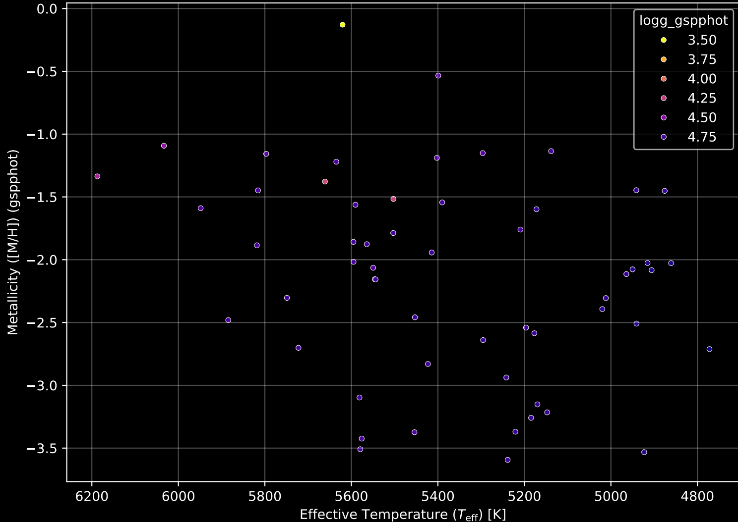
Gaia Stream: [NGC2298] Stellar Population Parameters (n= 56)
