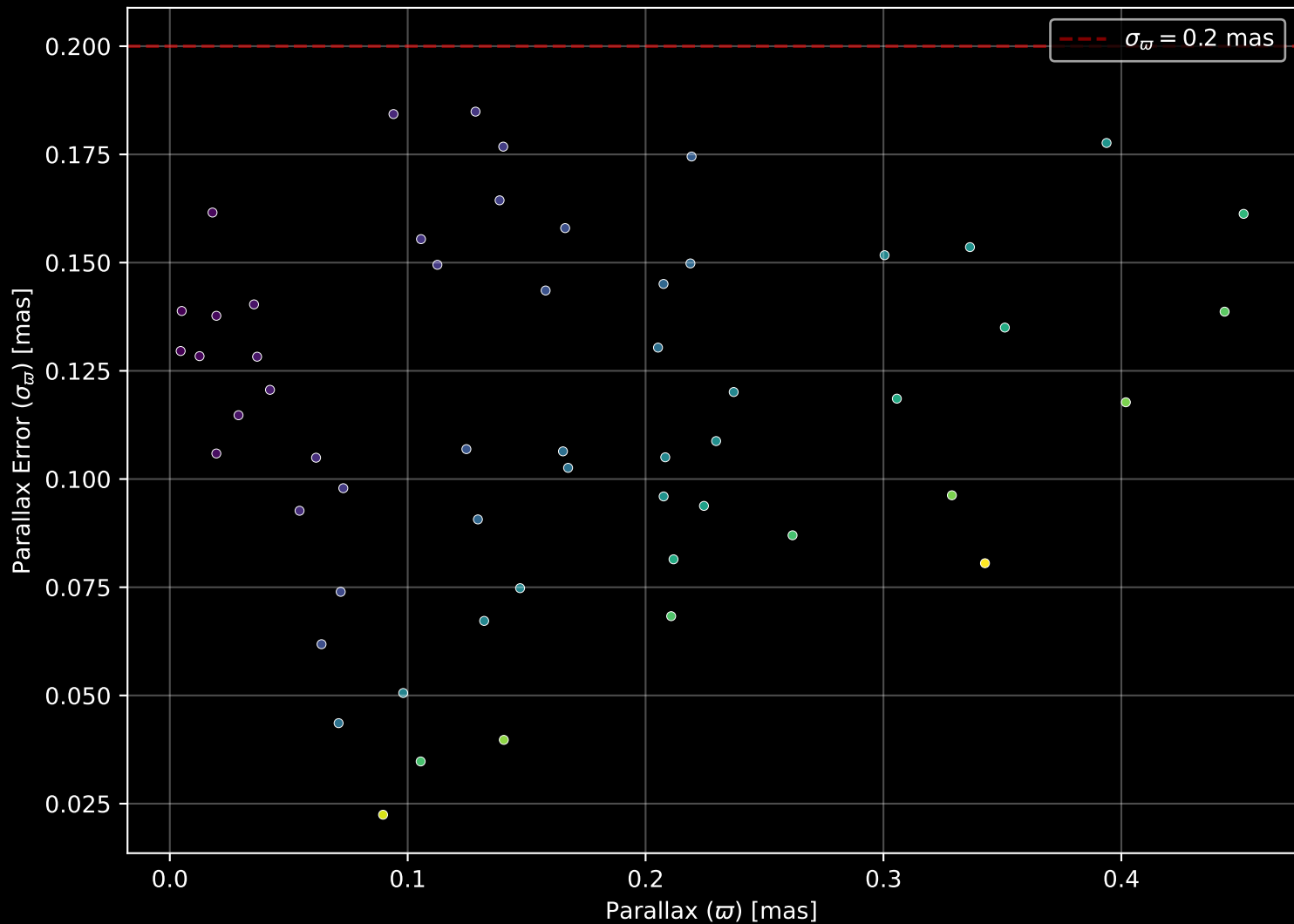
Gaia Stream: [NGC2298] Parallax Quality (n= 56)
