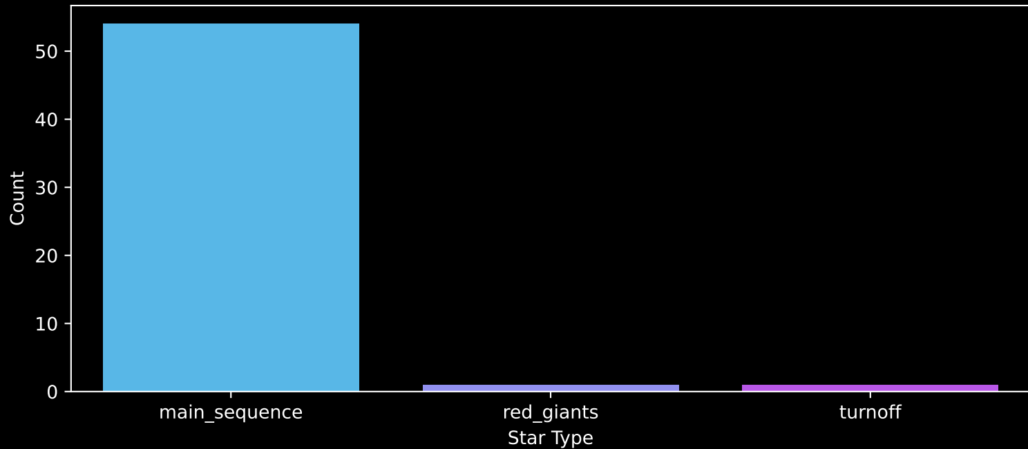
Gaia Stream: [NGC2298] Count plot of Star Type
