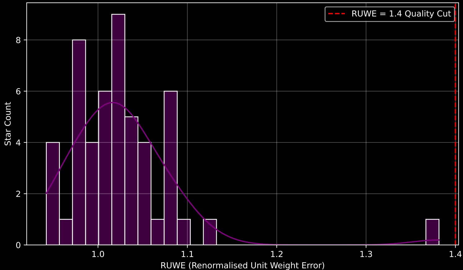
Gaia Stream: [NGC2808] RUWE Distribution (n= 51)
