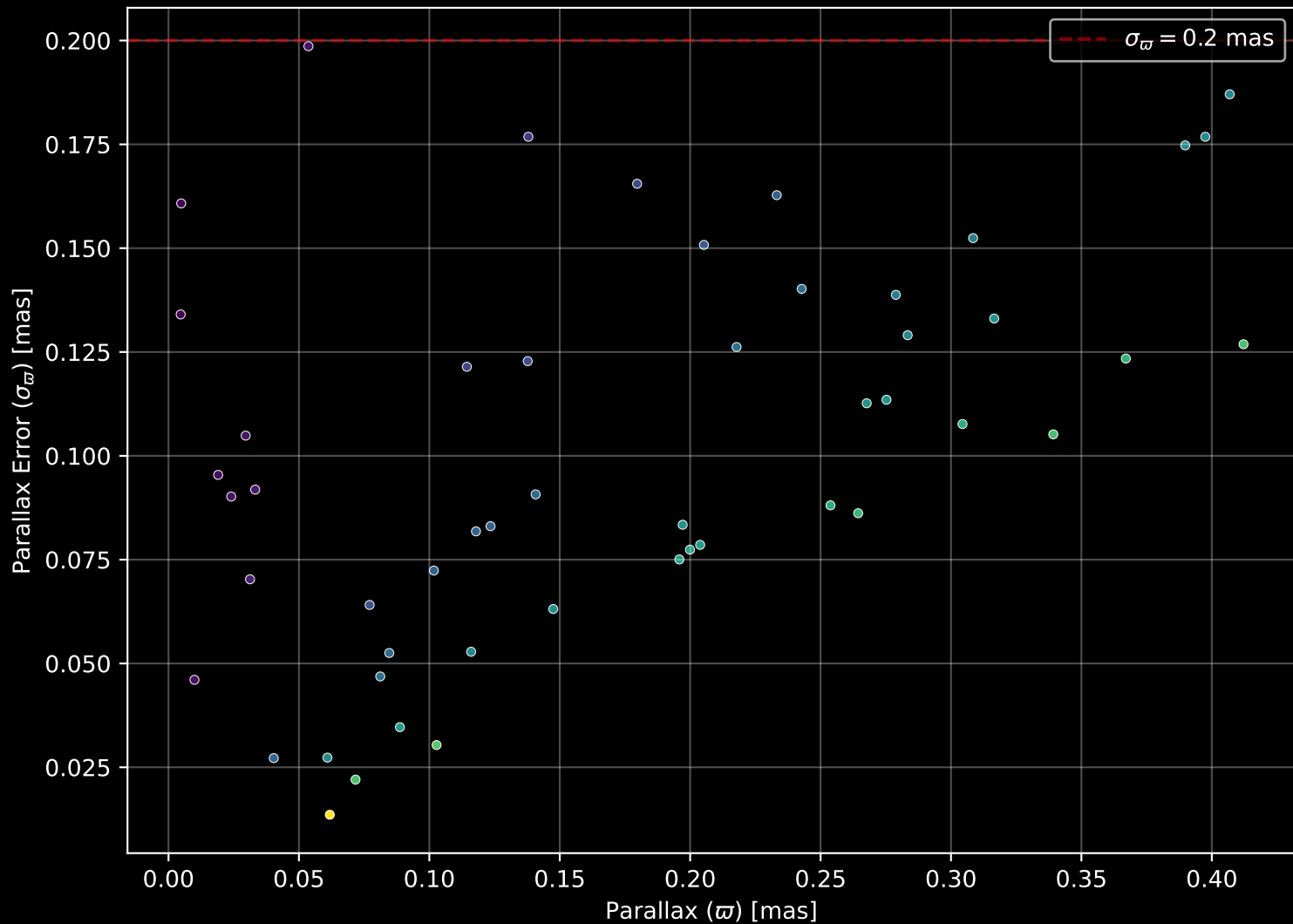
Gaia Stream: [NGC2808] Parallax Quality (n= 51)
