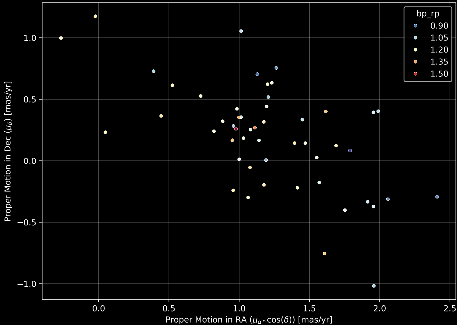
Gaia Stream: [NGC2808] Proper Motion Diagram (n= 51)
