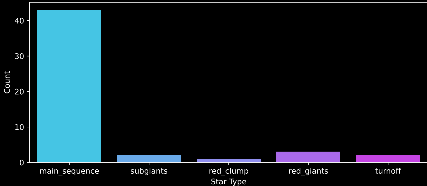
Gaia Stream: [NGC2808] Count plot of Star Type
