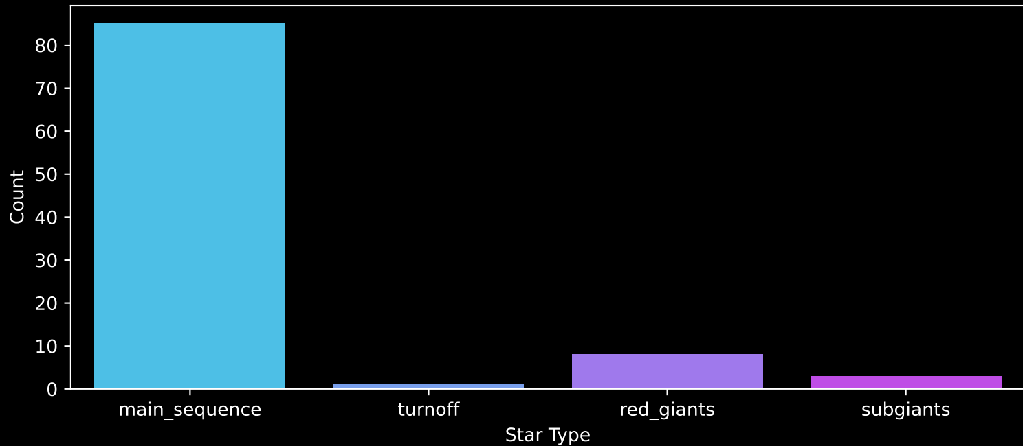
Gaia Stream: [NGC288] Count plot of Star Type
