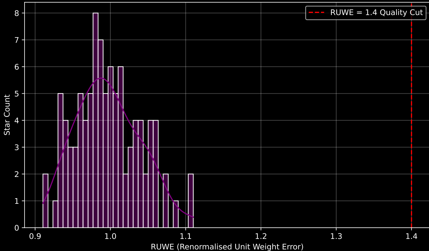
Gaia Stream: [NGC288] RUWE Distribution (n= 97)
