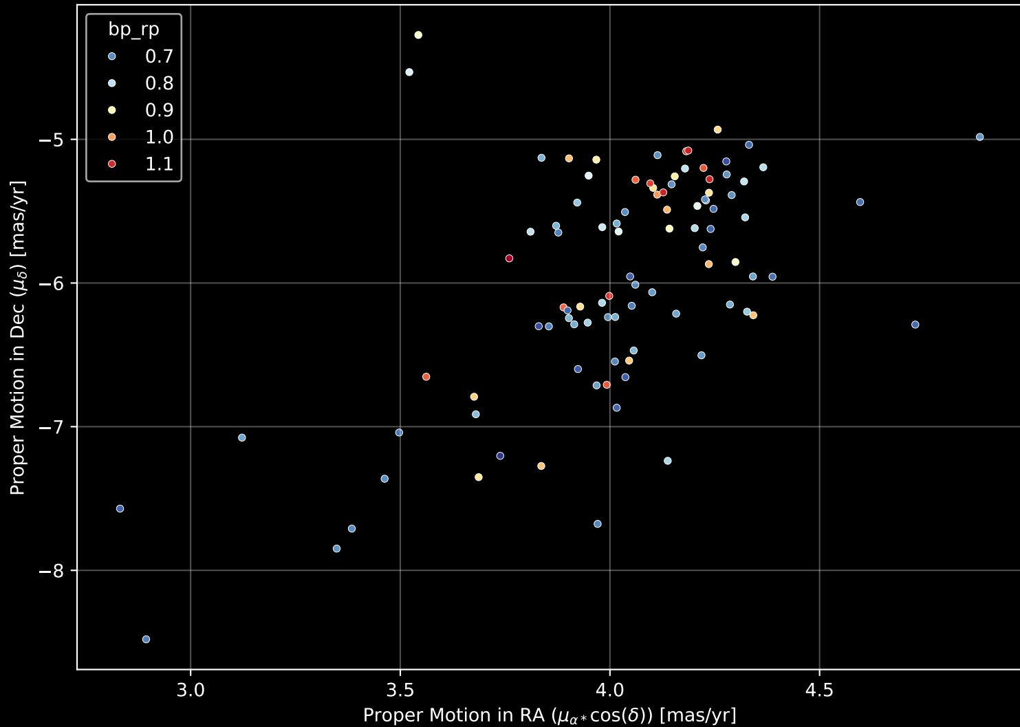
Gaia Stream: [NGC288] Proper Motion Diagram (n= 97)
