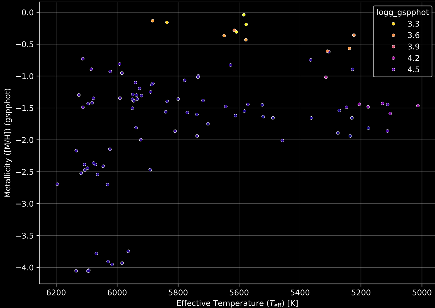
Gaia Stream: [NGC288] Stellar Population Parameters (n= 97)
