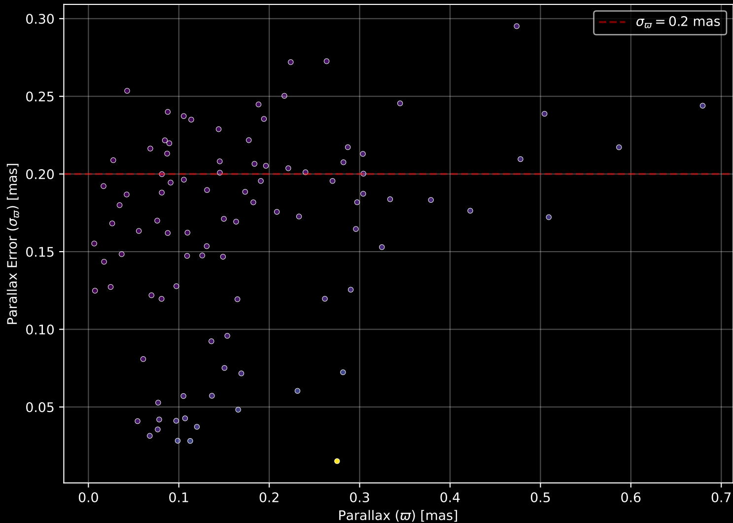
Gaia Stream: [NGC288] Parallax Quality (n= 97)
