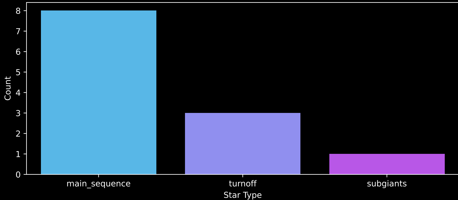
Gaia Stream: [NGC5466] Count plot of Star Type
