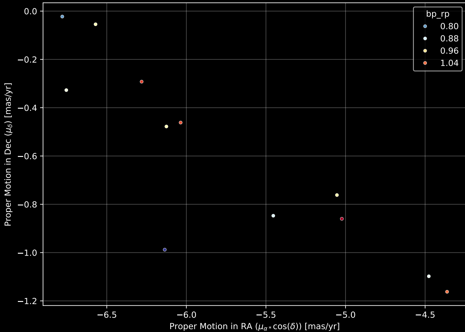
Gaia Stream: [NGC5466] Proper Motion Diagram (n= 12)
