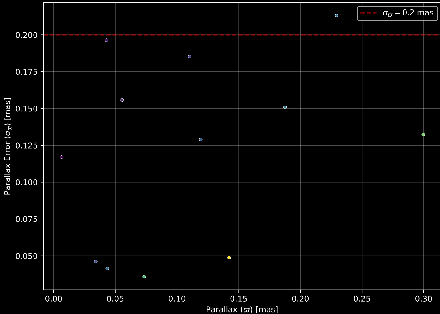
Gaia Stream: [NGC5466] Parallax Quality (n= 12)
