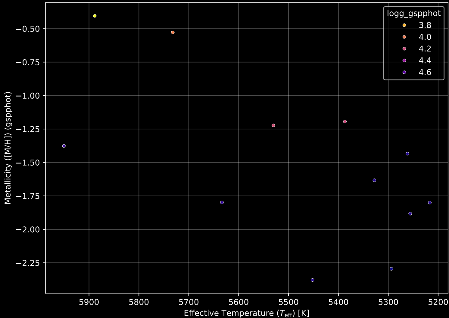
Gaia Stream: [NGC5466] Stellar Population Parameters (n= 12)
