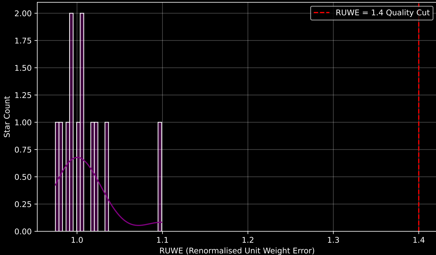
Gaia Stream: [NGC5466] RUWE Distribution (n= 12)
