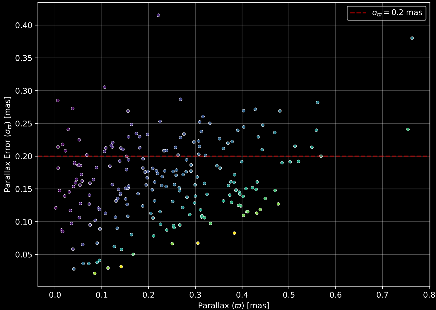
Gaia Stream: [NGC6101] Parallax Quality (n= 218)
