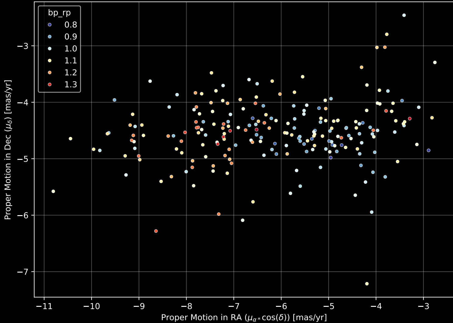
Gaia Stream: [NGC6101] Proper Motion Diagram (n= 218)
