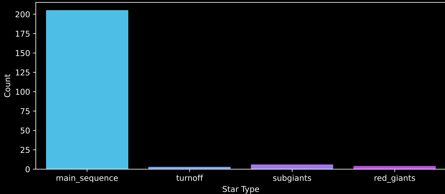
Gaia Stream: [NGC6101] Count plot of Star Type
