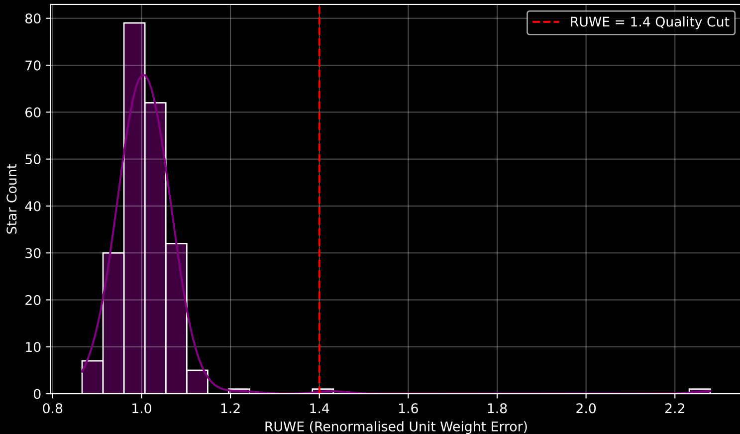
Gaia Stream: [NGC6101] RUWE Distribution (n= 218)
