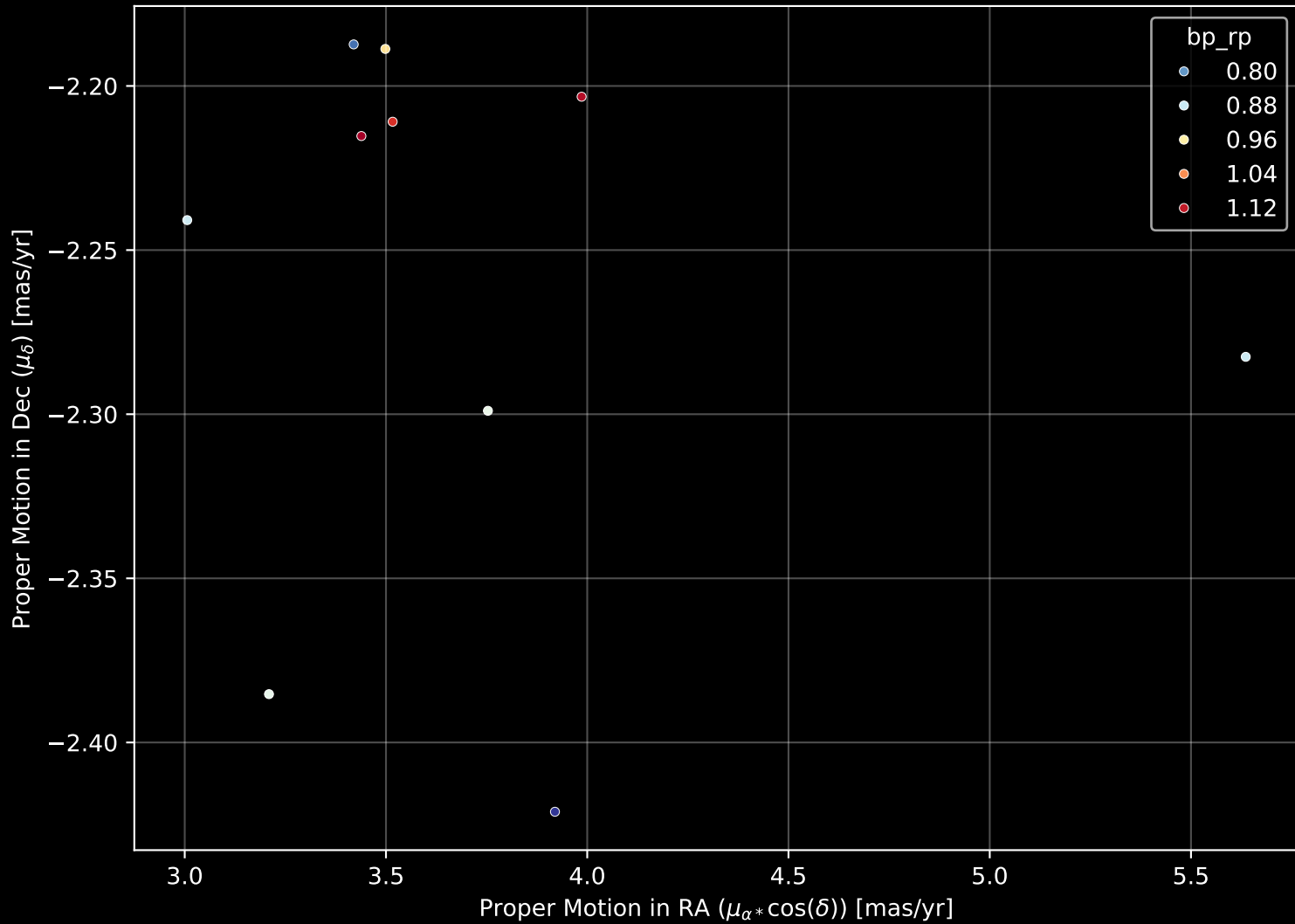
Gaia Stream: [NGC7089] Proper Motion Diagram (n= 10)
