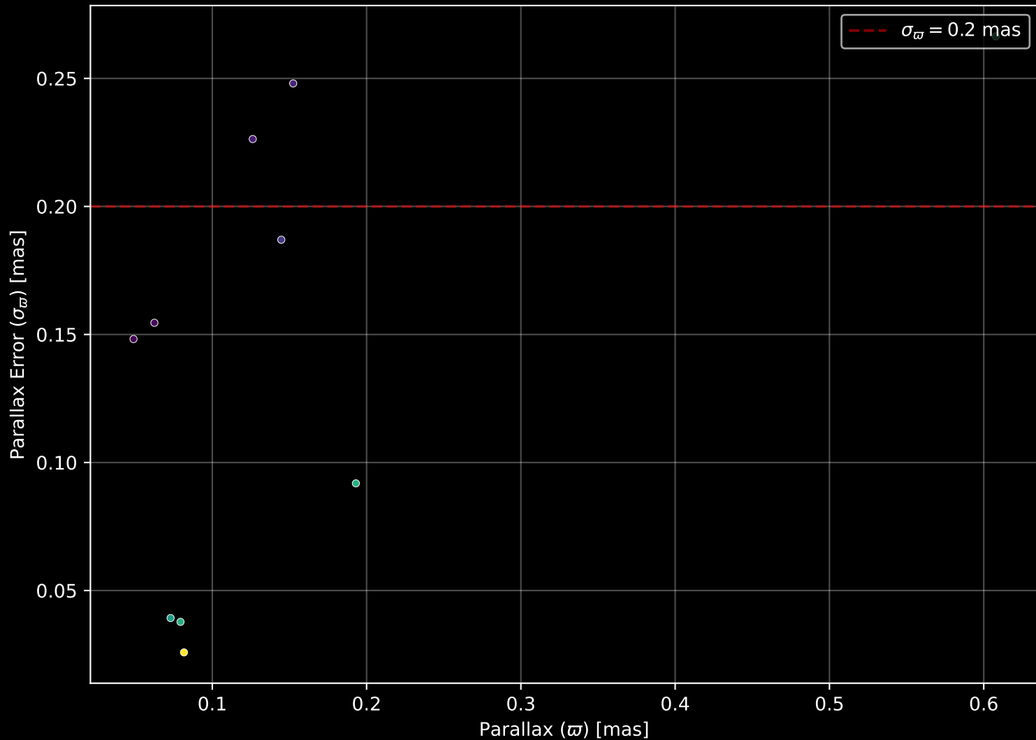
Gaia Stream: [NGC7089] Parallax Quality (n= 10)
