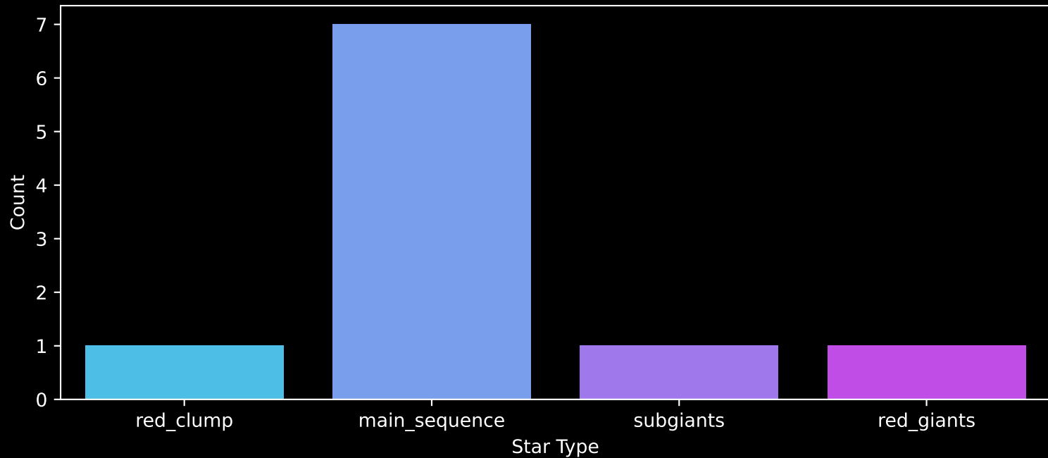
Gaia Stream: [NGC7089] Count plot of Star Type
