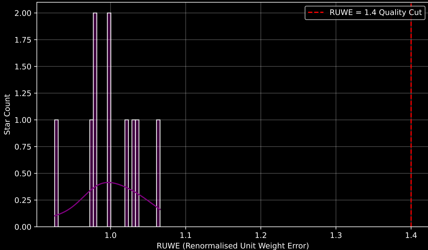
Gaia Stream: [NGC7089] RUWE Distribution (n= 10)
