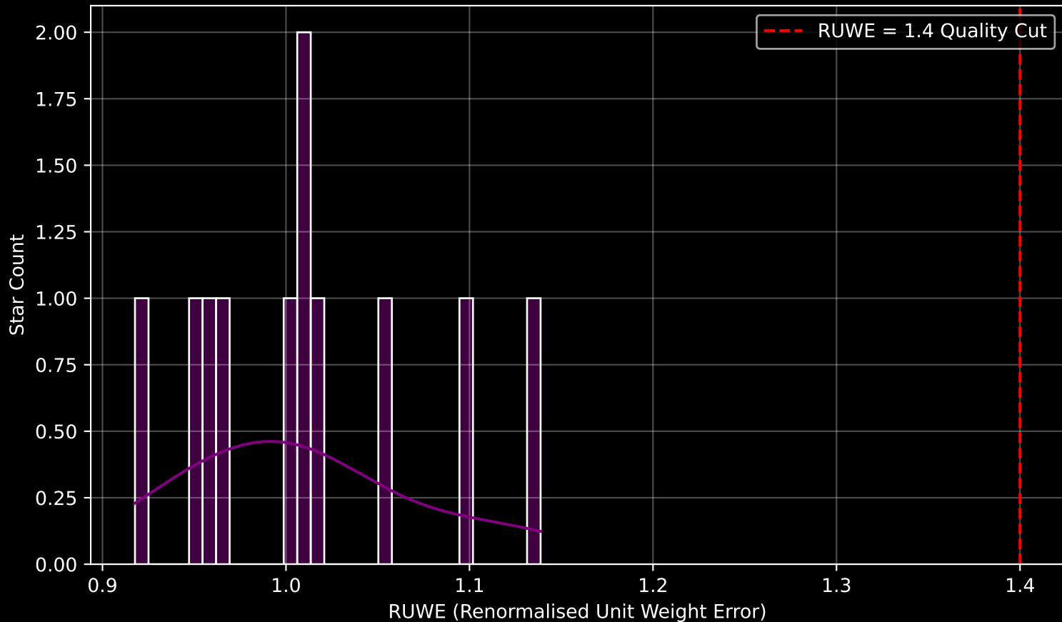
Gaia Stream: [NGC7492] RUWE Distribution (n= 11)
