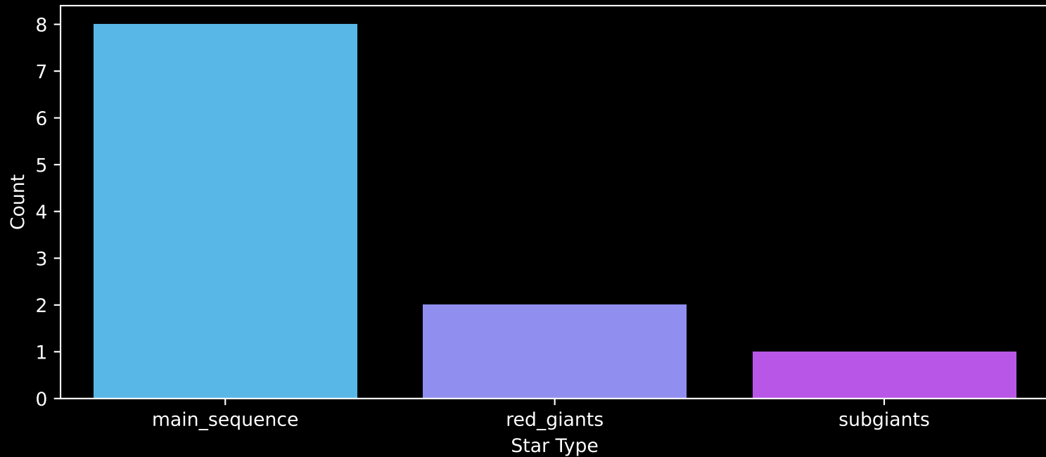
Gaia Stream: [NGC7492] Count plot of Star Type
