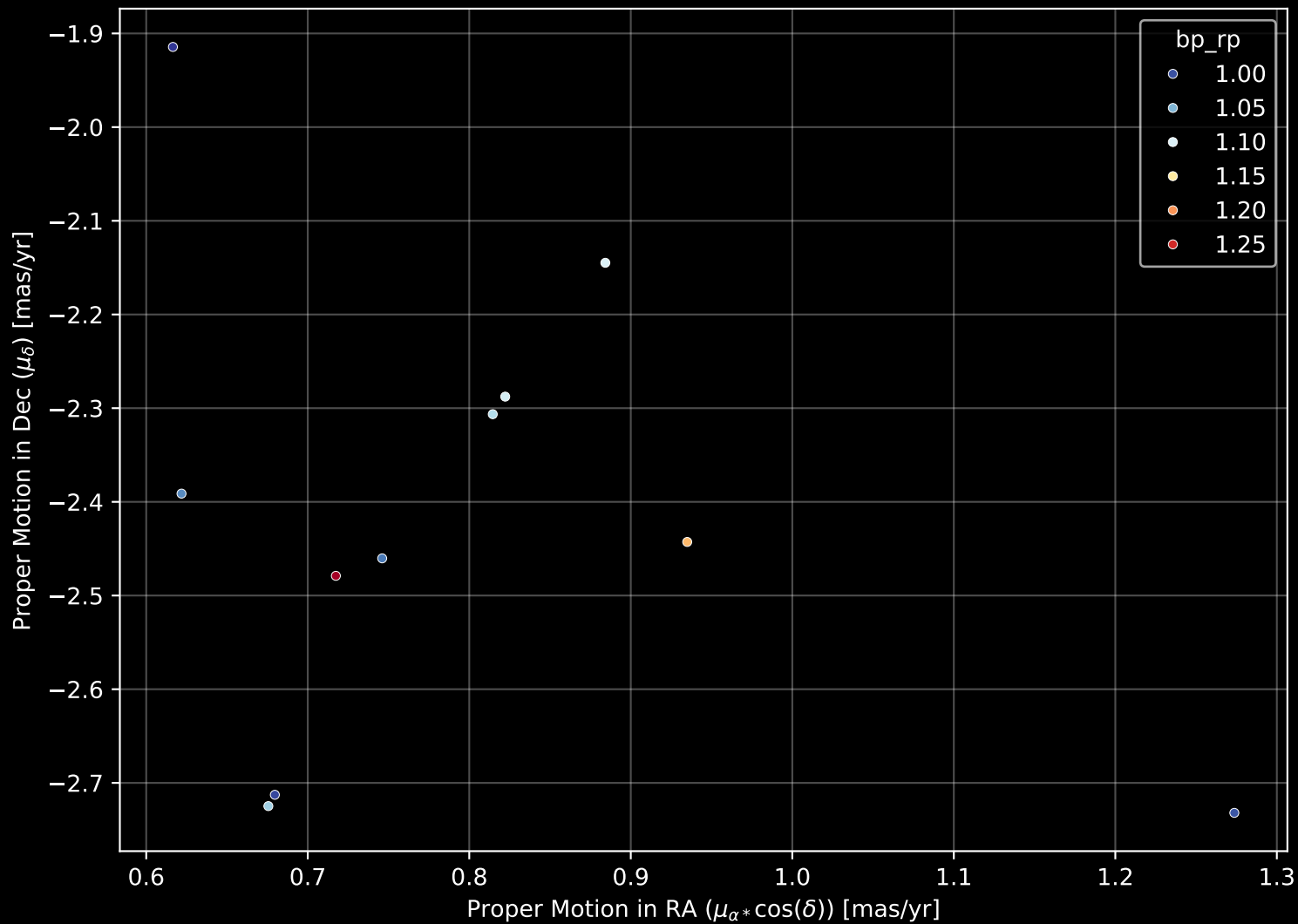
Gaia Stream: [NGC7492] Proper Motion Diagram (n= 11)
