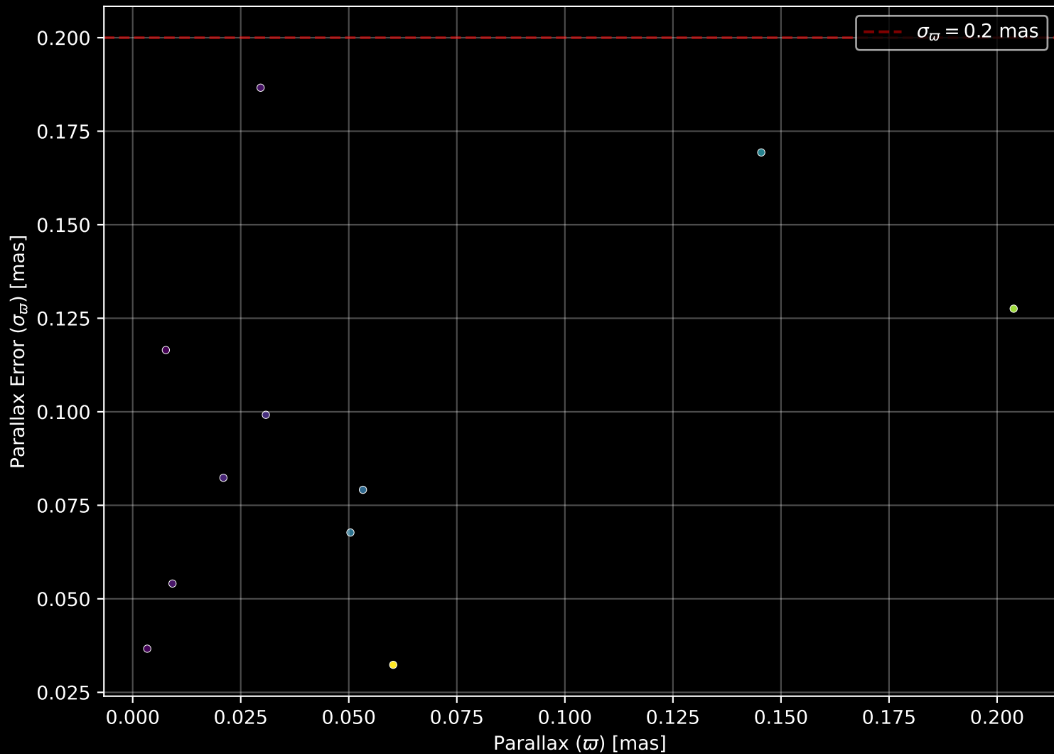
Gaia Stream: [NGC7492] Parallax Quality (n= 11)
