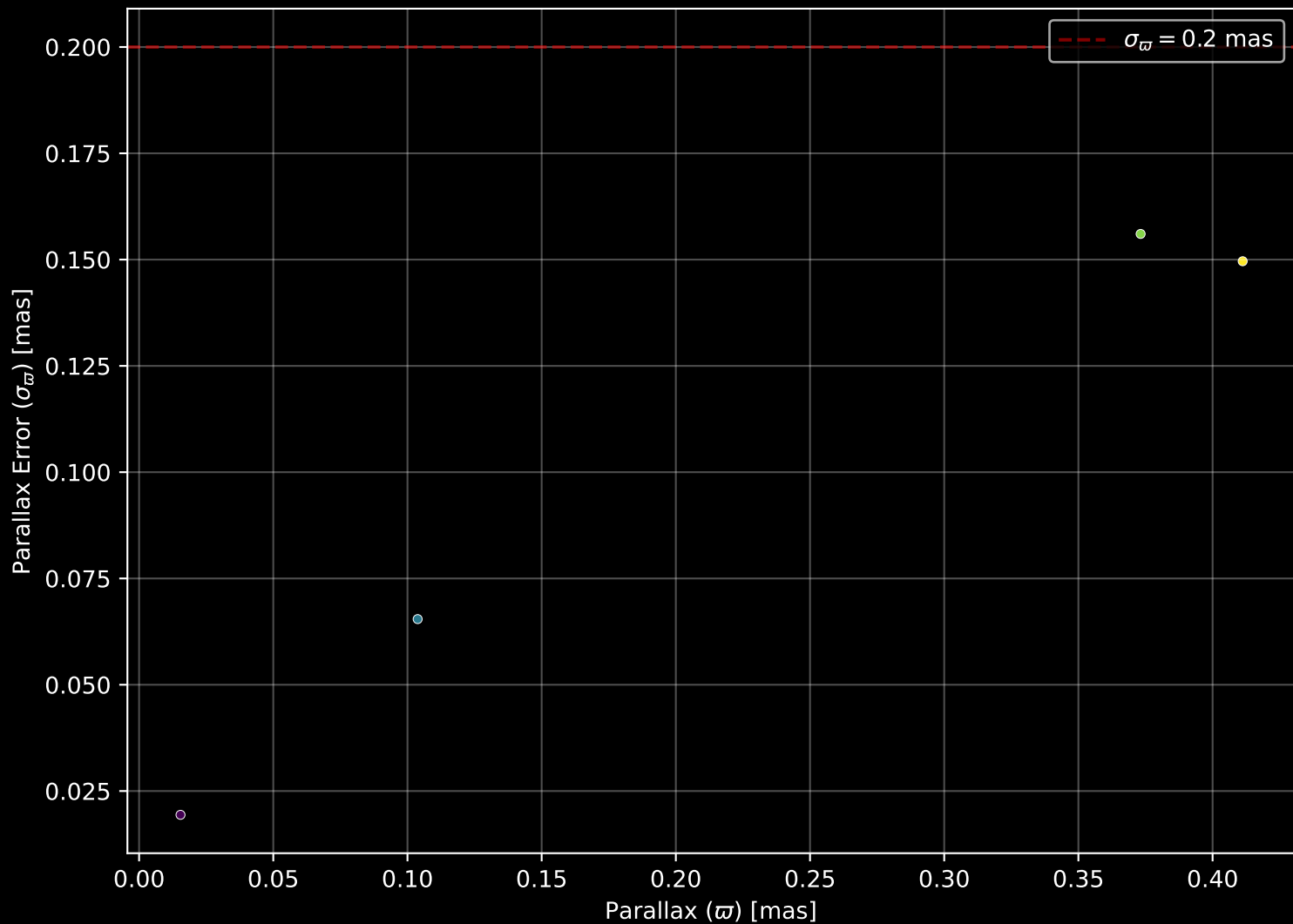
Gaia Stream: [New-1] Parallax Quality (n= 4)
