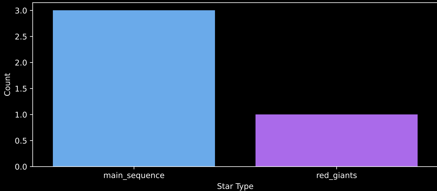
Gaia Stream: [New-1] Count plot of Star Type
