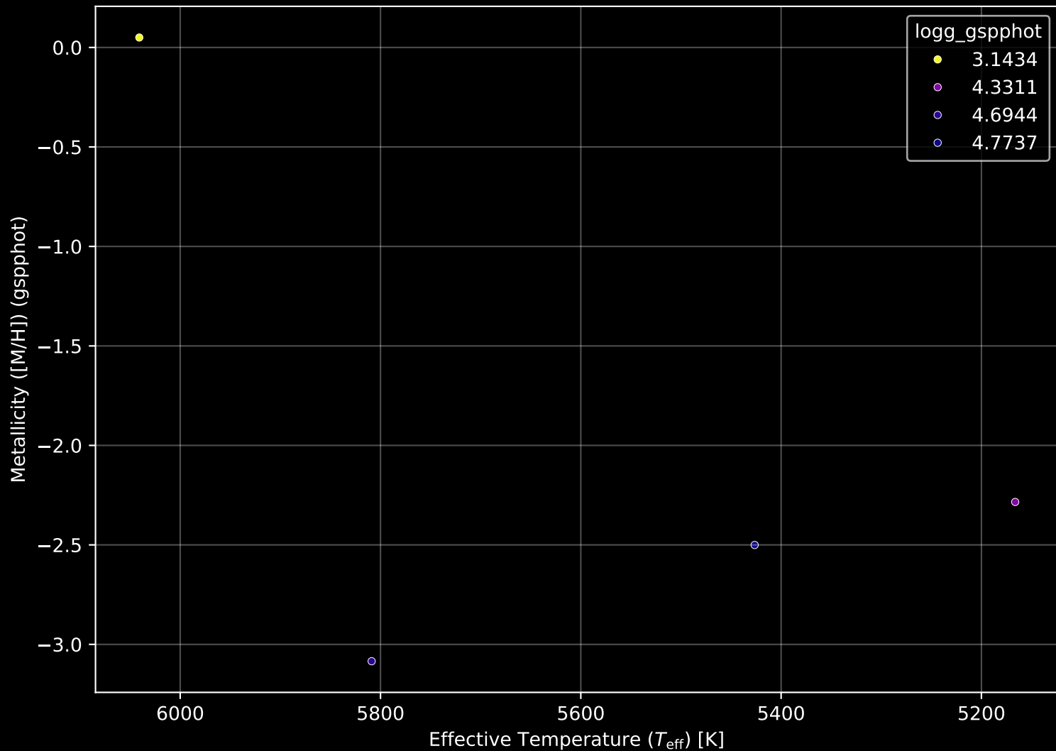
Gaia Stream: [New-1] Stellar Population Parameters (n= 4)
