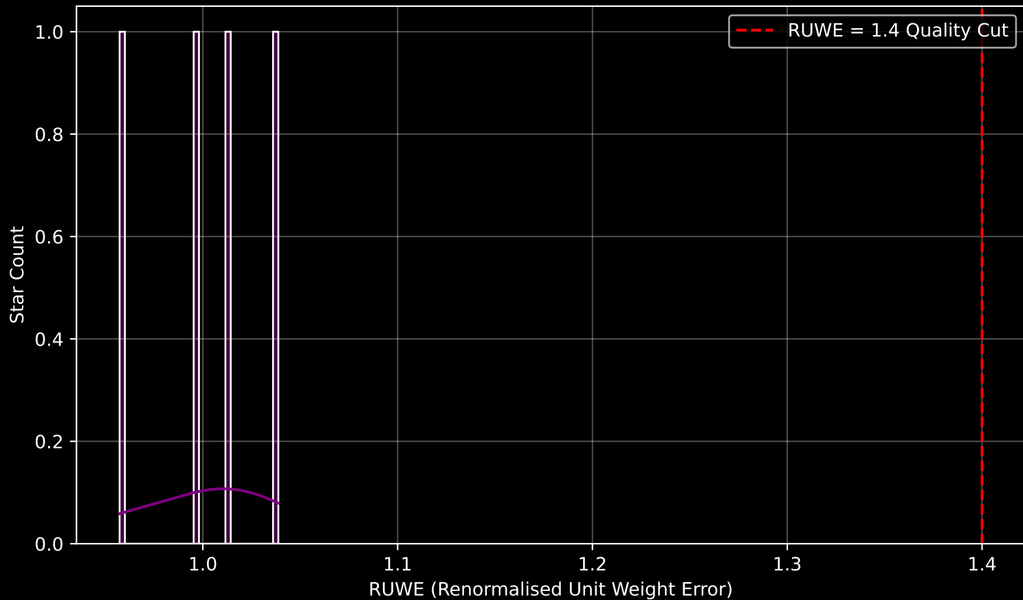
Gaia Stream: [New-1] RUWE Distribution (n= 4)
