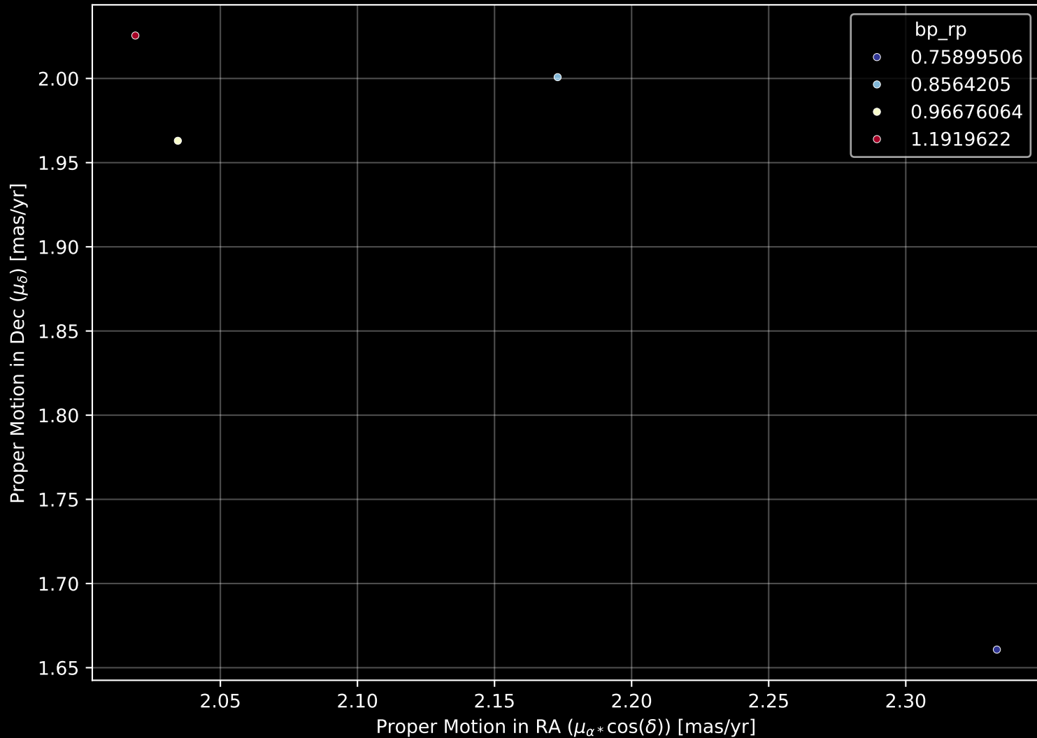
Gaia Stream: [New-1] Proper Motion Diagram (n= 4)
