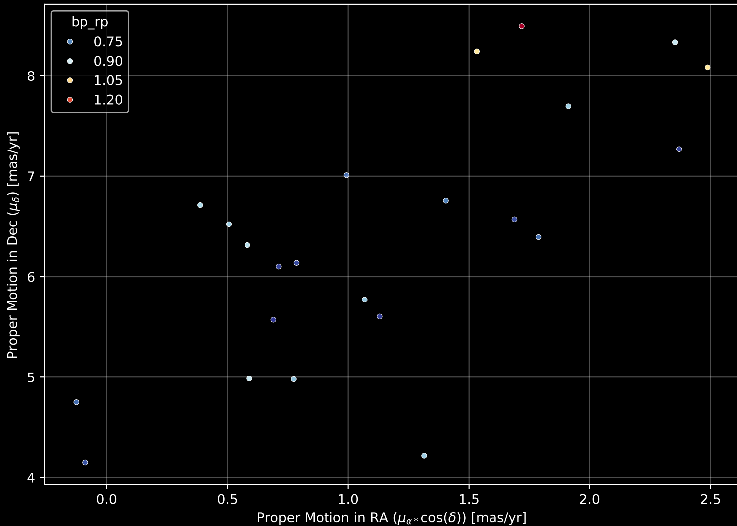
Gaia Stream: [New-12] Proper Motion Diagram (n= 23)
