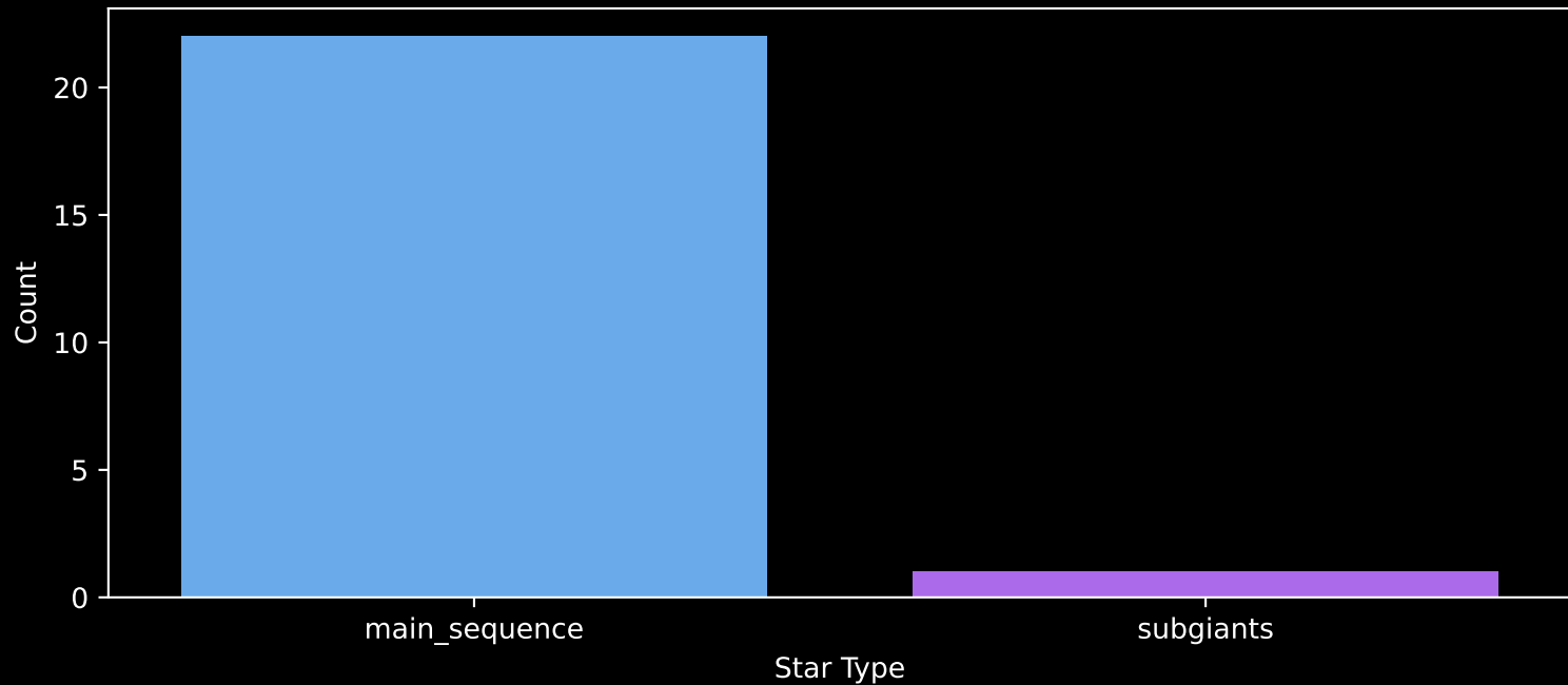
Gaia Stream: [New-12] Count plot of Star Type
