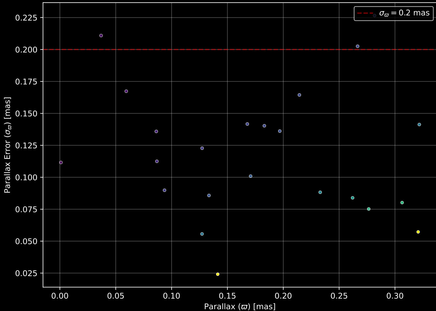
Gaia Stream: [New-12] Parallax Quality (n= 23)
