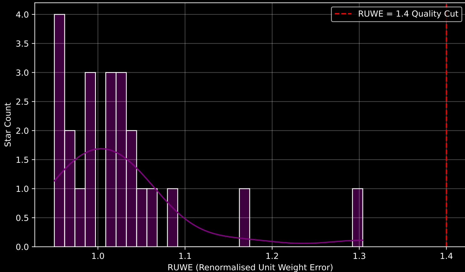
Gaia Stream: [New-12] RUWE Distribution (n= 23)
