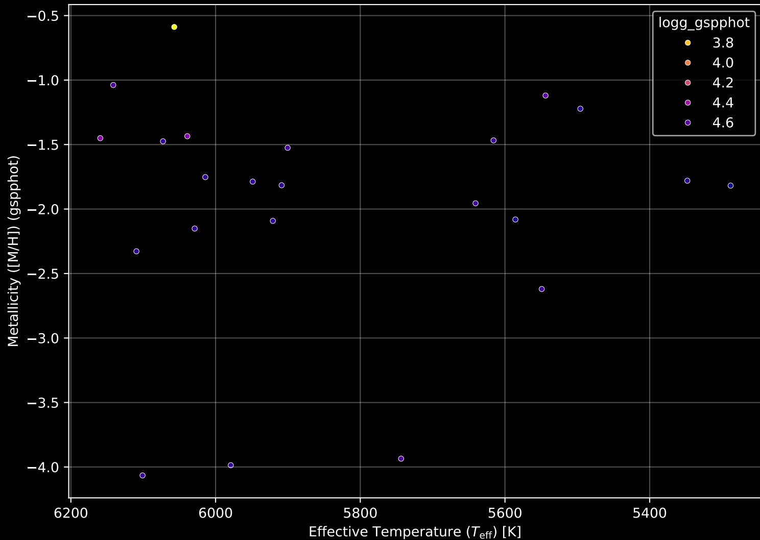
Gaia Stream: [New-12] Stellar Population Parameters (n= 23)
