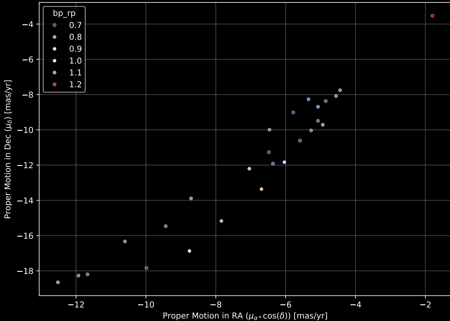
Gaia Stream: [New-13] Proper Motion Diagram (n= 26)
