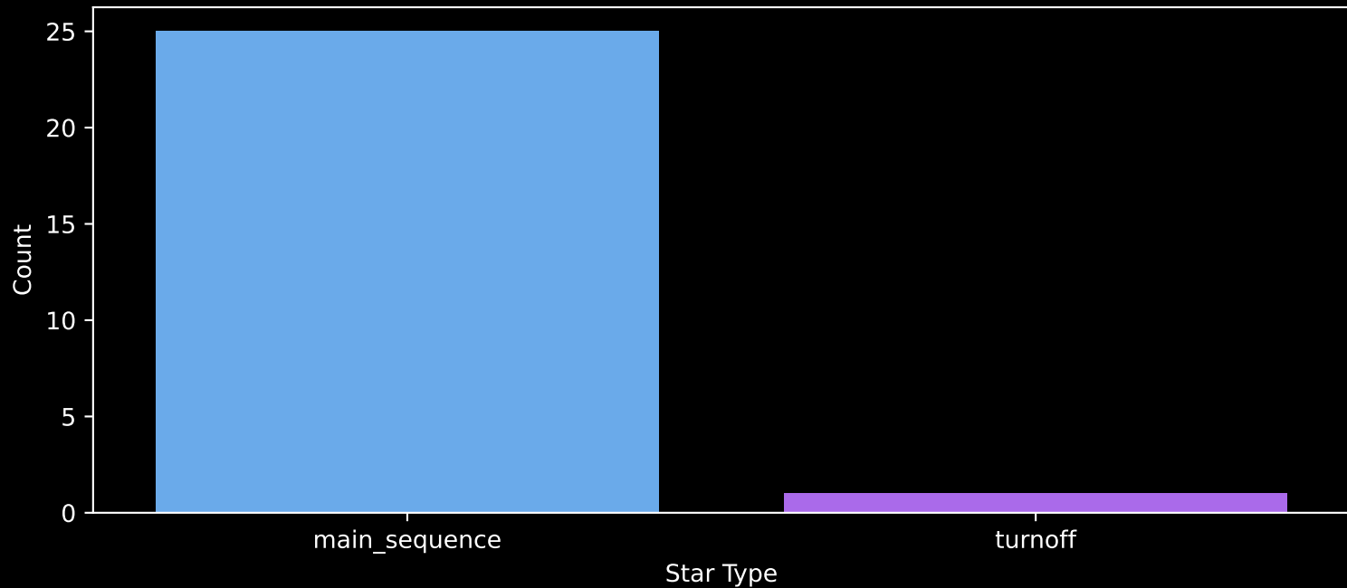
Gaia Stream: [New-13] Count plot of Star Type
