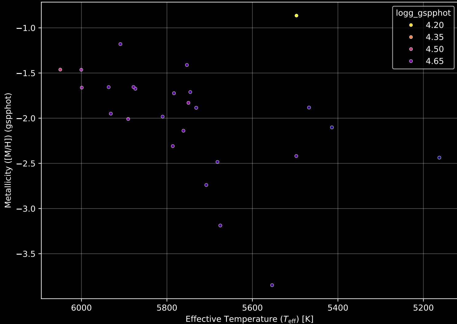
Gaia Stream: [New-13] Stellar Population Parameters (n= 26)
