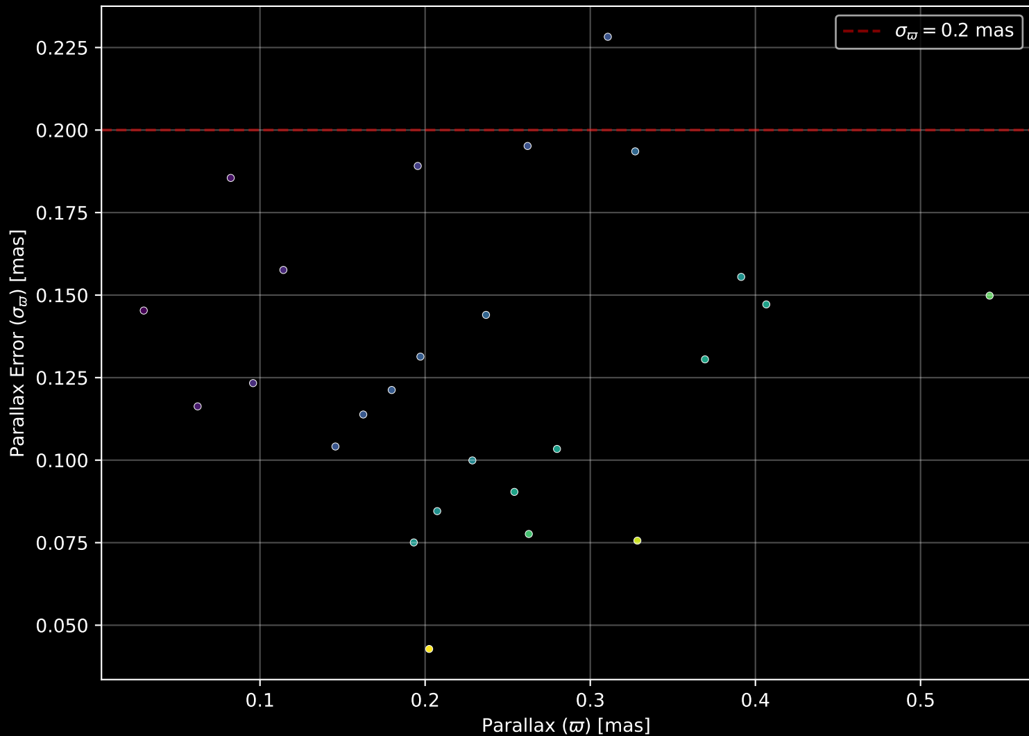
Gaia Stream: [New-13] Parallax Quality (n= 26)
