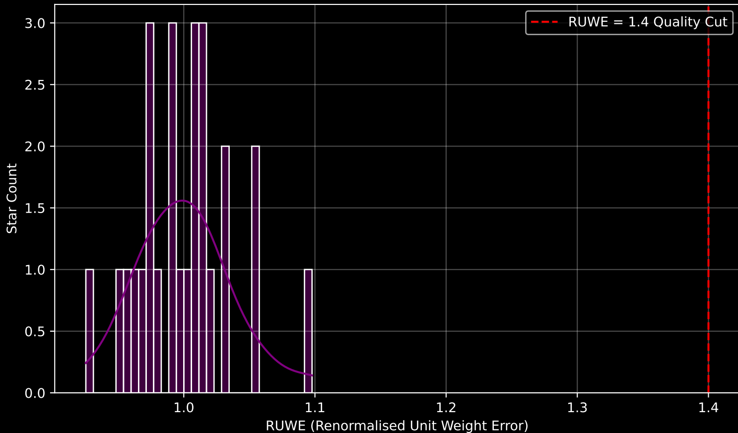
Gaia Stream: [New-13] RUWE Distribution (n= 26)
